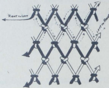
FIG. 1 - FISH NETTING
