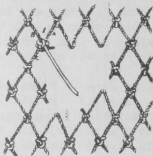
STARTER KNOT
