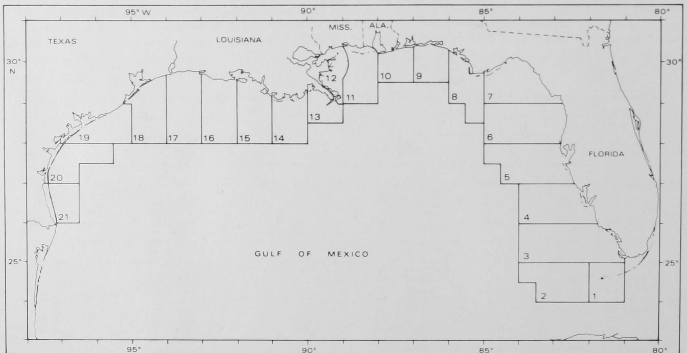
Figure 1.—Statistical subareas used in reporting Gulf Coast Shrimp Data (after Kutkuhn, 1962).
