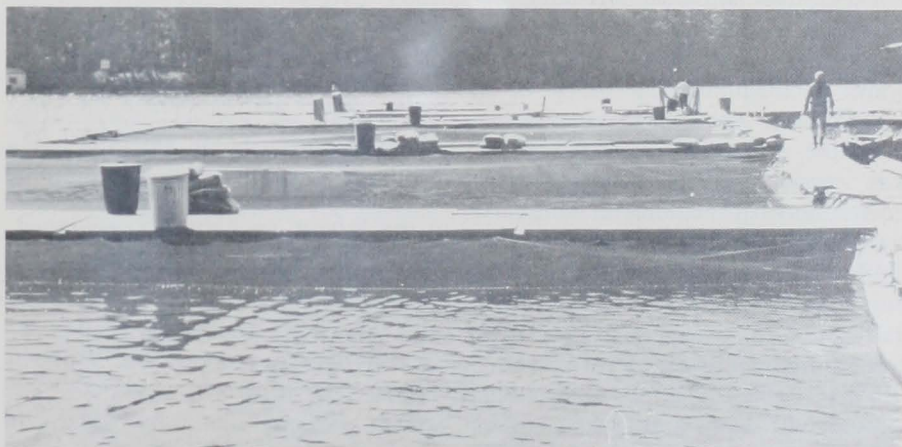
Figure 7.—Salmon-rearing pens located at Squaxin Island, Washington. (Photo by J. Frazer, STOWW.)
