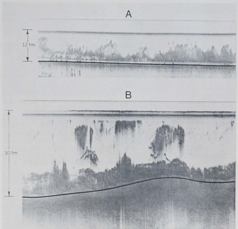
Figure 10.—Daytime traces of pelagic red crabs on a "white line" Fathometer. A: Bahia Magdalena. Crabs on and near bottom. The inverted "V" traces were probably fish. B: Thetis Bank. Crabs on the bottom as well as near the surface. The "white line" is occluded because of the density of the crabs.
