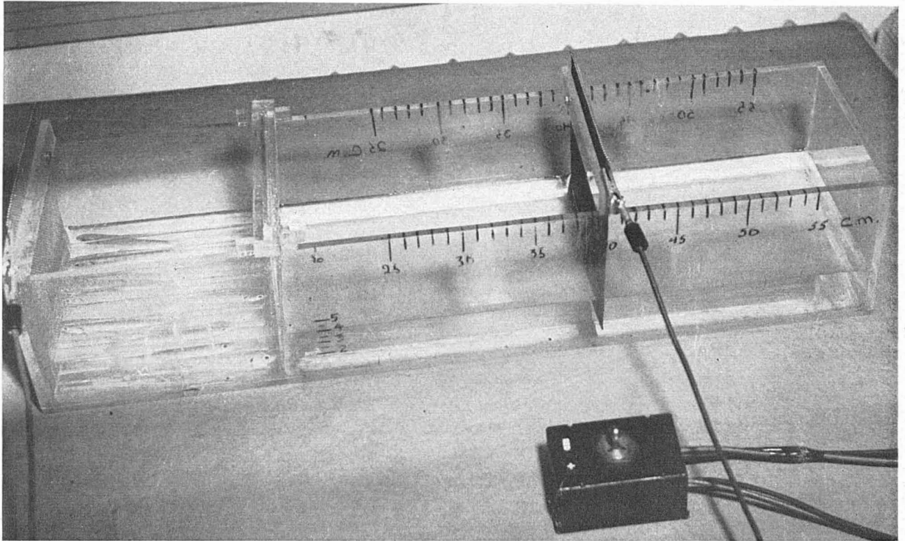
FIGURE 1.—Experimental tank, 60 cm. x 15 cm. x 11 cm.
