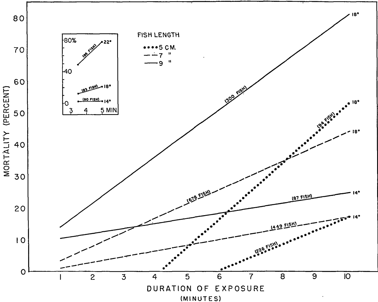
FIGURE 14.—Effect of duration of exposure in relation to temperature and fish length upon mortality of salmon fingerlings ( Oncorhynchus tshawytscha ) exposed to pulsating d. c. Tests run at 4 volts/cm., current density range 0.14 to 0.27 milliamps./cm. 2 , 2 pulses/sec., pulse duration 20 milliseconds. (Insert: tests run at 2 volts/cm., current density range 0.09 to 0.11 milliamps./cm. 2 , 2 pulses/sec., pulse duration 20 milliseconds., fish length 9 cm.)
