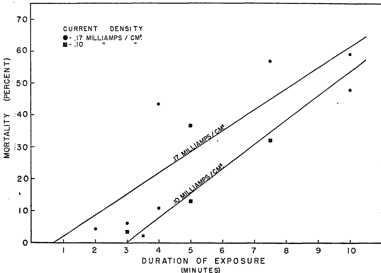
FIGURE 9.—Effect of duration of exposure in relation to current density upon mortality of salmon fingerlings ( Oncorhynchus tshawytscha ) exposed to pulsating d. c. Tests run at 2 volts/cm., 2 pulses/sec., pulse duration 20 milliseconds, temperature range 10.0° to 19.9° C., fish length cm. Sizes of symbols correspond to fish number categories: 16–49 and 50–65.
