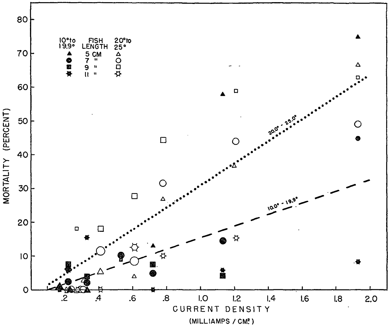
FIGURE 5.—Effect of current density in relation to fish length and water temperature upon mortality of salmon fingerlings ( Oncorhynchus tshawytscha ) exposed to pulsating d. c. Tests run at 4 volts/cm., 2 pulses/sec., pulse duration 20 milli-sec., duration of exposure 30 seconds. Sizes of symbols correspond to fish number categories: 23-74, 75-149, and 150-443.
