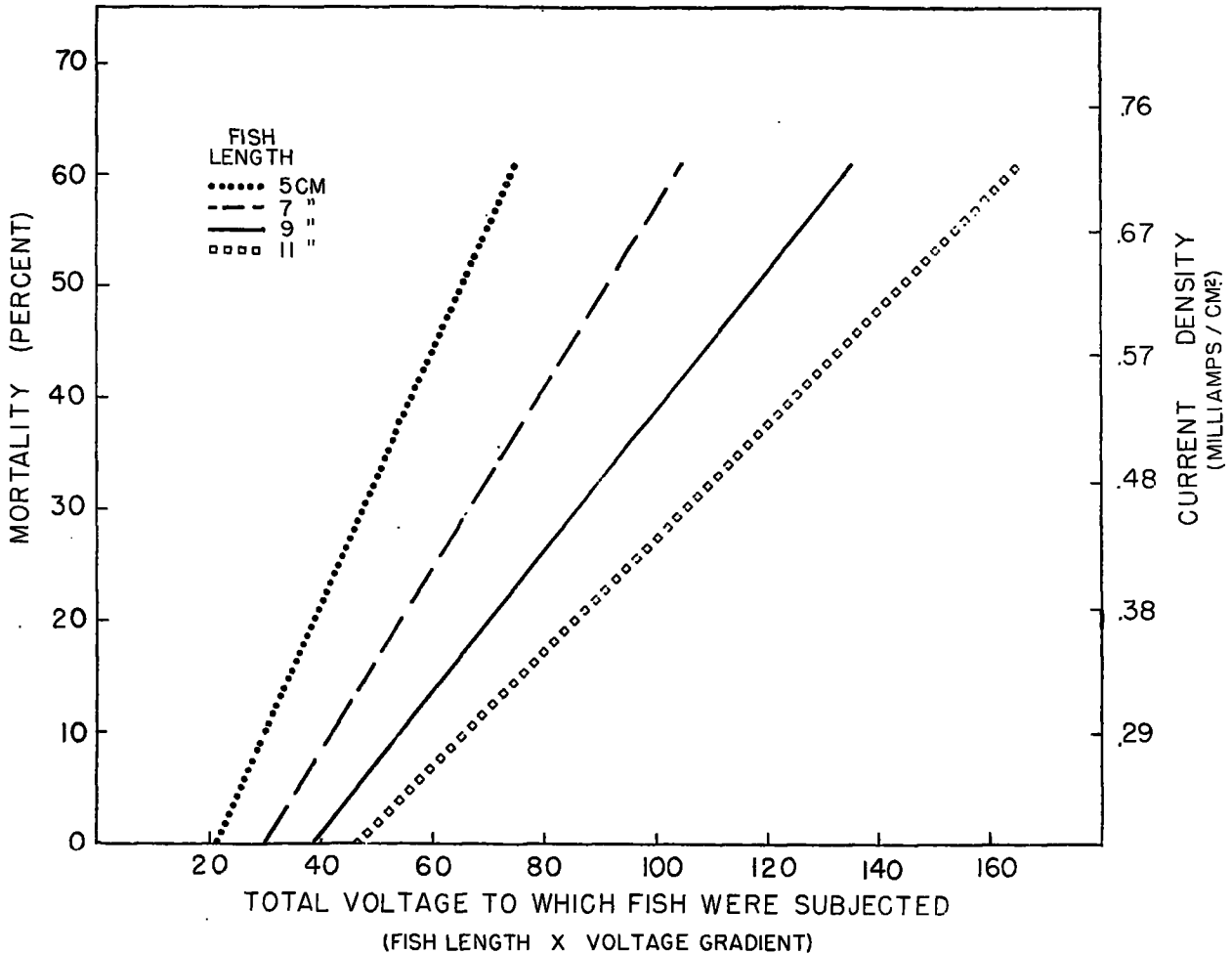
FIGURE 7.—Effect of the total voltage to which the fish were subjected in relation to fish length and current density upon mortality of salmon fingerlings ( Oncorhynchus tshawytscha ) exposed to pulsating d. c. (fig. 4 replotted in terms of the total voltage to which fish were subjected).
