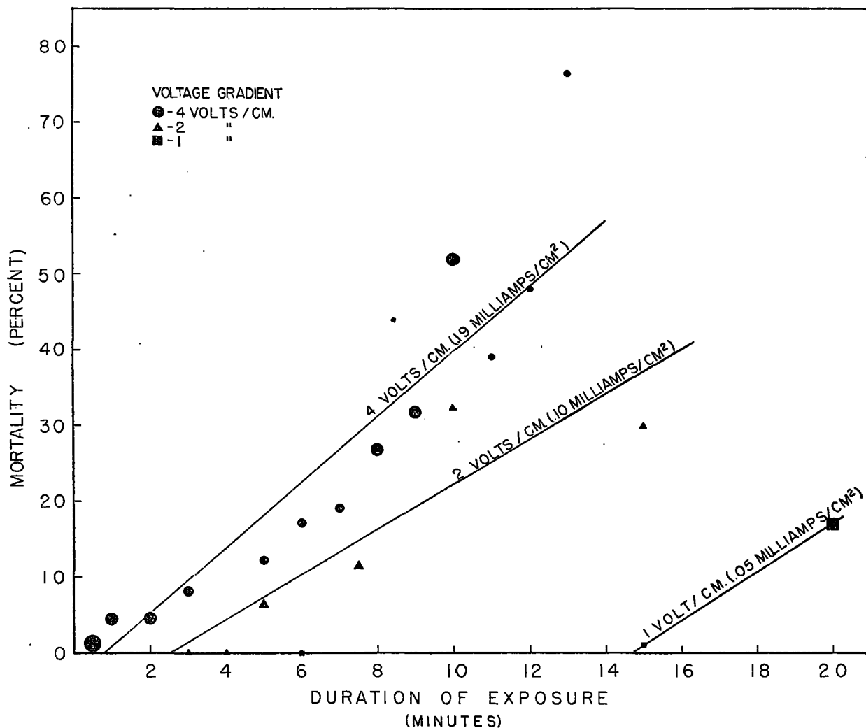
FIGURE 8.—Effect of duration of exposure in relation to the combined effects of voltage gradient and current density upon mortality of salmon fingerlings ( Oncorhynchus tshawytscha ) exposed to pulsating d. c. Tests run at 2 pulses/sec., pulse duration 20 millisees., temperature 10.0° to 19.9° C., fish length 7 cm. Sizes of symbols correspond to fish number categories: 17-49, 50-99, 100-199 and 200-241.
