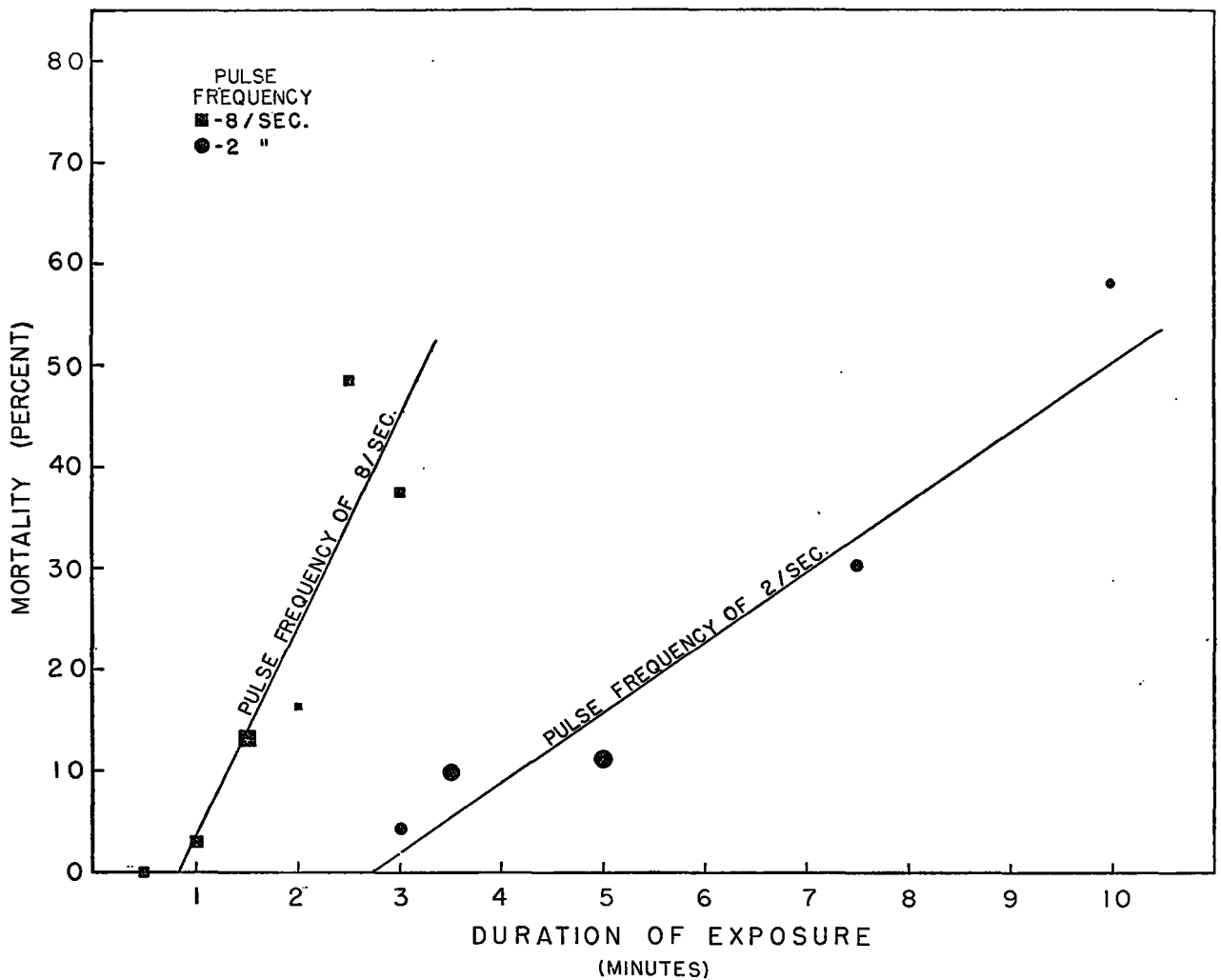
FIGURE 11.—Effect of duration of exposure in relation to pulse frequency upon mortality of salmon fingerlings ( Oncorhynchus tshawytscha ) exposed to pulsating d. c. Tests run at 2 volts/cm., current density range 0.08 to 0.13 milliamps./cm. 2 , pulse duration 20 millisees., temperature range 12.0° to 19.9° C., fish length 9 cm. Sizes of symbols correspond to fish number categories: 27-49, 50-99, and 100-111.
