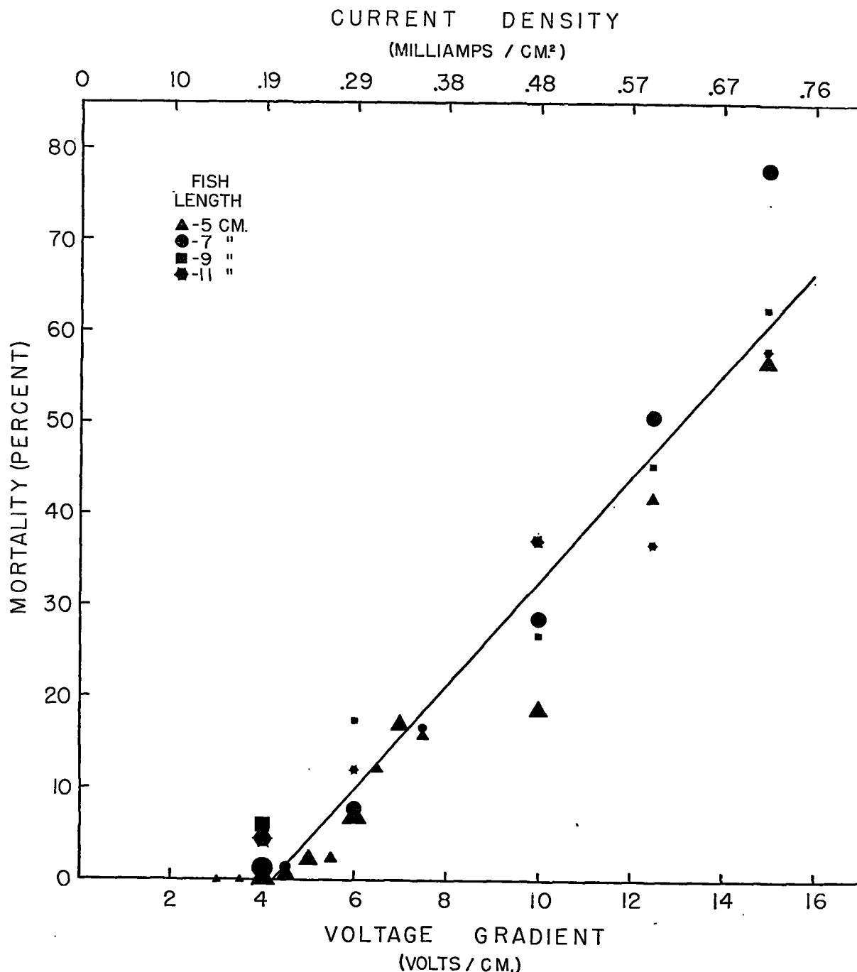
FIGURE 4.—Combined effects of voltage gradient and current density in relation to fish length upon mortality of salmon fingerlings ( Oncorhynchus tshawytscha ) exposed to pulsating d. c. Tests run at 2 pulses/sec., pulse duration 20 milli-secs., temperature range 10.0° to 19.9° C., duration of exposure 30 seconds. Sizes of symbols correspond to fish number categories: 10-49, 50-99, 100-199, and 200-227.
