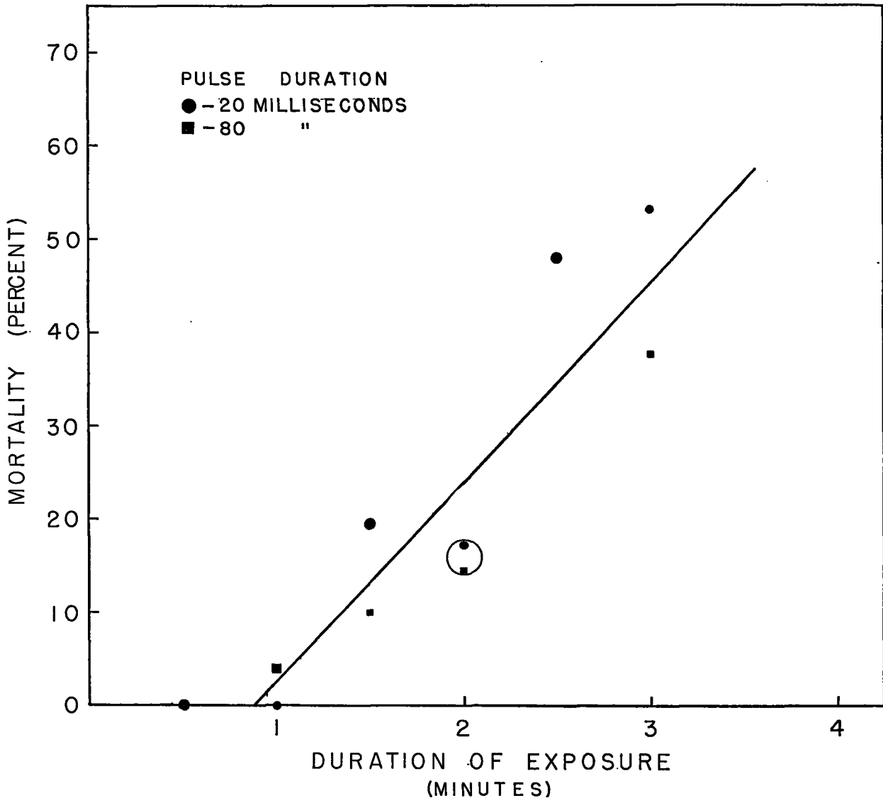
FIGURE 12.—Effect of duration of exposure in relation to pulse duration upon mortality of salmon fingerlings ( Oncorhynchus tshawytscha ) exposed to pulsating d.c. Tests run at 2 volts/cm., current density 0.10 milliamps./cm. 2 , 8 pulses/sec., temperature range 10.0° to 16.0° C., fish length 9 cm. For explanation of circled data see text. Sizes of symbols correspond to fish number categories: 14-49 and 50-58.
