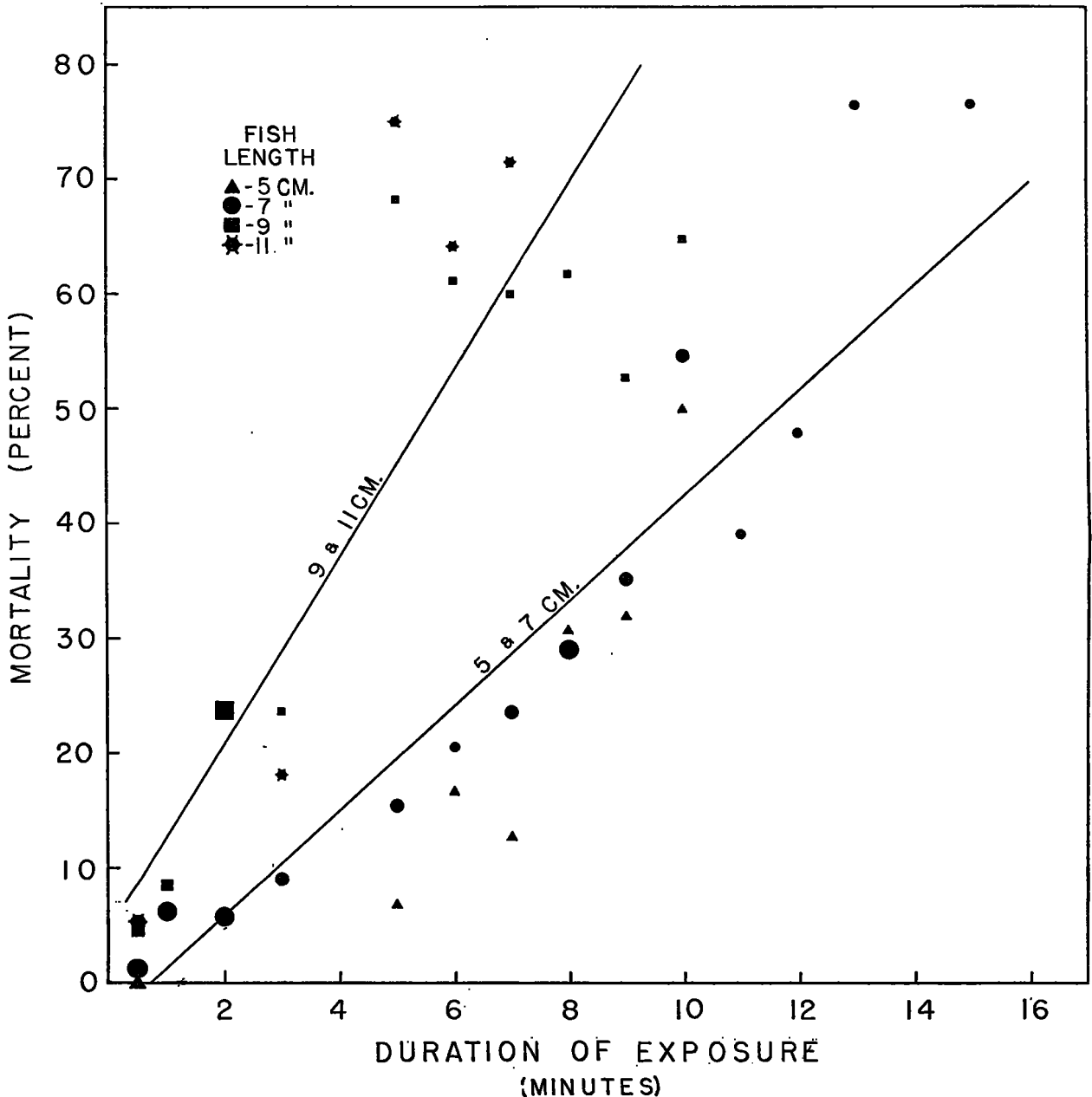
FIGURE 13.—Effect of duration of exposure in relation to fish length upon mortality of salmon fingerlings ( Oncorhynchus tshawytscha ) exposed to pulsating d. c. Tests run at 4 volts/cm., current density range 0.14 to 0.27 milliamps./cm. 2 , 2 pulses/sec., pulse duration 20 millisecs., temperature range 15.0° to 19.9° C. Sizes of symbols correspond to fish number categories: 11-49, 50-99, and 100-154.
