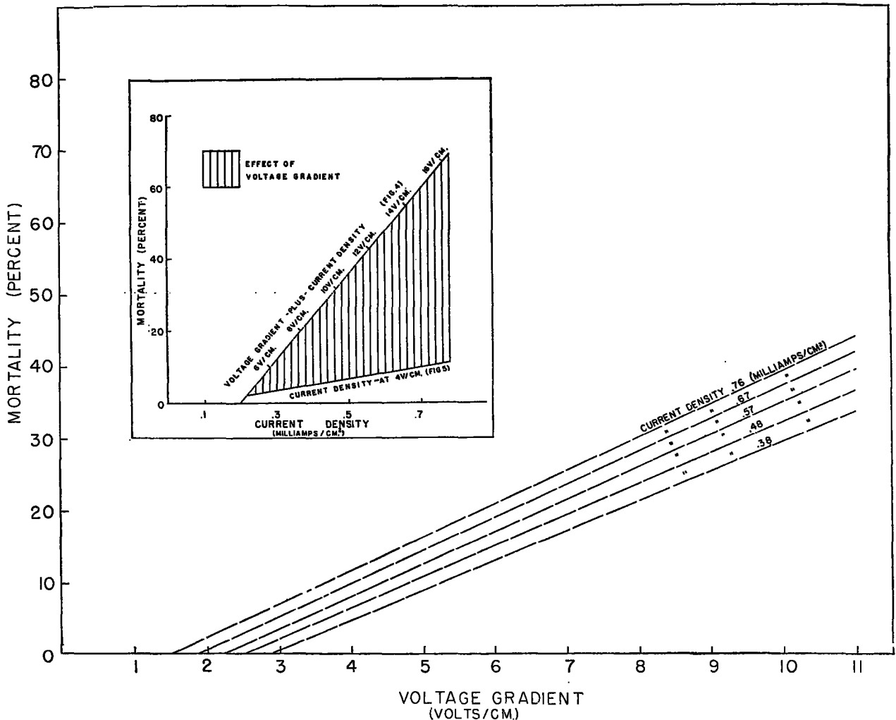
FIGURE 6.—Effect of voltage gradient in relation to current density upon mortality of salmon fingerlings ( Oncorhynchus tshawytscha ) exposed to pulsating d. c. calculated (see insert) from the combined effects of voltage gradient and current density (fig. 4) and the effect of current density (fig. 5).
