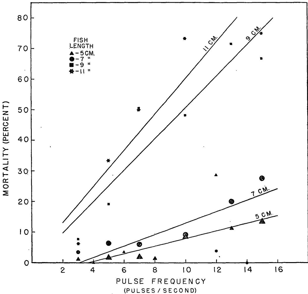
FIGURE 10.—Effect of pulse frequency in relation to fish length upon mortality of salmon fingerlings ( Oncorhynchus tshawytscha ) exposed to pulsating d. c. Tests run at 4 volts/cm., current density range 0.15 to 0.27 milliamps./cm. 2 , pulse duration 20 millisechs., temperature range 10.0° to 19.9° C., duration of exposure 30 seconds. Sizes of symbols correspond to fish number categories: 10-49, 50-99, and 100-199.
