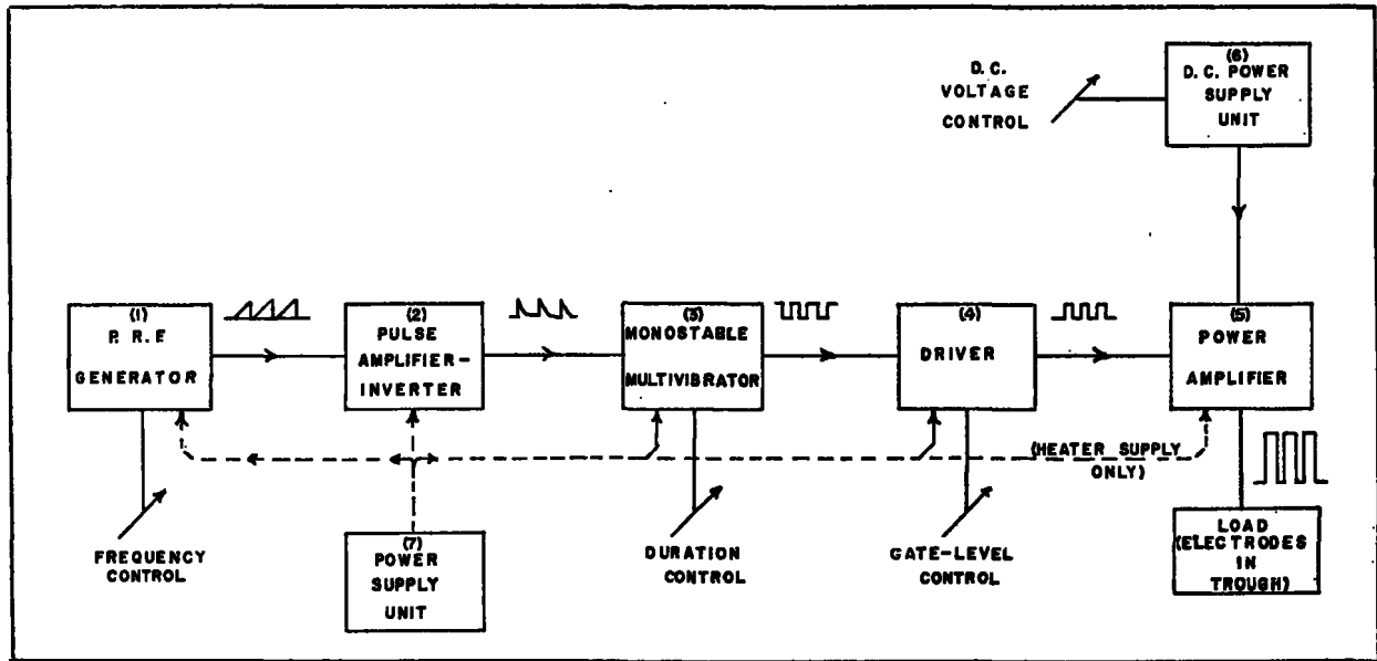
FIGURE 3.—Block diagram of square-wave generator.
