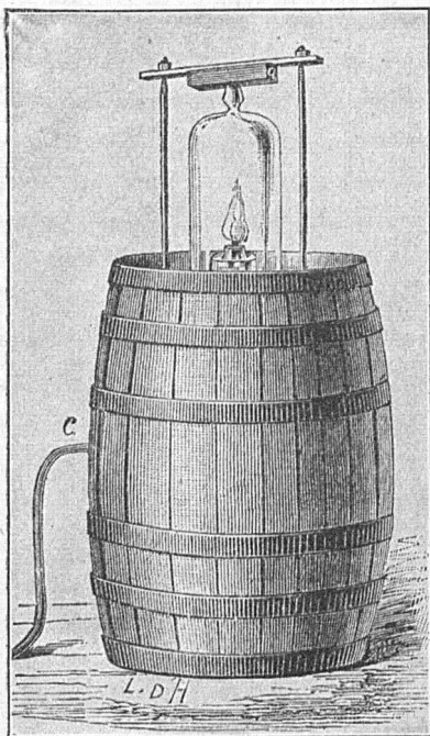
FIG. 8.—Boutan's apparatus for using a magnesium flash-light under water. The reservoir for the magnesium powder, the rubber bulb, and the weights used to steady the apparatus are not shown in the figure. (Copy of fig. 3 in Boutan, 1893.)
