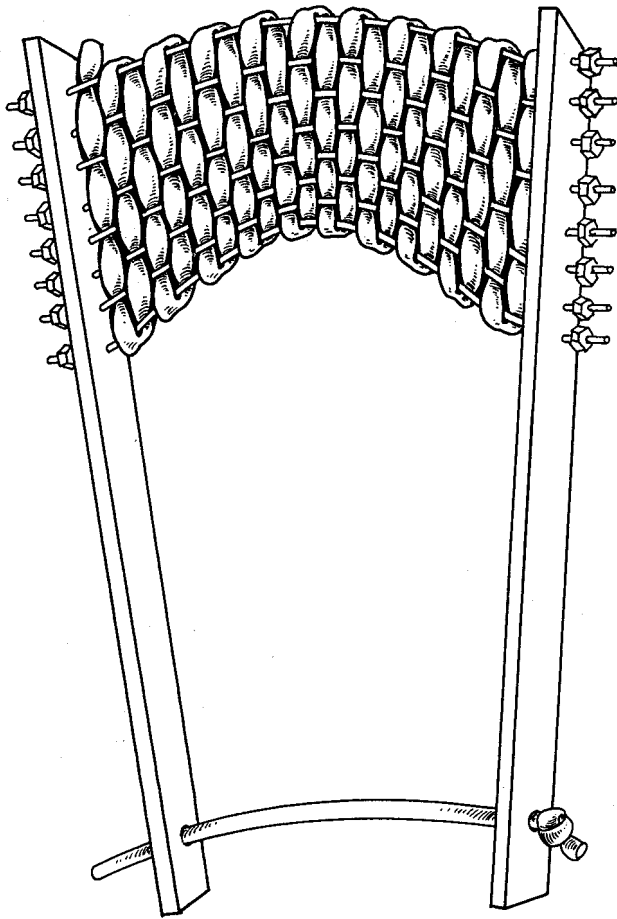
FIGURE 64.—Mechanical model of the ligament of C. virginica . Arches are in scale and correspond to the curves visible in a cross section of the ligament at a magnification of about 100X. Diameter of rubber tubing representing fibrillae is not in scale.
