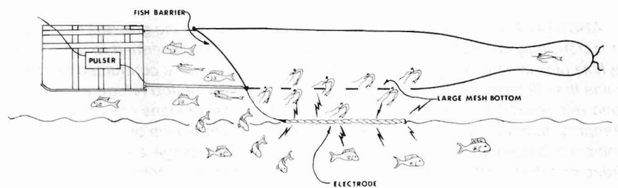
Figure 3.—Selective electric trawl diagram depicting method of shrimp separation employing an electrical field.
