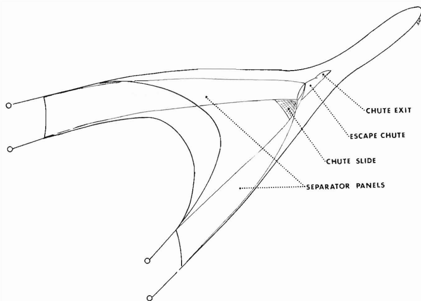
Figure 1.—Webbing panel type shrimp separator trawl design.
