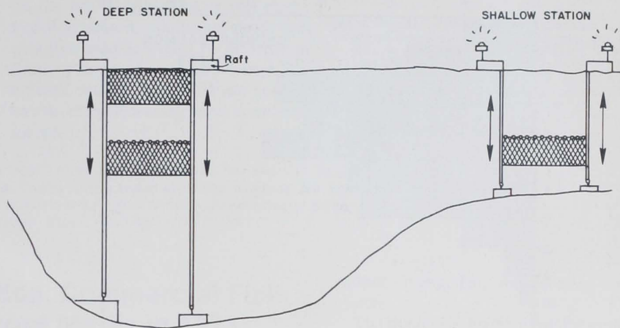
Figure 1.—Diagrammatic sketch of net suspension system for sampling of vertical distribution of juvenile salmonids in Lower Monumental pool, 1973.
