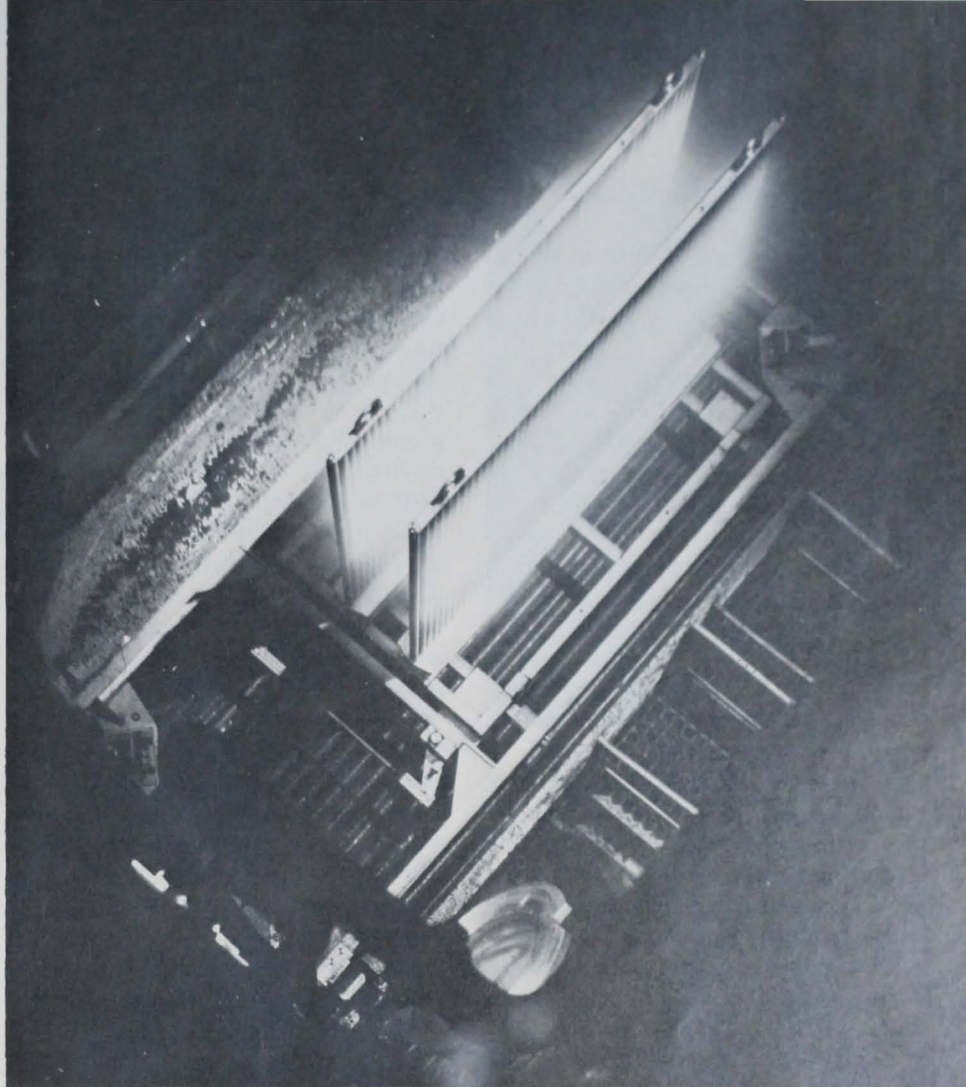
Cobalt-60 irradiation source in water storage pool at U.S. Army Natick Laboratories, Natick, Mass.
