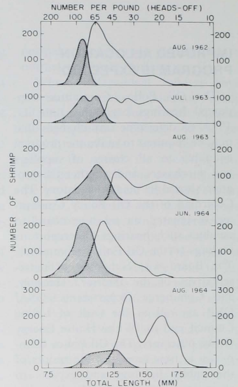
Figure 1.—Length-frequency distributions of brown shrimp that were discarded (shaded areas) or kept (unshaded areas) on the Texas shrimping grounds (from Berry and Benton, 1969).
