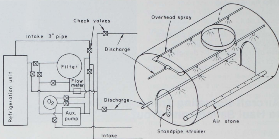
Figure 2. — Diagrammatic view showing life support system in one of the six sections of the tank truck.
