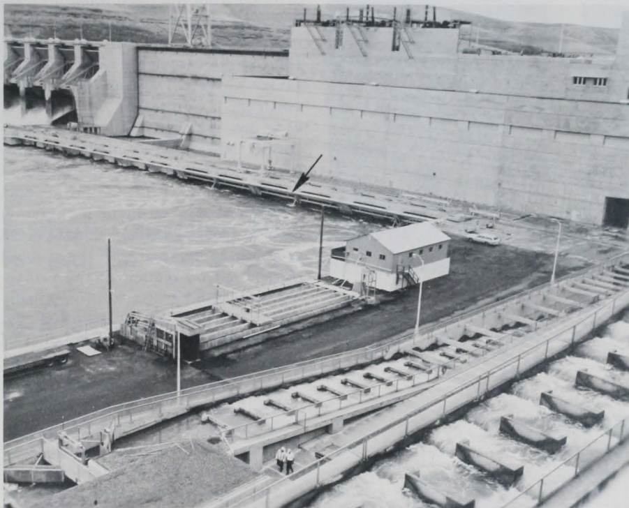
Figure 5. — Collection area into which fish are transferred through a pipe conduit (see arrow) from turbine intake gateways. Here fish are graded by size and held in long raceways for inspection and marking.
