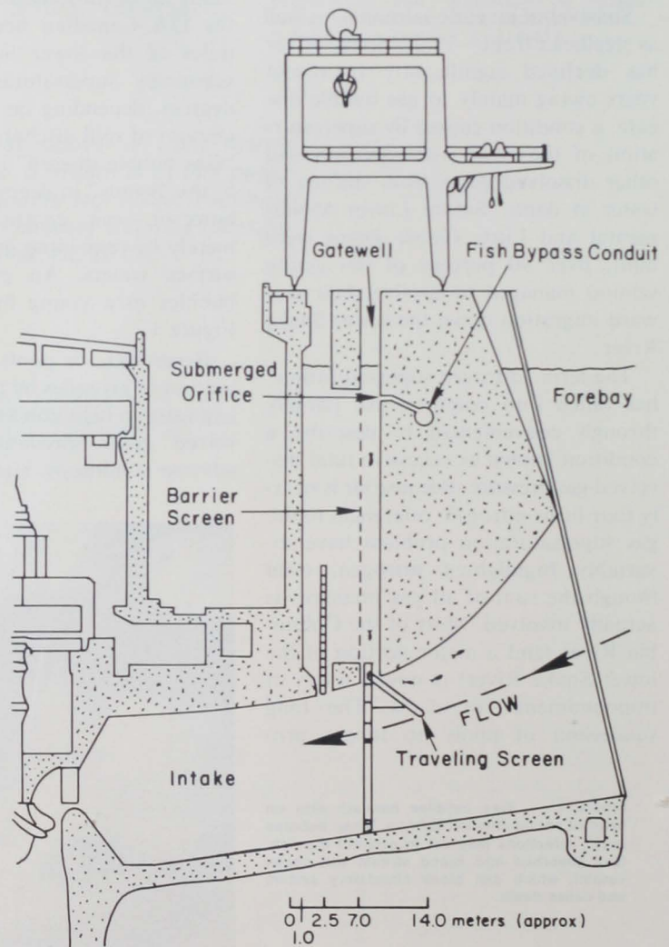
Figure 4.—Sectional view of powerhouse showing traveling screen in operating position within turbine intake.
