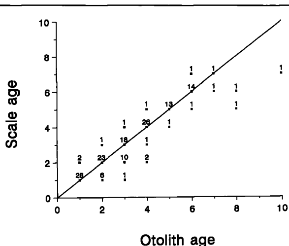
Figure 5 Weakfish, Cynoscion regalis , assigned ages from scales and otoliths. The number of fish each point represents is indicated. The 45° line represents 100% agreement.
