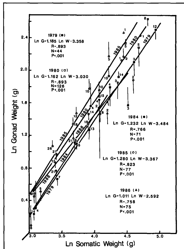
Figure 3 Relationship between the log of ovary weight ( \ln G ) and log female somatic weight ( \ln W ) during each of the five study years. For illustration, mean ovary weight data (+1 SE) are plotted for each 10-g weight class. The equation, G = aW^b (in log-linear form as \ln G = \ln a + b \ln W ), and its summary statistics are provided for each fitted regression line.
