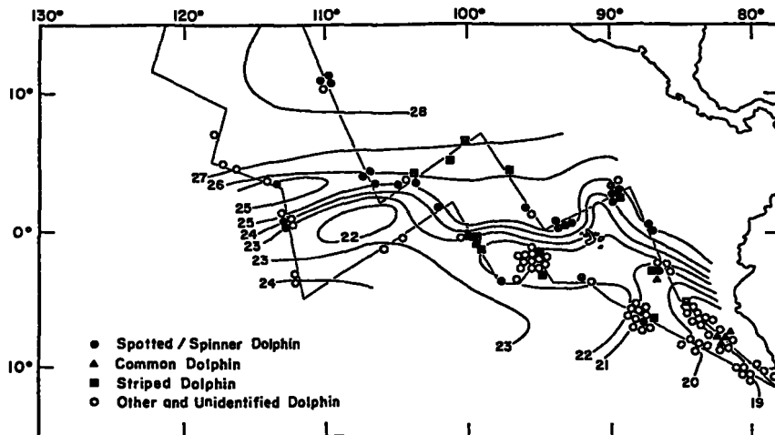
FIGURE 9.—Distribution of dolphin schools in the equatorial region during October-November 1977, relative to surface isotherms ( ^{\circ}\text{C} ). Notice the Equatorial Front or zone of rapid temperature change just north of the Equator. Clumping of sightings along the track is due to nighttime travel by ship. "Other" dolphins are primarily pilot whales.
