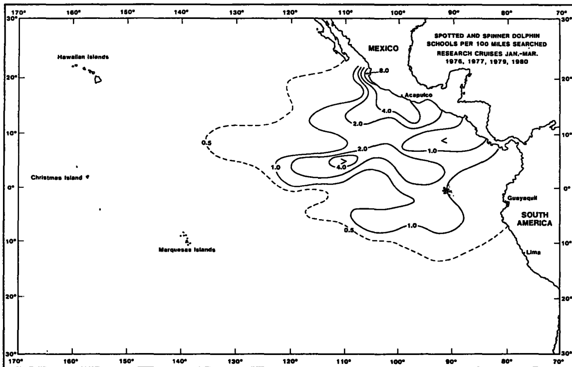
FIGURE 6.—Distribution of relative abundance of spotted and spinner dolphins, inferred from data of the January-March research cruises. Hawaiian and Marquesas sightings are not considered.
