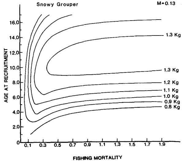
FIGURE 15.—Yield per recruit in weight of snowy grouper where M = 0.13 (from Matheson and Huntsman, see Table 1).
