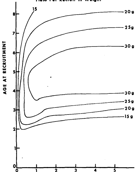
White Grunt M = 0.57 Yield Per Recruit in Weight
