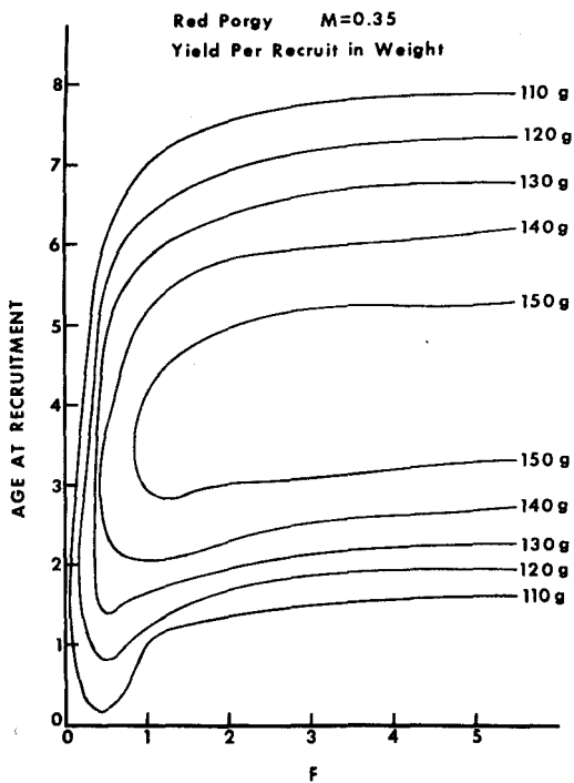
FIGURE 1.—Yield per recruit in weight of red pogy where M = 0.35 .
