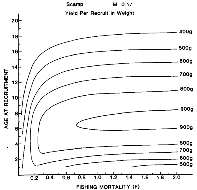
FIGURE 18.—Yield per recruit in weight of scamp where M = 0.17 (from Matheson, Manooch and Huntsman, see Table 1).
