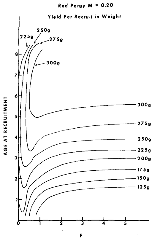
FIGURE 2.—Yield per recruit in weight of red pogy where M = 0.20 .
