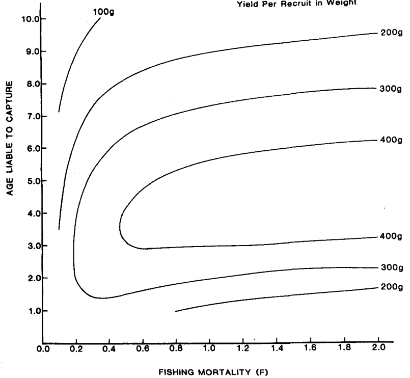
FIGURE 11.—Yield per recruit in weight of red snapper where M = 0.40 .
