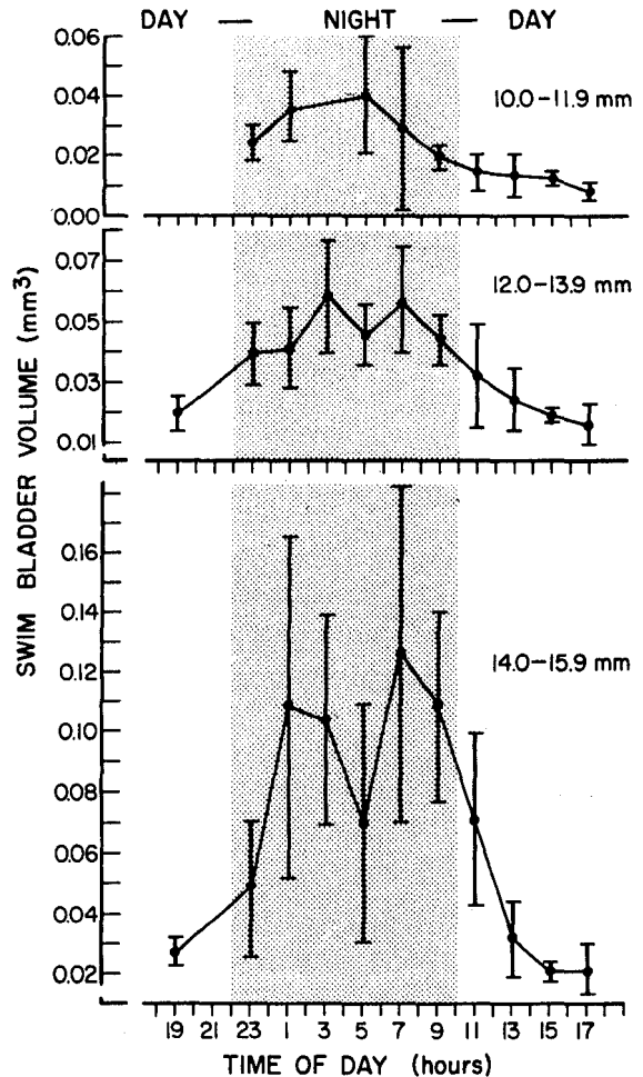
FIGURE 2.—Mean swim bladder volume \pm 2 SE of mean for 2-h class intervals plotted at midpoint of each 2-h class. Data shown for three length classes of laboratory-reared northern anchovy larvae; the onset of dark was at 2200 h and onset of light at 1000 h. No transitional level of illumination existed between night and day.
