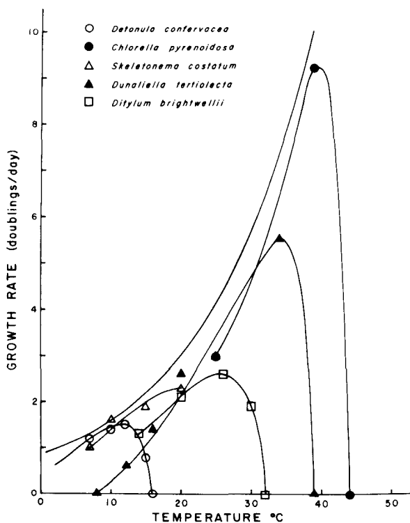
FIGURE 2.—Growth rate vs. temperature curves for five unicellular algae with different temperature optima: Detooula confervacea (Guillard and Ryther, 1962; Smayda, 1969), Skeletonema costatum (Jørgensen, 1968), Ditylum brightwellii (Paasche, 1968), Dunaliella tertiolecta (McLachlan, 1960; Ukeles, 1961; Eppley, 1963; Eppley and Sloan, 1966), Chlorella pyrenoidosa (Sorokin and Krauss, 1958, 1962).
