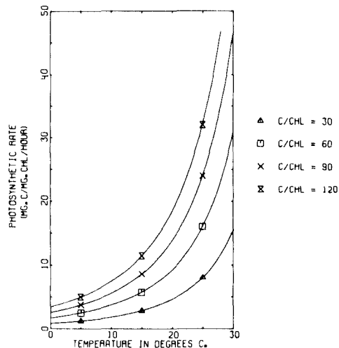
FIGURE 9.—Maximum expected photosynthetic rate (assimilation number) from Equations (1) and (5) with the assumption that the growth rate will be one-half the value predicted by Equation (1) to adjust for natural daylength averaging 12 hr light/day. Photosynthetic rates are expressed as milligrams carbon assimilated/milligram chlorophyll a /hour. This figure gives values more in line with ocean measurements than does Figure 8.
