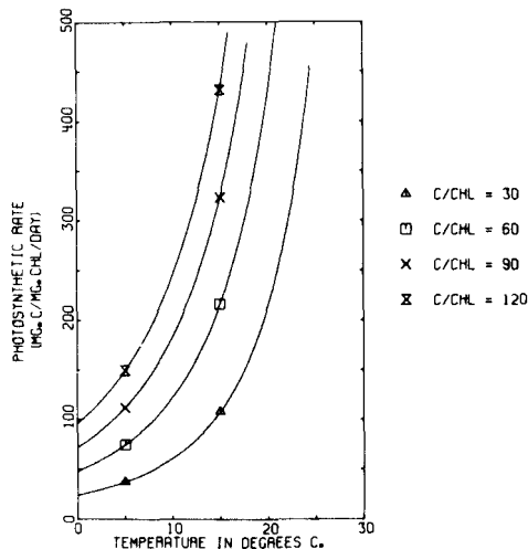
FIGURE 8.—The variation in maximum expected rate of photosynthesis (assimilation number) with temperature. Rates were computed by combining Equations (1) and (5) and are expressed as milligrams carbon/milligram chlorophyll a /day. Continuous light was assumed.
