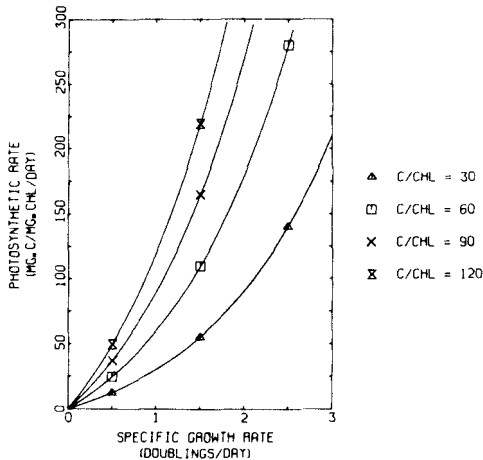
FIGURE 6.—Photosynthetic rate (assimilation number/day) vs. the specific growth rate of the phytoplankton computed from Equation (5). Photosynthetic rate is expressed as milligrams carbon assimilated per day per milligram chlorophyll a and is shown for several values of the ratio carbon/chlorophyll a in the phytoplankton crop (30, 60, 90, and 120 g/g).
