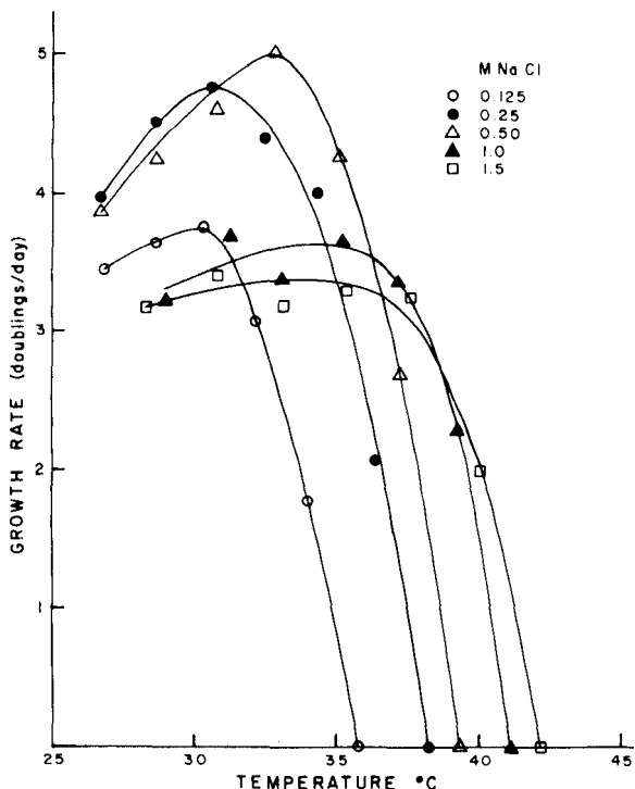
FIGURE 3.—Growth rate vs. temperature curves for Dunaliella tertiolecta measured in culture media containing different salt concentrations (R. W. Eppley and F. M. Macias, unpublished data).
