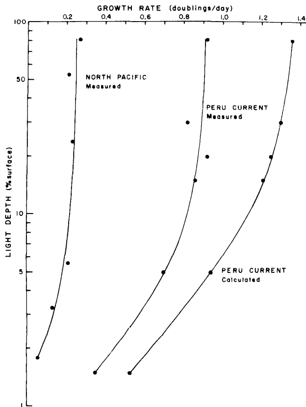
FIGURE 5.—Variation in growth rate of natural marine phytoplankton with depth in the Peru Current, June 1969, and in the subtropical North Pacific central gyre, November 1971 (this laboratory, unpublished). The "light depth" of the ordinate was calculated as the radiant energy at depth as a percentage of that at the surface so that data from the two regions, with euphotic zone depths of about 30 and about 150 m, could be compared. The calculated line is based on Equation (1) for 19°C with the assumption that light limits growth rate below the surface. The \mu_{\max} from Equation (1) was multiplied by (I/2.5 + I) where I is the radiant energy at depth as percent of surface. The half-saturation constant of 2.5% is low (see Rodhe, 1965) and suggests that the Peru Current phytoplankton were "shade adapted." Hence, measured \mu would be less than expected from Equation (1), in spite of abundant nutrients. In the North Pacific study enrichment experiments and other data suggested limitation of phytoplankton growth rate by both nitrogen and phosphorus concentration (Perry, Renger, Eppley, and Venrick, unpublished data). There the temperature in the mixed layer was 22°C and the maximum expected value would be slightly greater than shown for the Peru Current.
