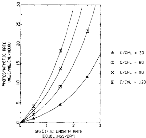
FIGURE 7.—Same as Figure 6, but photosynthetic rates (assimilation numbers) were calculated per hour, rather than per day, assuming 12 hr light per day (i.e., values of Figure 6 were divided by 12).
