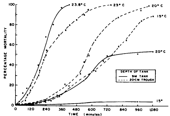
FIGURE 5.—Comparison of LE_{100} curves for coho salmon acclimated at 10° C and subjected to three temperatures (15°, 20°, and 23° C) in 20-cm and 9-m deep tanks containing water supersaturated with nitrogen gas at 130% saturation. Oxygen concentrations varied from 115 to 125% saturation.
