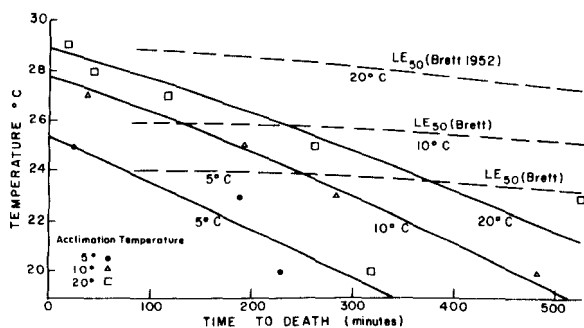
FIGURE 2.—Median-resistance-time ( LE_{50} ) plotted from temperature tolerance tests with coho salmon fingerlings acclimated at 5°, 10°, and 20° C and stressed for 12 hr at 115-120% saturation of N_2 , then subjected to temperature increases in water supersaturated at 125-130%. Brett's LE_{50} curves for fish acclimated at 5° and 20° C—without N_2 stress—are shown for comparison.
