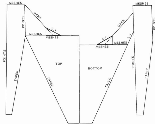
Figure 4.—Semiballoon trawl generalized schematic.
