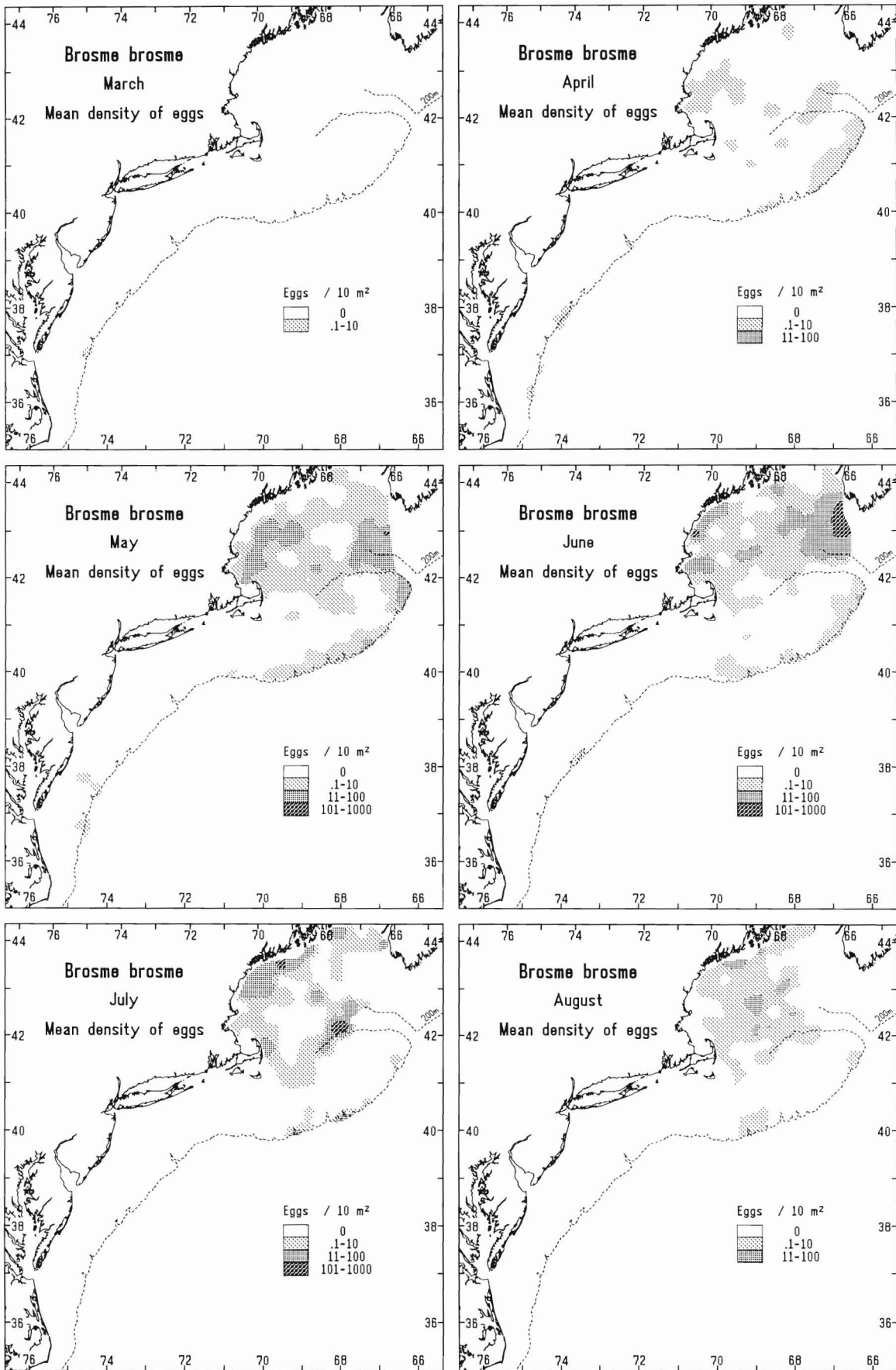
Figure 22 Brosme brosme ; composite monthly areal plots of mean egg densities (no./10 m²).
