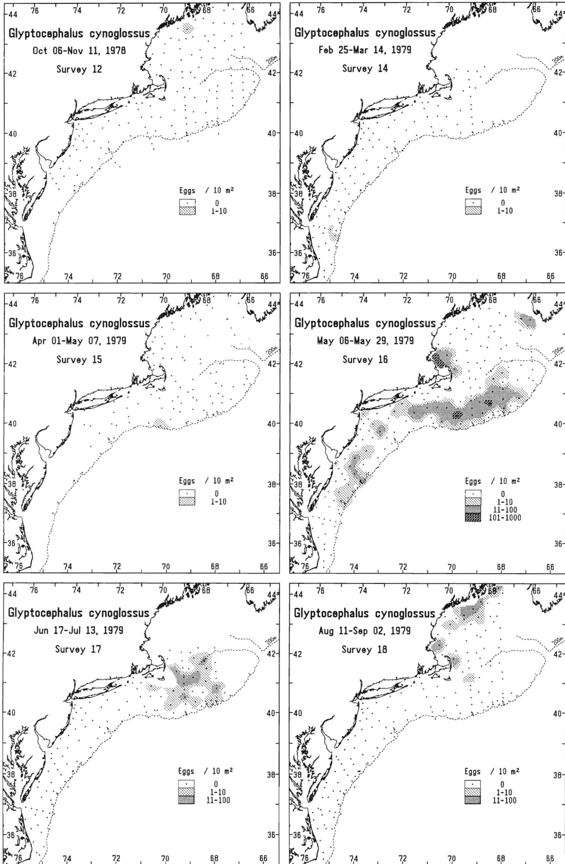
Figure 98 Glyptocephalus cynoglossus ; survey areal plots of egg densities (no./10 m 2 ).
