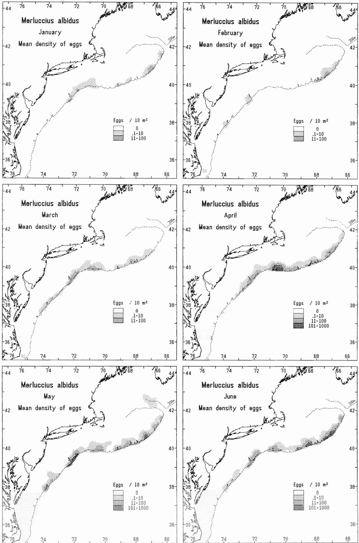
Figure 34 Merluccius albidus ; composite monthly areal plots of mean egg densities (no./10 m 2 ).
