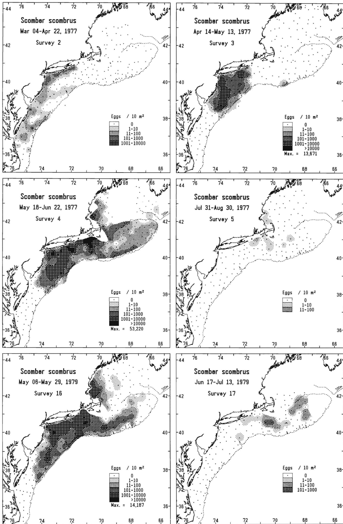
Figure 80 Scomber scombrus ; survey areal plots of egg densities (no./10 m 2 ).
