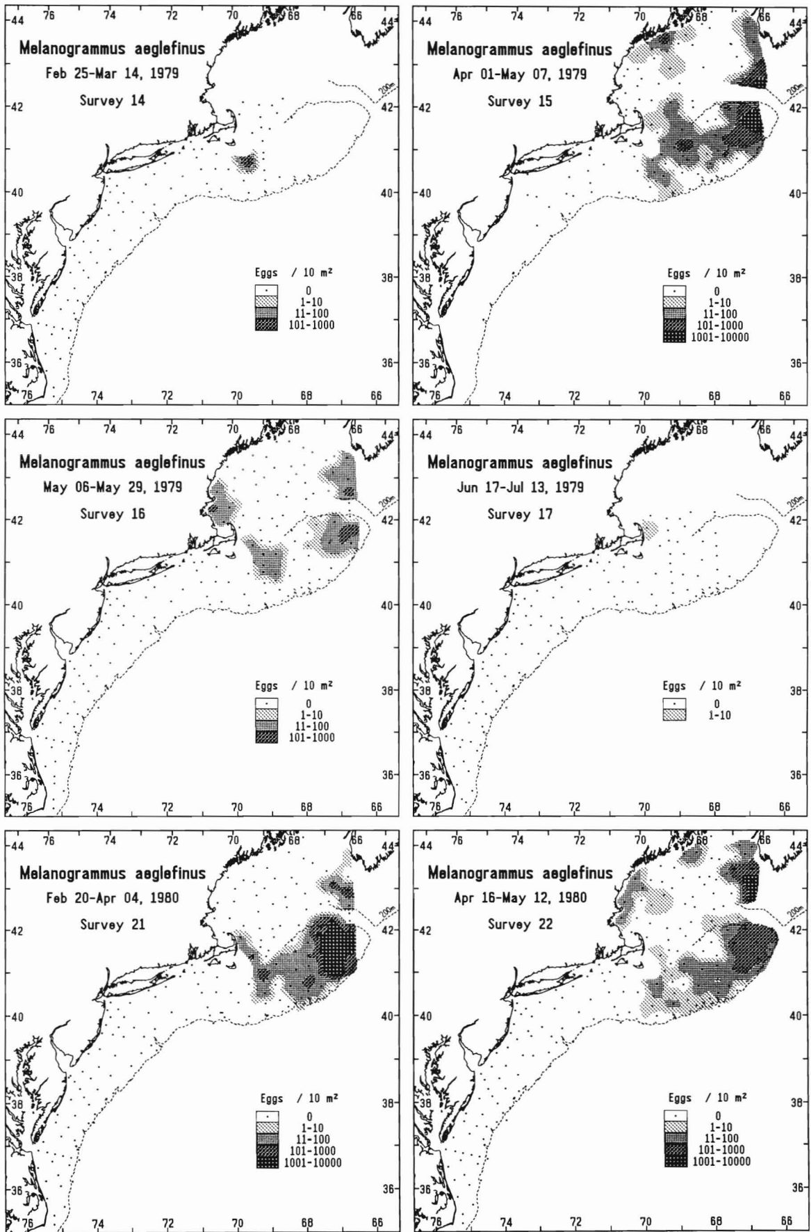
Figure 32 Melanogrammus aeglefinus ; survey areal plots of egg densities (no./10 m 2 ).
