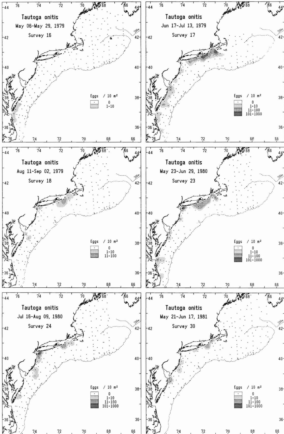
Figure 65 Tautoga onitis ; survey areal plots of egg densities (no./10 m 2 ).
