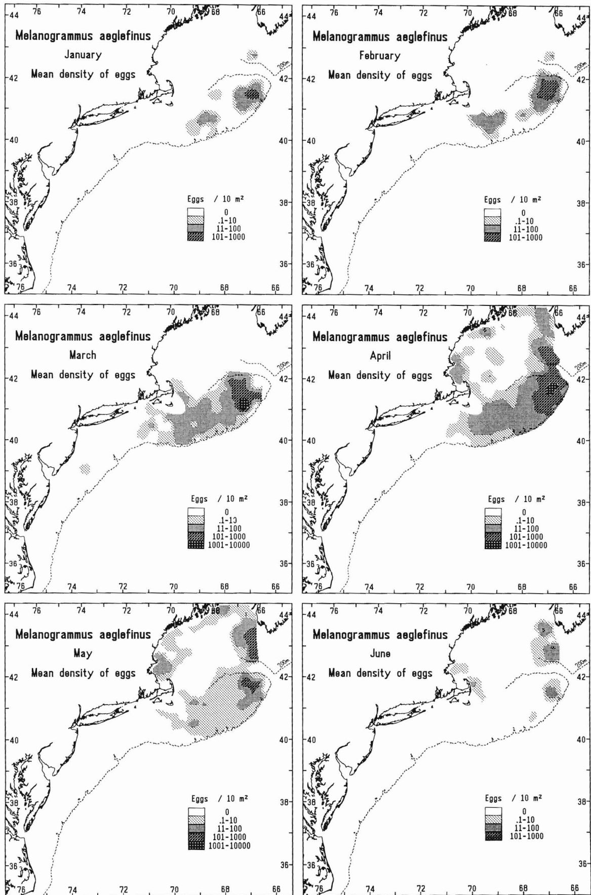
Figure 31 Melanogrammus aeglefinus ; composite monthly areal plots of mean egg densities (no./10 m 2 ).
