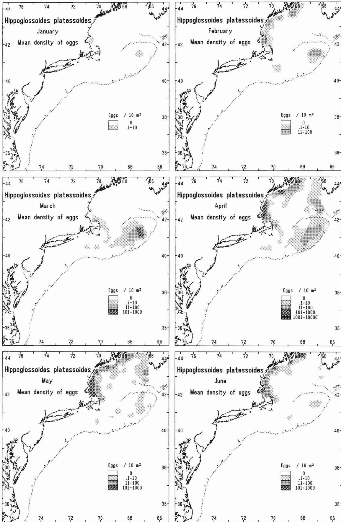
Figure 100 Hippoglossoides platessoides ; composite monthly areal plots of mean egg densities (no./10 m 2 ).
