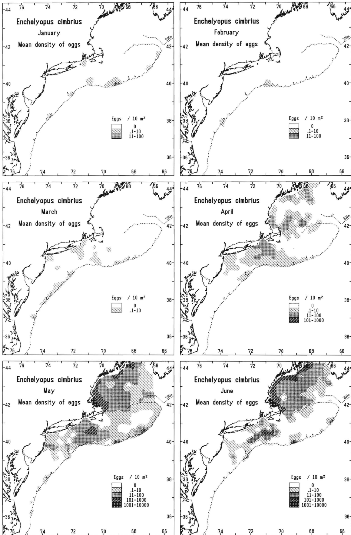
Figure 25 Enchelyopus cimbricus ; composite monthly areal plots of mean egg densities (no./10 m 2 ).
