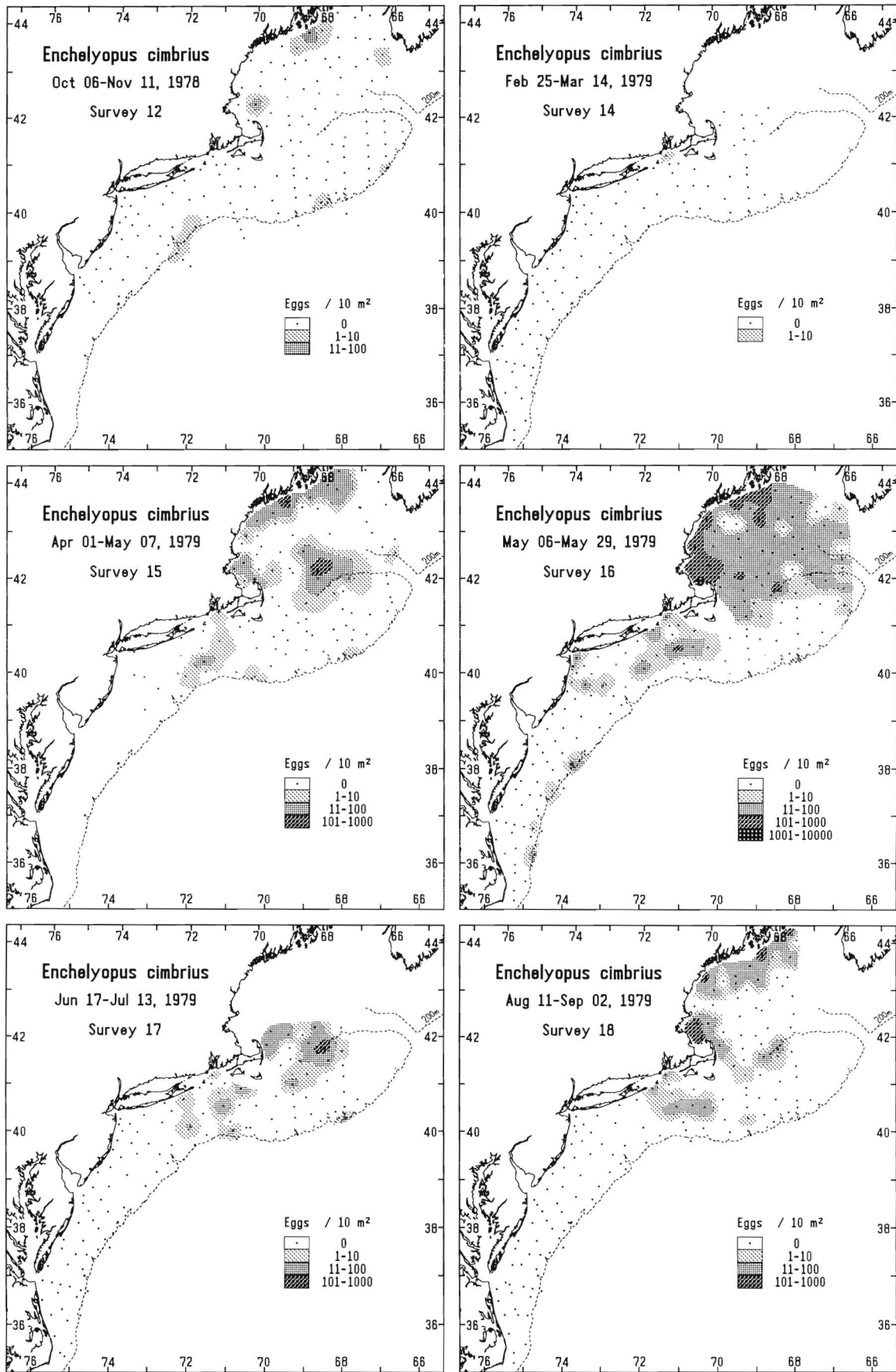
Figure 26 Enchelyopus cimbrinus ; survey areal plots of egg densities (no./10 m 2 ).
