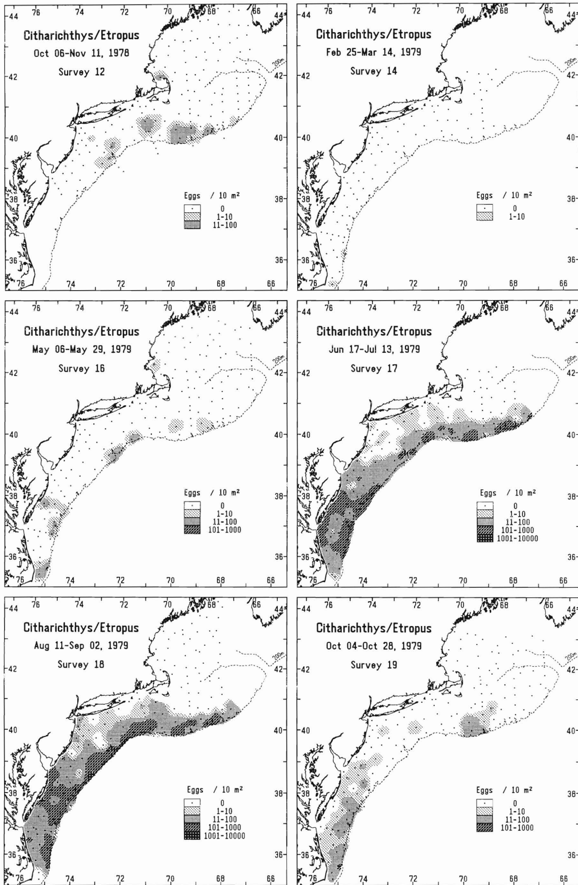
Figure 86 Citharichthys/Etropus ; survey areal plots of egg densities (no./10 m 2 ).
