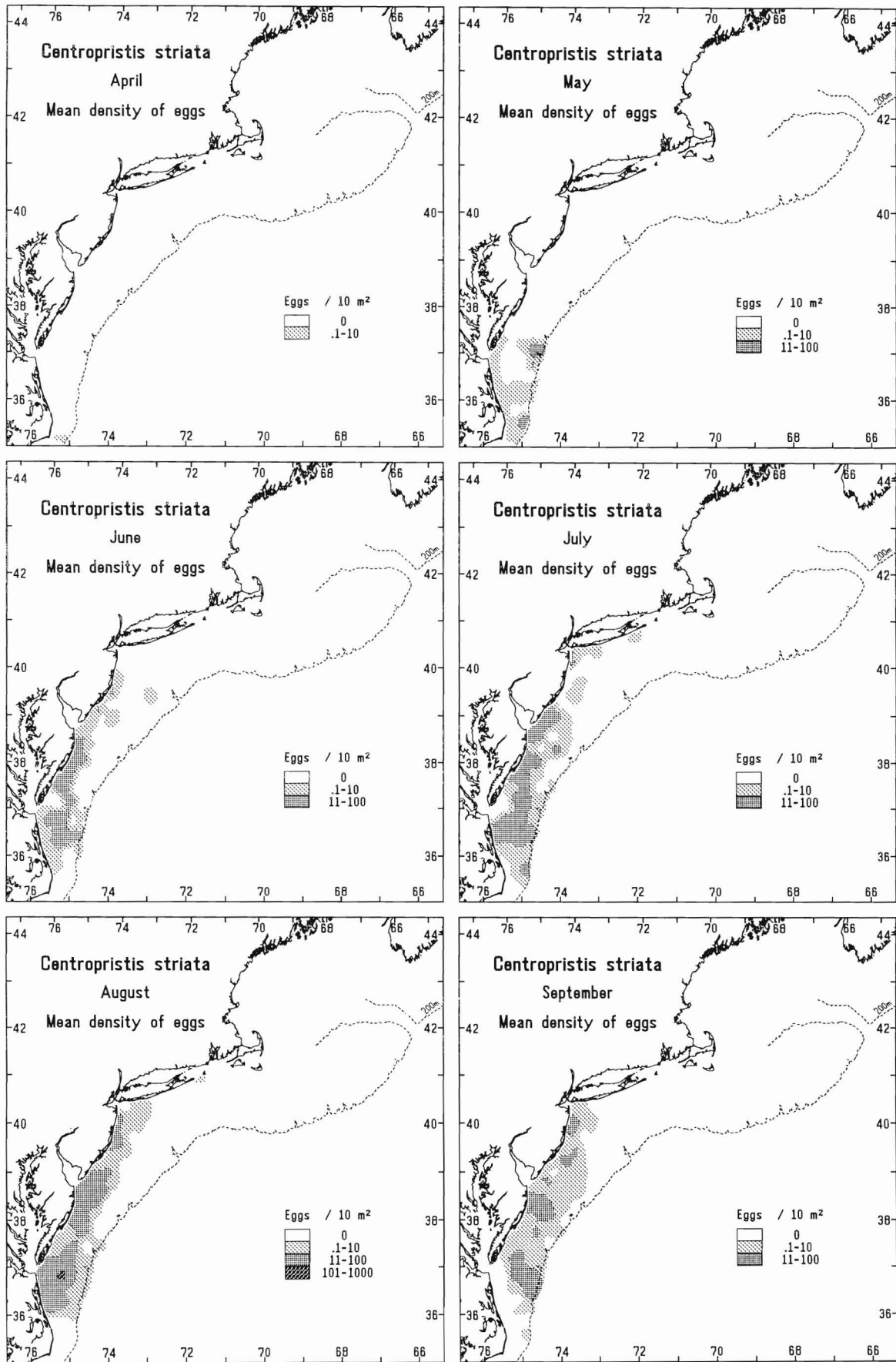
Figure 49 Centropristis striata ; composite monthly areal plots of mean egg densities (no./10 m 2 ).
