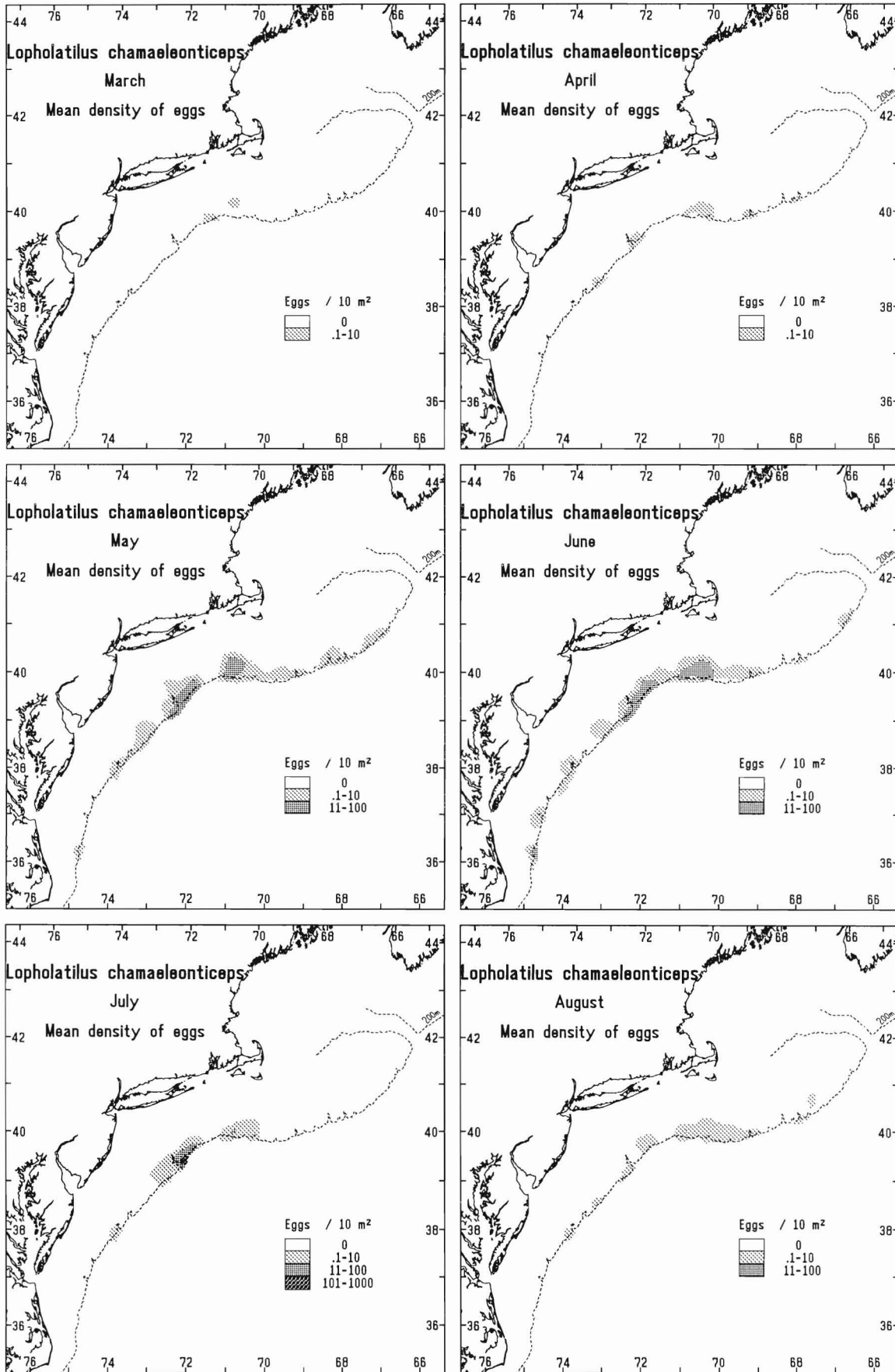
Figure 52 Lopholatilus chamaeleonticeps ; composite monthly areal plots of mean egg densities (no./10 m 2 ).
