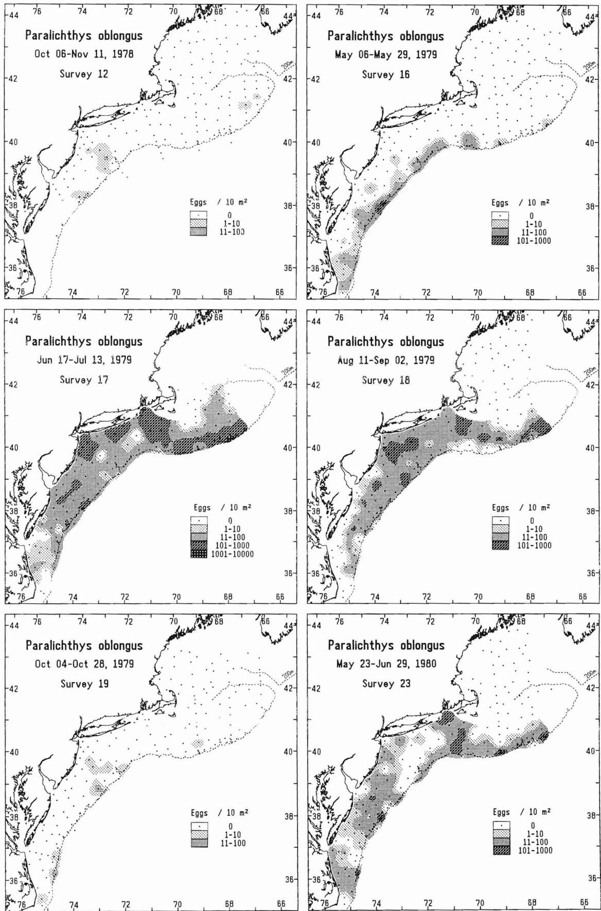
Figure 92 Paralichthys oblongus ; survey areal plots of egg densities (no./10 m 2 ).
