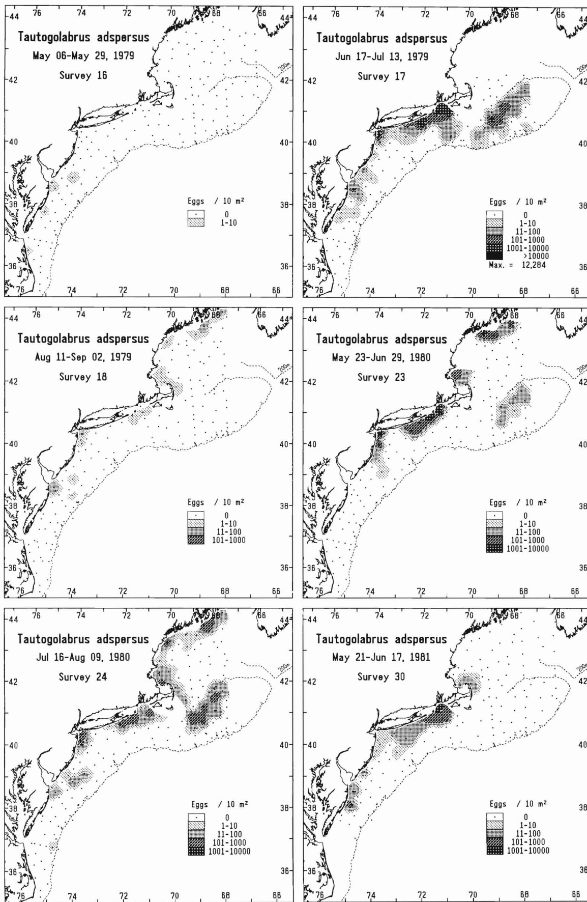
Figure 68 Tautoglabrus adspersus ; survey areal plots of egg densities (no./10 m 2 ).
