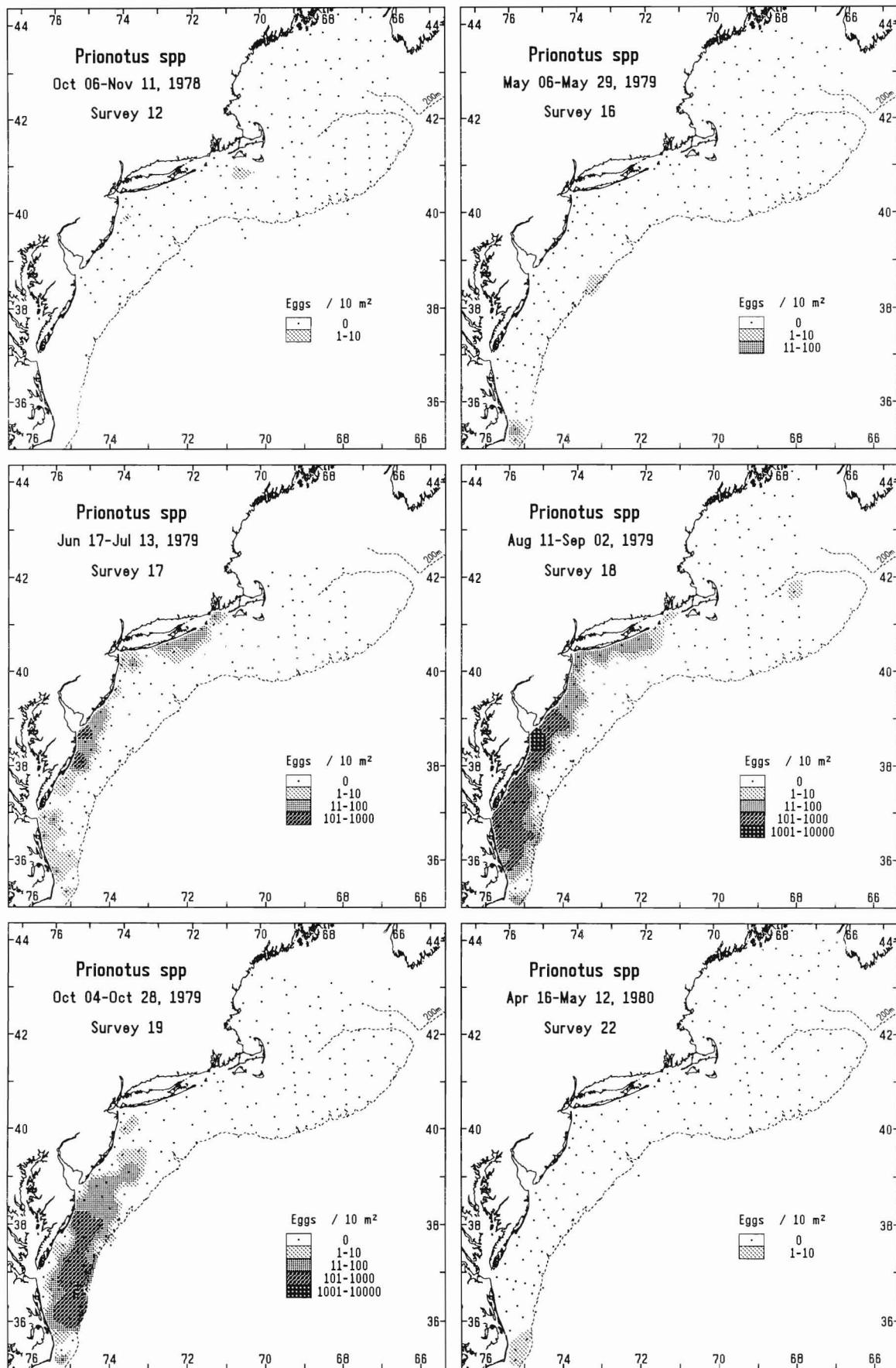
Figure 47 Prionotus spp.; survey areal plots of egg densities (no./10 m 2 ).
