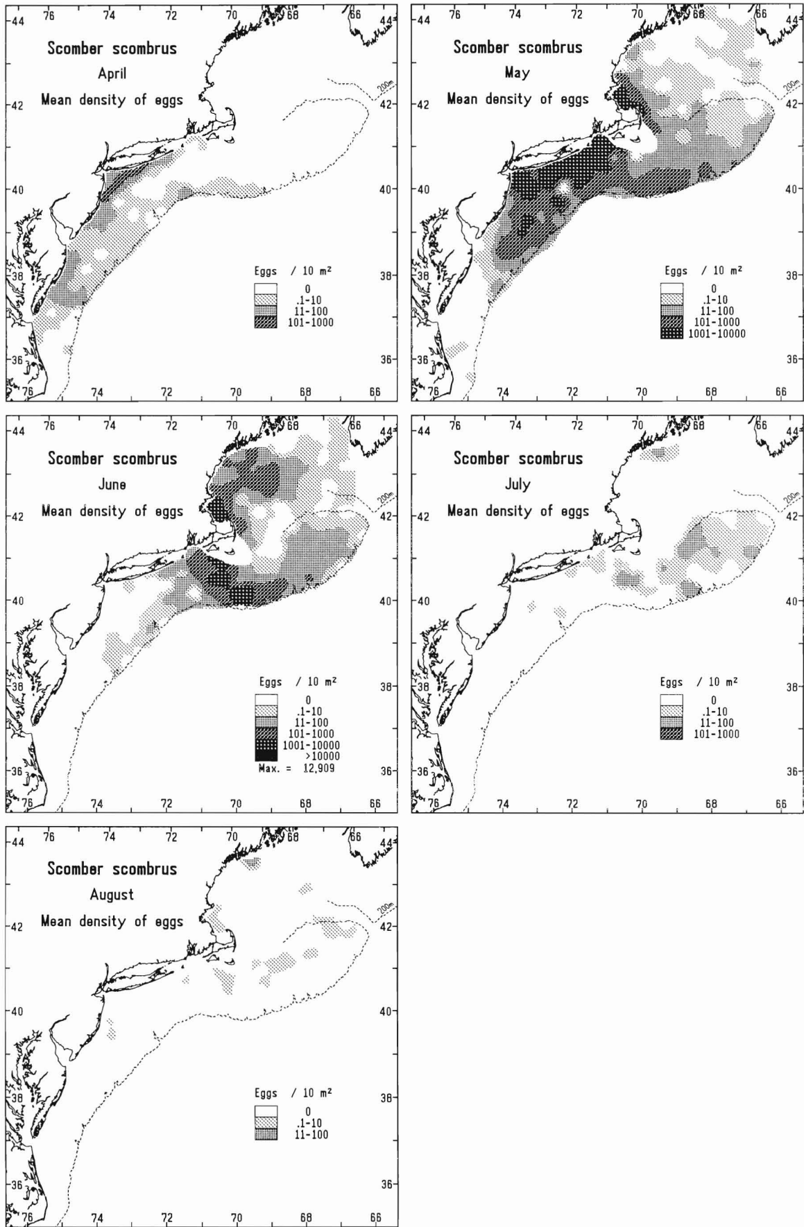
Figure 79 Scomber scombrus ; composite monthly areal plots of mean egg densities (no./10 m 2 ).
