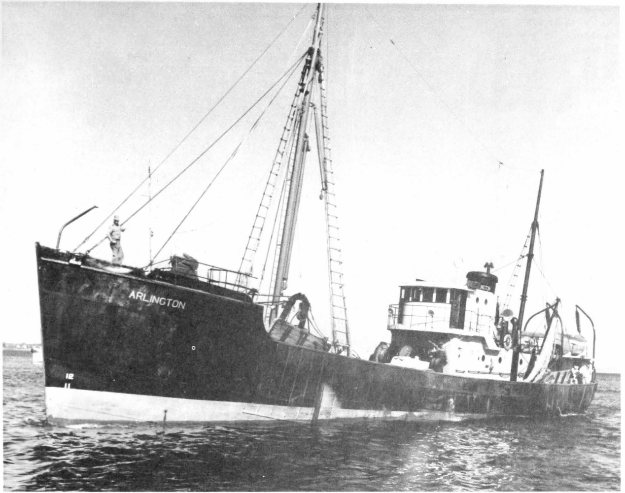
Figure 4.--A typical large otter trawler, mainstay of the Boston haddock fleet. Vessels such as this travel 150 to 200 miles out to sea to catch haddock.
