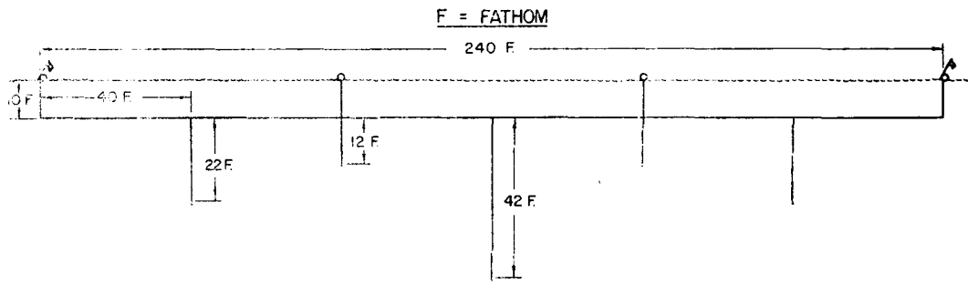
ARRANGEMENT OF A BASKET OF GEAR USED ON SMITH CRUISE 5
