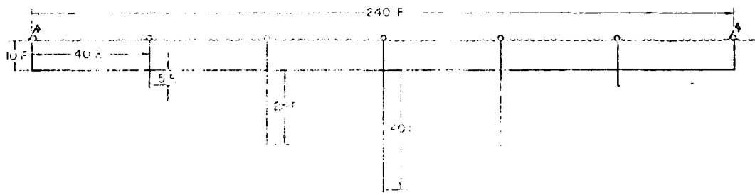
ARRANGEMENT OF A BASKET OF GEAR USED ON STATION 9 THROUGH 19, SMITH CRUISE 7
