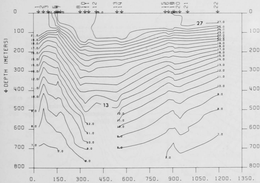
Figure 2. — Gulf Shipper , 7302, stations 1-22, 12-15 February 1973.
