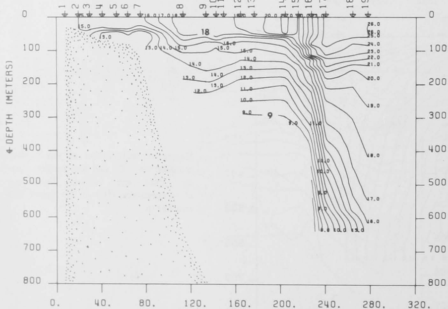
Figure 9. — Mormac Rigel , 7311, stations 1-19, 1 November 1973.
