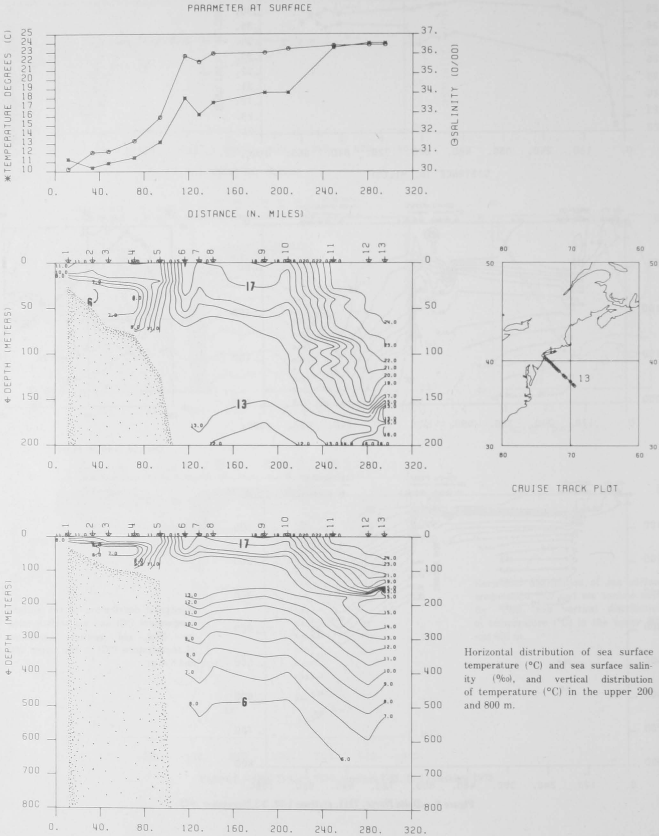
Figure 7.—Mormac Argo, 7305, stations 1-13, 12-13 May 1973.
