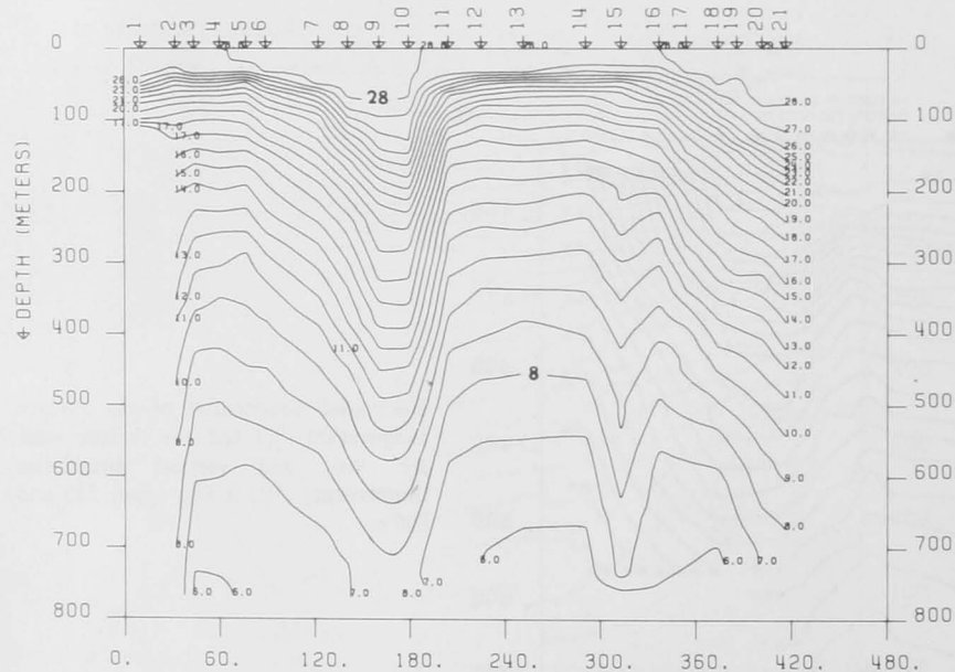
Figure 5. — Gulf Trader, 7310, stations 1-21, 14-15 October 1973.
