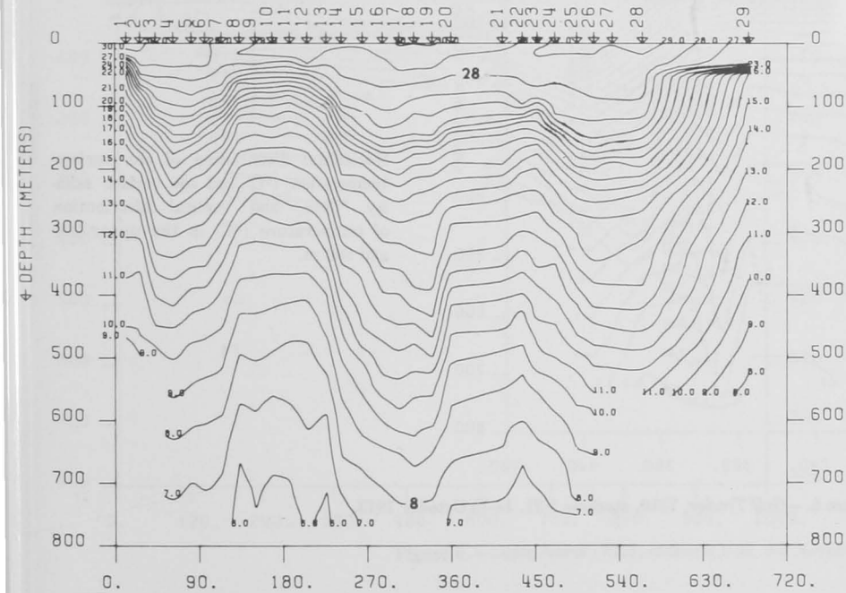
Figure 4.—Gulf Trader, 7308, stations 1-29, 1-2 August 1973.
