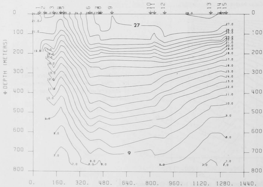
Figure 3.—Gulf Shipper, 7304, stations 1-15, 20-24 April 1973.
