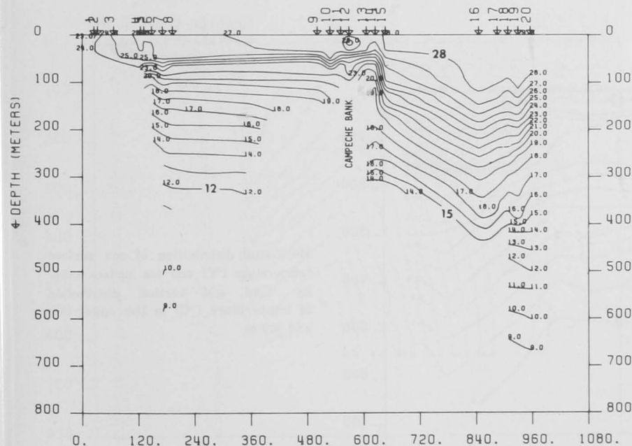
Figure 6. — Delta Norte, 7311, stations 1-20, 3-5 November 1973.
