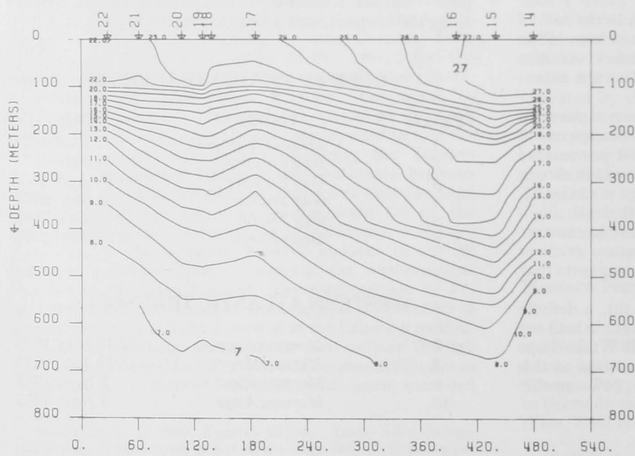
Figure 1. — Delta Argentina , 7211, stations 14-22, 1-2 January 1973.
