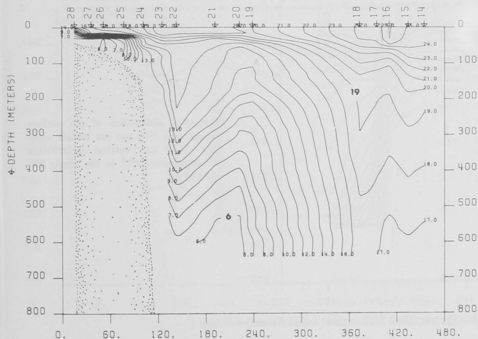
Figure 8. — Mormac Argo , 7305, stations 28-14, 17-18 June 1973.
