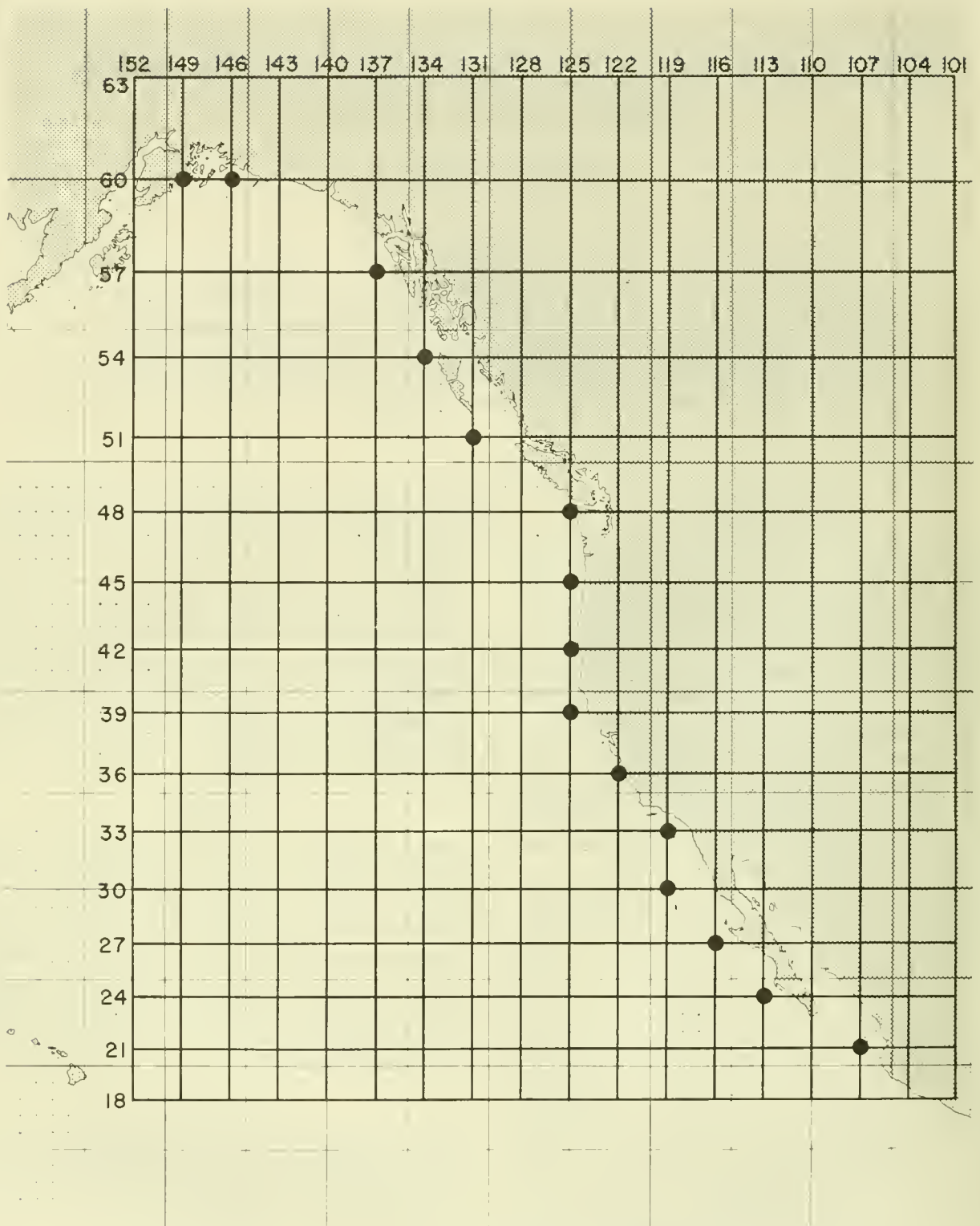
Figure 1.—Data grid. Intersections at which upwelling indices are computed are marked with large dots.
