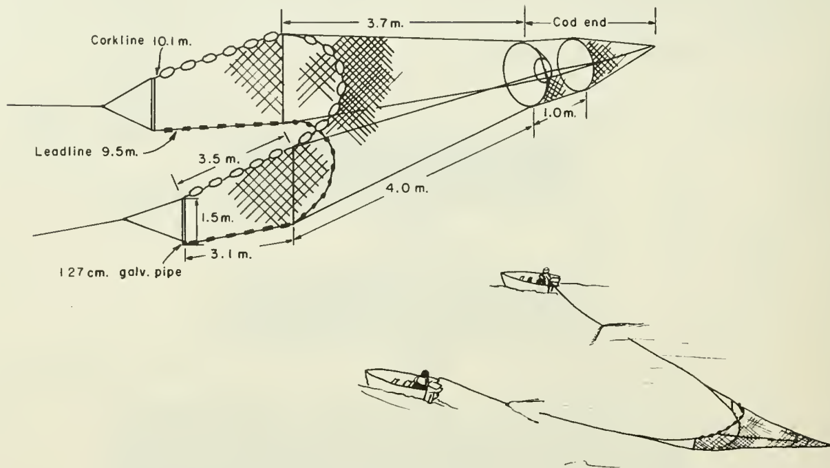
Figure 3.--Two-boat trawl used to sample distribution of juvenile salmonids in Mayfield Reservoir.
