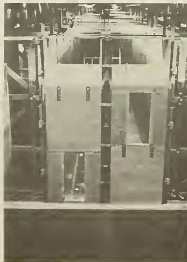
Figure 5.--Test condition for comparing responses of salmon to vertical orifices at deep (left) and shallow (right) settings.
