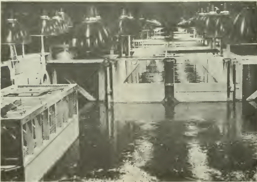
Figure 6.--Introductory pool (foreground) during discharge from shallow (A) and deep (B) orifices. Salmon were released from structure in left foreground.
