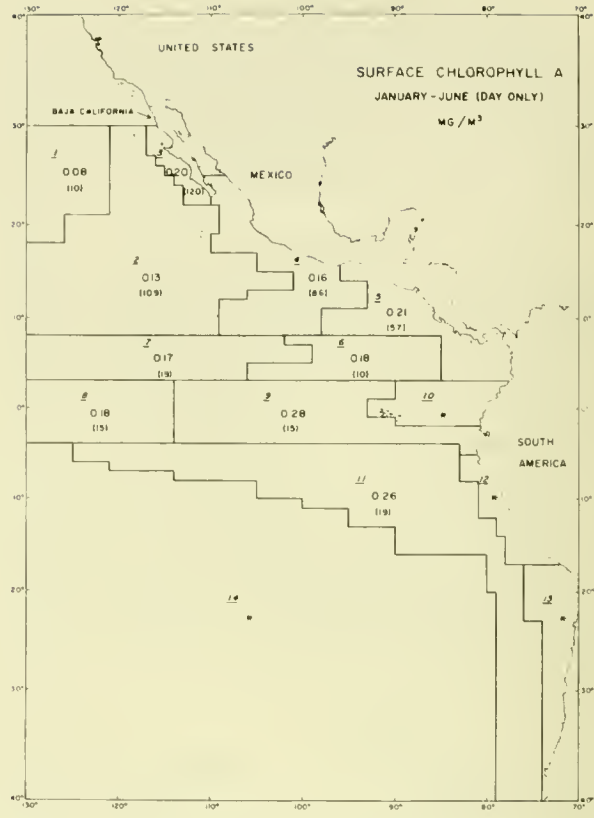
Figure 4.--Geometric means and (in parentheses) numbers of observations of surface chlorophyll a in milligrams per cubic meter, for each of the areas 1 to 14, in January to June. Daylight data only; asterisk indicates <10 observations; for further explanation see text.
