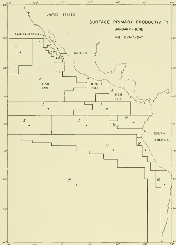
Figure 5.--Geometric means and (in parentheses) numbers of observations of surface primary productivity in milligrams of carbon per cubic meter per day, for each of the areas 1 to 14, in January to June. Daylight data only; asterisk indicates <10 observations; for further explanation see text.
