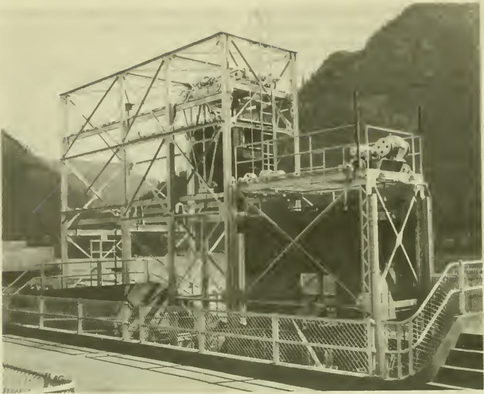
Figure 2.--Trapping facilities, Washington shore fishway, Bonneville Dam.
