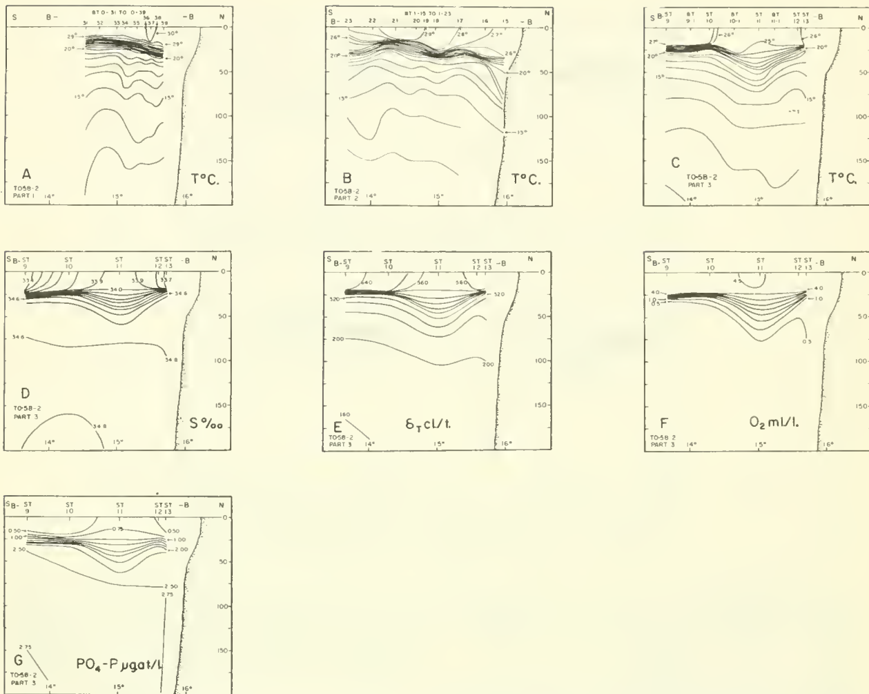
Figure 12.--Vertical distributions of properties on cruise TO-58-2, parts 1, 2, and 3, along section B-B (see fig. 8); depth scale in m.
