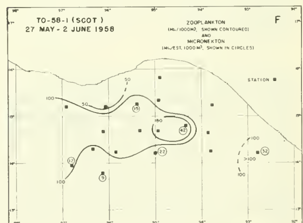
Figure 4.--Horizontal distributions of properties on cruise TO-58-1.
