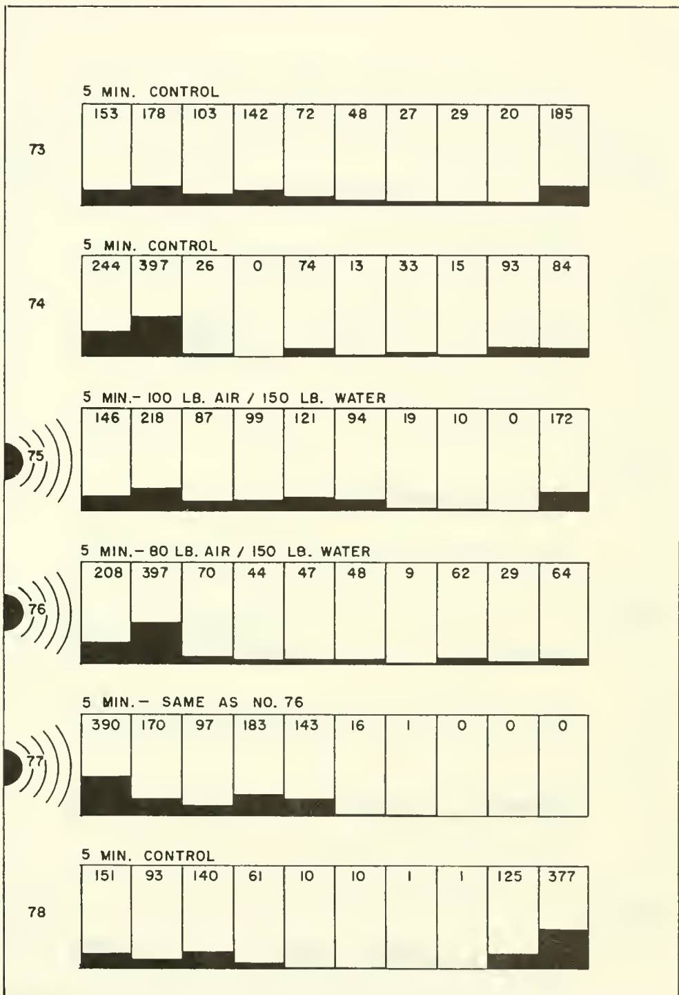
Figure 24.--Distribution of fish in pens, experiments 73-78. All experiments started with 100 fish in each pen. In controls, gates between pens lifted for indicated period, then lowered. Tests same, except sounds under indicated operating conditions applied for indicated time at indicated location. Numbers and dark bars show distribution of fish after gates lowered.
