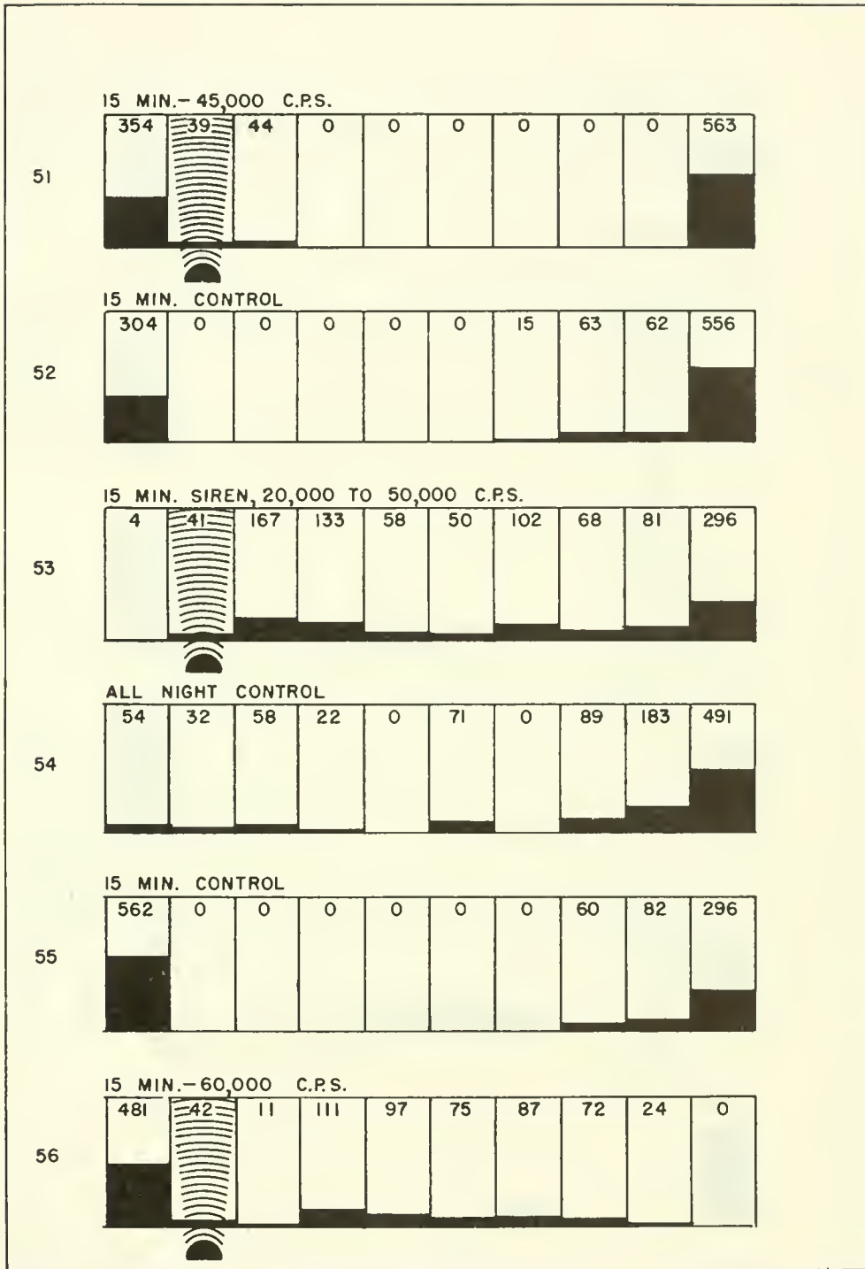
Figure 17.--Distribution of fish in pens, experiments 51-56, Experiments 51-53, 55, 56 started with 1,000 fish in pen No. 1 (far left); 54 started with 1,000 fish in pen No. 10 (far right). In controls, gates between pens lifted for indicated period, then lowered, Tests same, except sounds of indicated durations and frequencies (cycles per second) applied at indicated location while gates up. Numbers and dark bars show distribution of fish after gates lowered.
