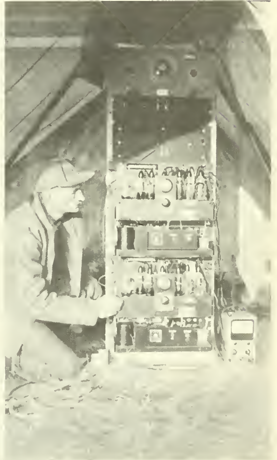
Figure 7.-- Power amplifiers and signal generator used to provide sound to the underwater speaker shown in figure 6.
