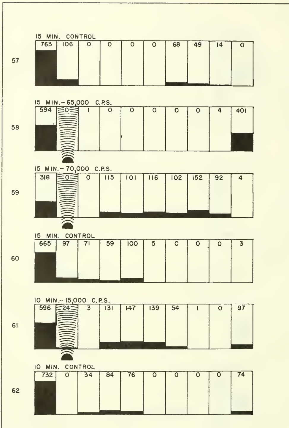
Figure 18.--Distribution of fish in pens, experiments 57-62. All experiments started with 1,000 fish in pen No. 1 (far left). In controls, gates between pens lifted for indicated period, then lowered. Tests same, except sounds of indicated durations and frequencies (cycles per second) applied at indicated location while gates up. Numbers and dark bars show distribution of fish after gates lowered.
