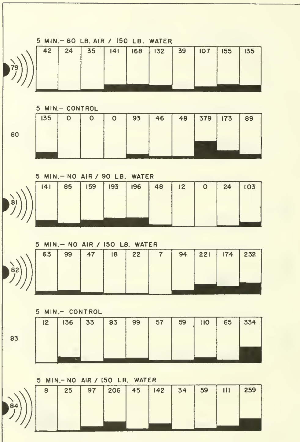
Figure 25.--Distribution of fish in pens, experiments 79-84. All experiments started with 100 fish in each pen. In controls, gates between pens lifted for indicated period, then lowered. Tests same, except sounds under indicated operating conditions applied for indicated time at indicated location. Numbers and dark bars show distribution of fish after gates lowered.
