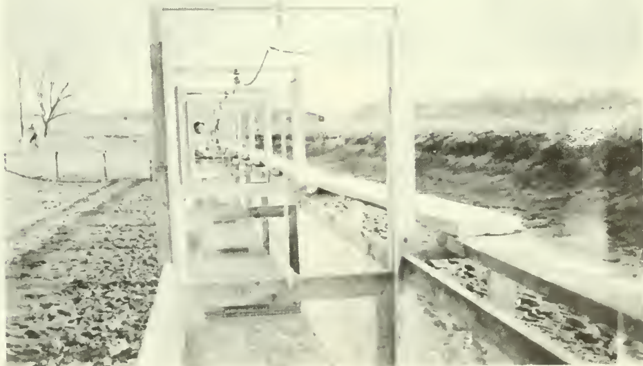
Figure 2.--Dry pond, trap structure completed, gates rigged and in place.
