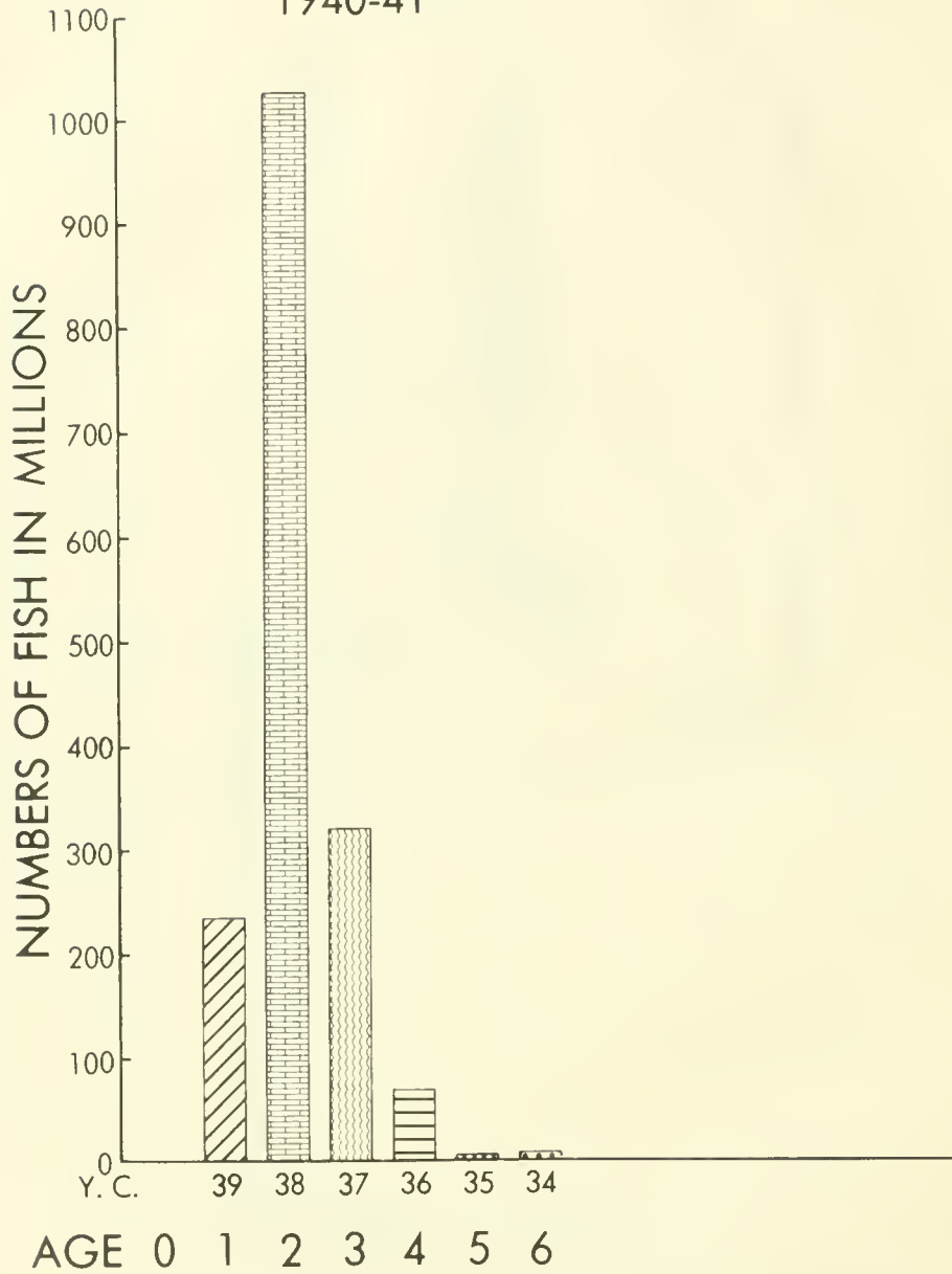
Figure 20.--Catch in millions of fish, by age and year class, for San Pedro for the season 1940-41.
