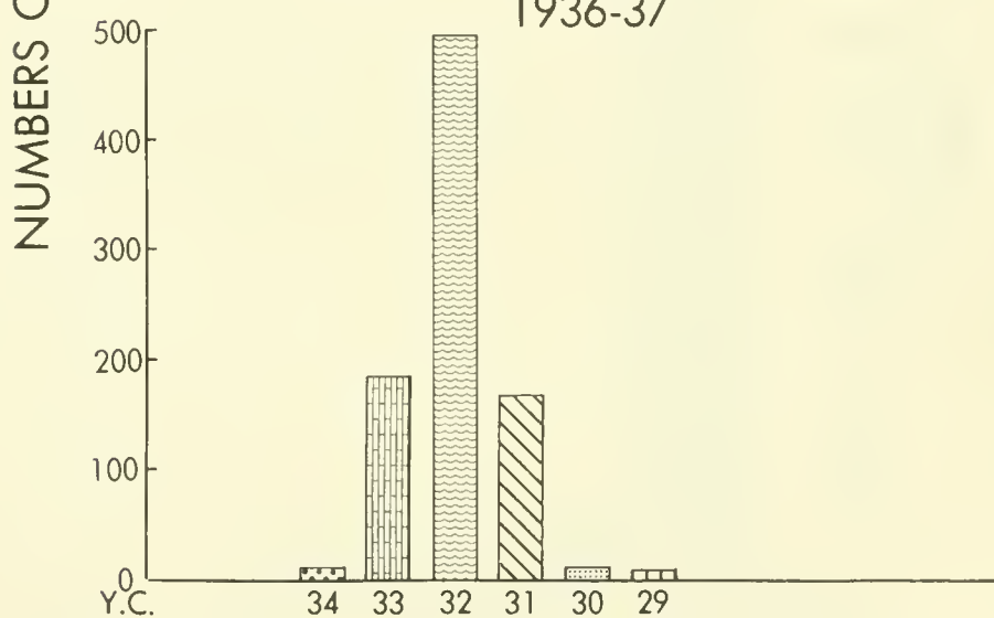
Figure 17.--Catch in millions of fish, by age and year class, for San Pedro for the seasons 1935-36 and 1936-37.
