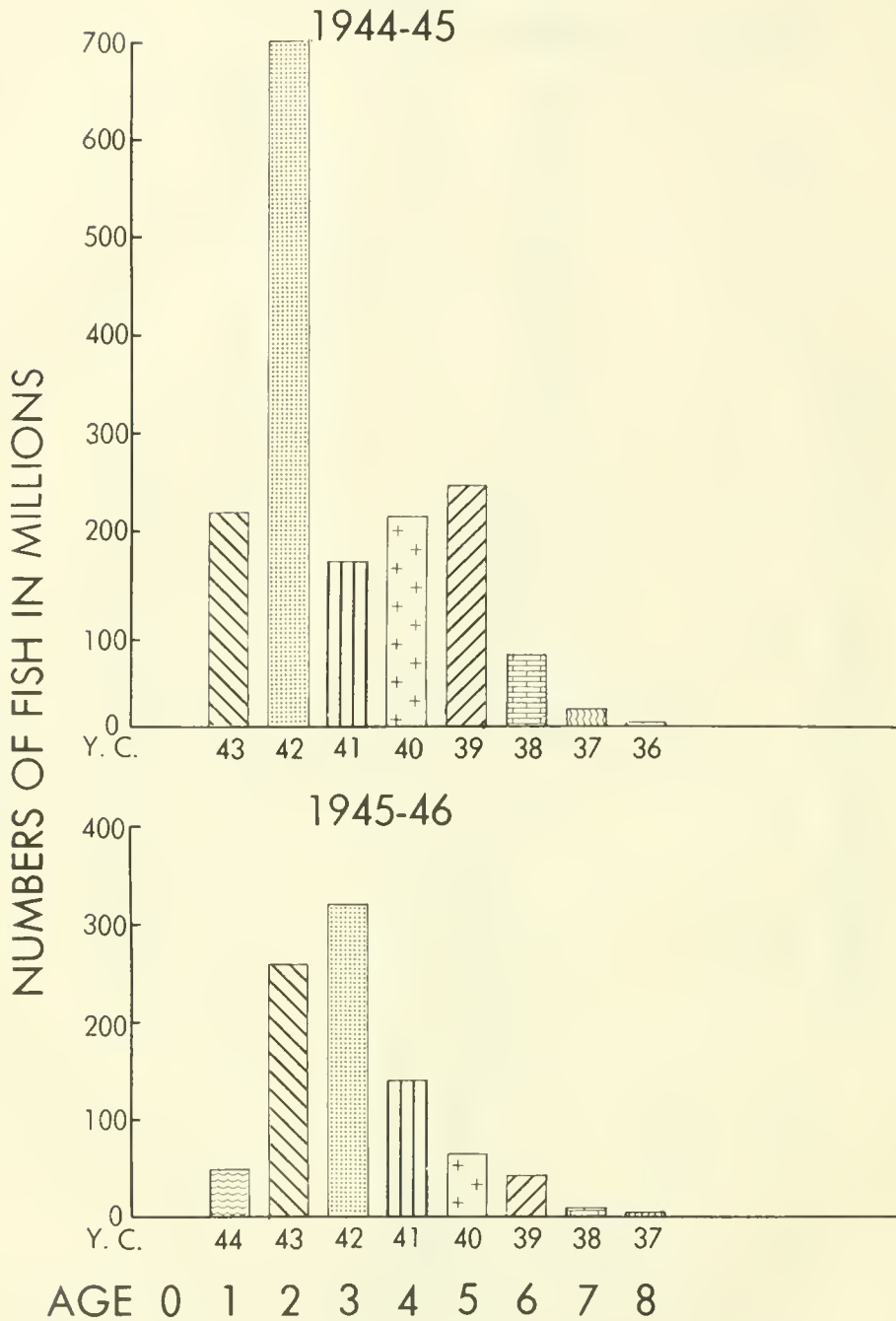
Figure 12.--Catch in millions of fish, by age and year class, for Monterey for the seasons 1944-45 and 1945-46.
