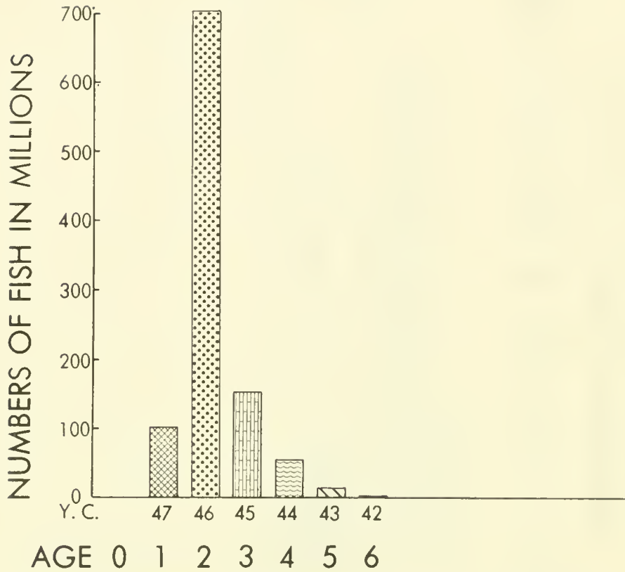
Figure 25.--Catch in millions of fish, by age and year class, for San Pedro for the season 1948-49.
