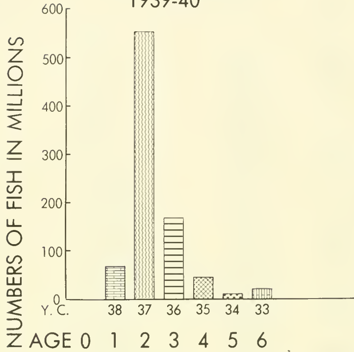
Figure 19.--Catch in millions of fish, by age and year class, for San Pedro for the season 1939-40.
