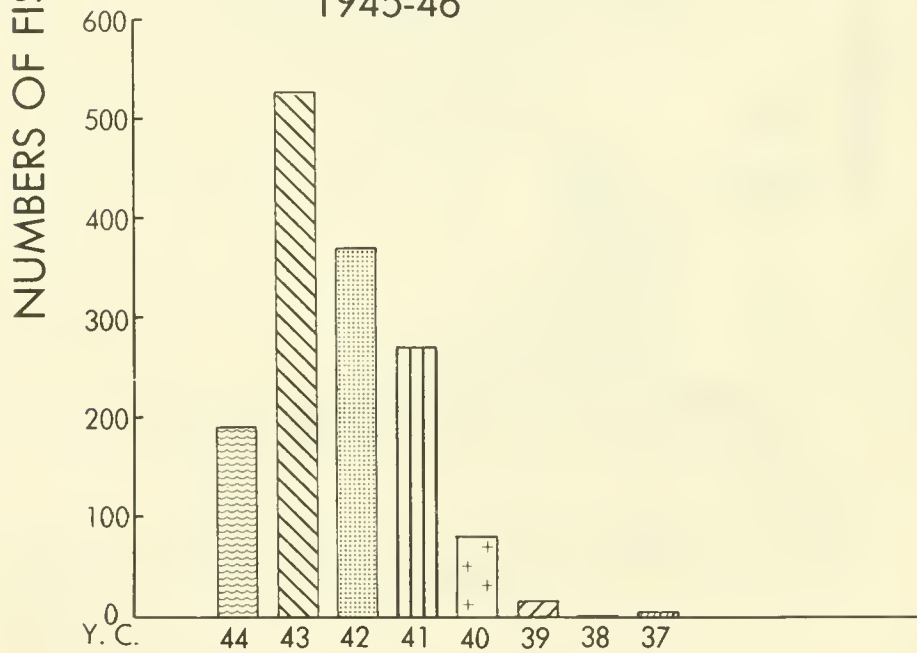
Figure 23.--Catch in millions of fish, by age and year class, for San Pedro for the seasons 1944-45 and 1945-46.
