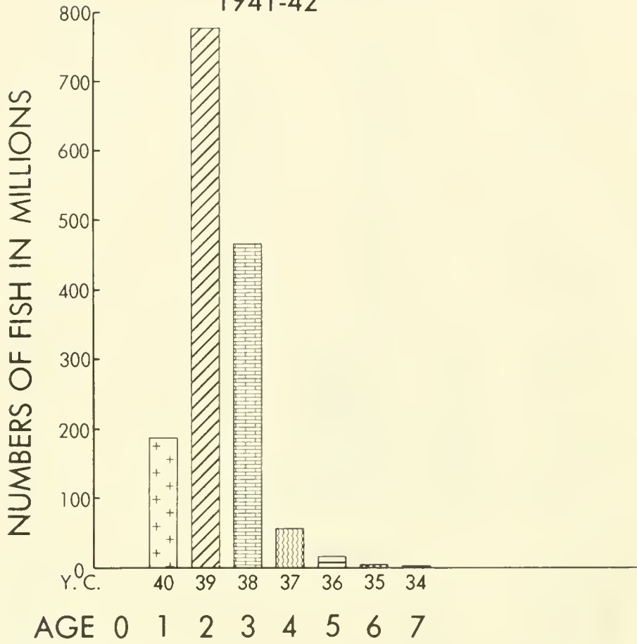
Figure 21.--Catch in millions of fish, by age and year class, for San Pedro for the season 1941-42.
