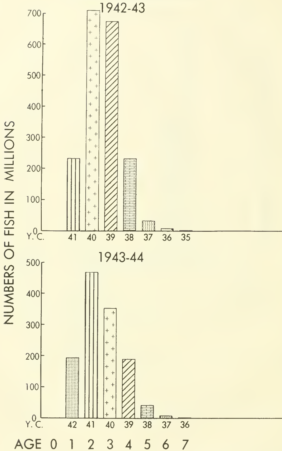
Figure 22.--Catch in millions of fish, by age and year class, for San Pedro for the seasons 1942-43 and 1943-44.
