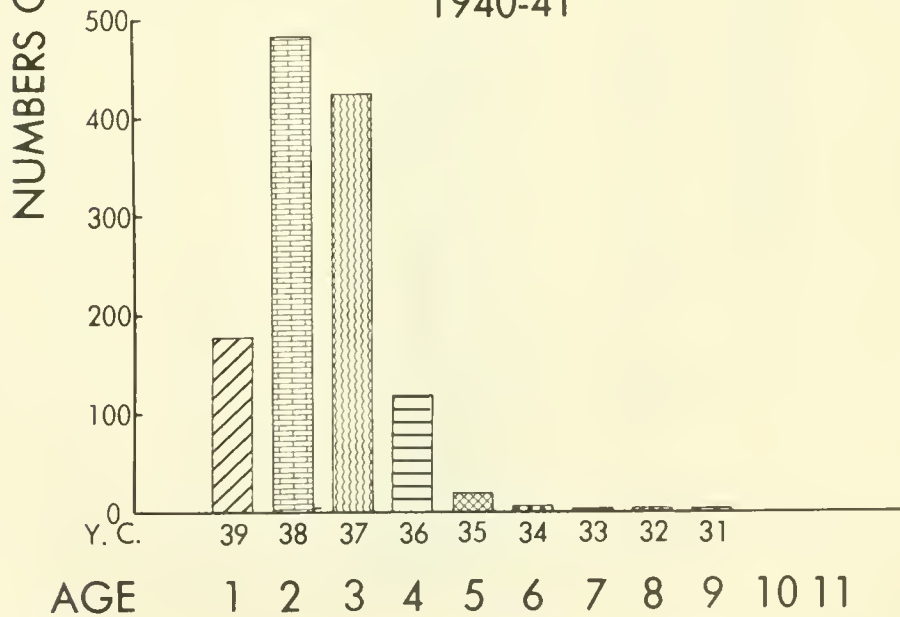
Figure 9.--Catch in millions of fish, by age and year class, for Monterey for the seasons 1939-40 and 1940-41.
