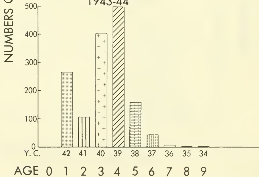
Figure 11.--Catch in millions of fish, by age and year class, for Monterey for the seasons 1942-43 and 1943-44.
