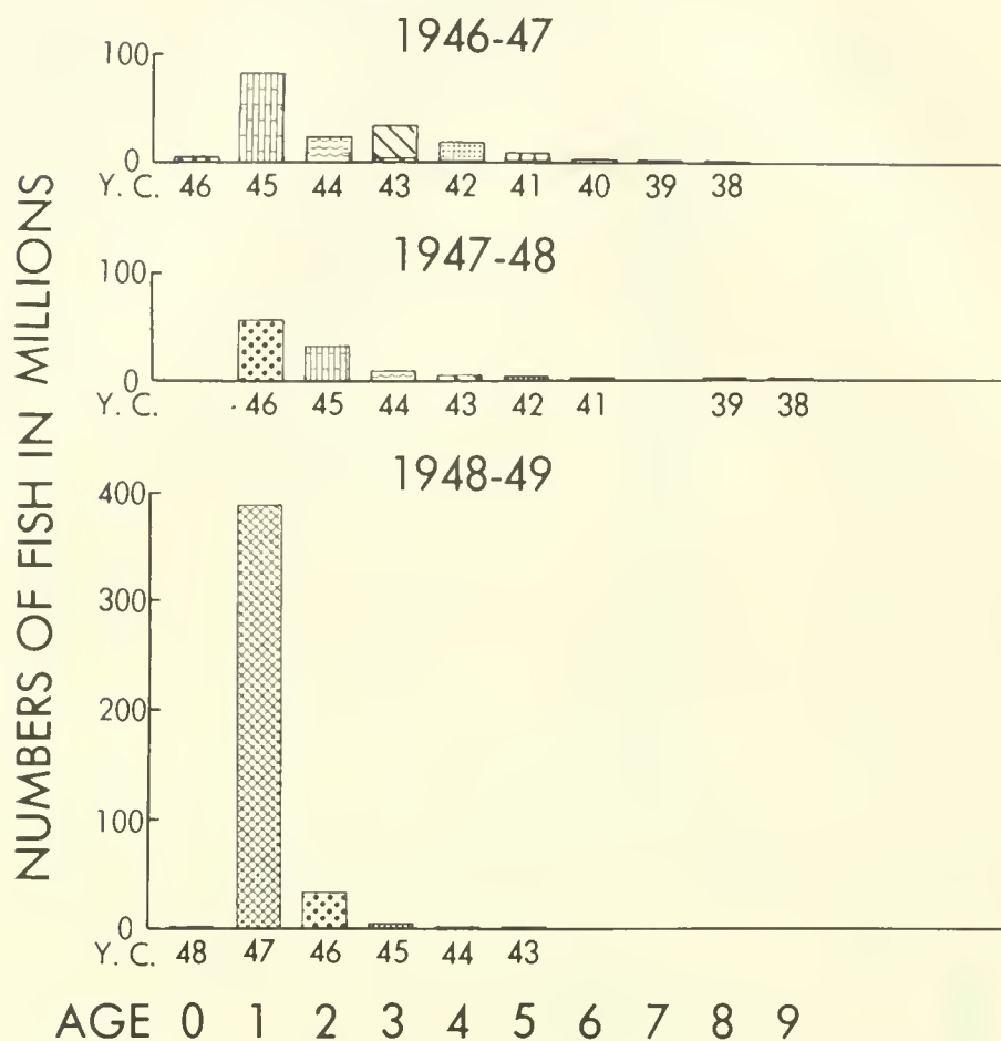
Figure 13.--Catch in millions of fish, by age and year class, for Monterey for the seasons 1946-47 through 1948-49.
