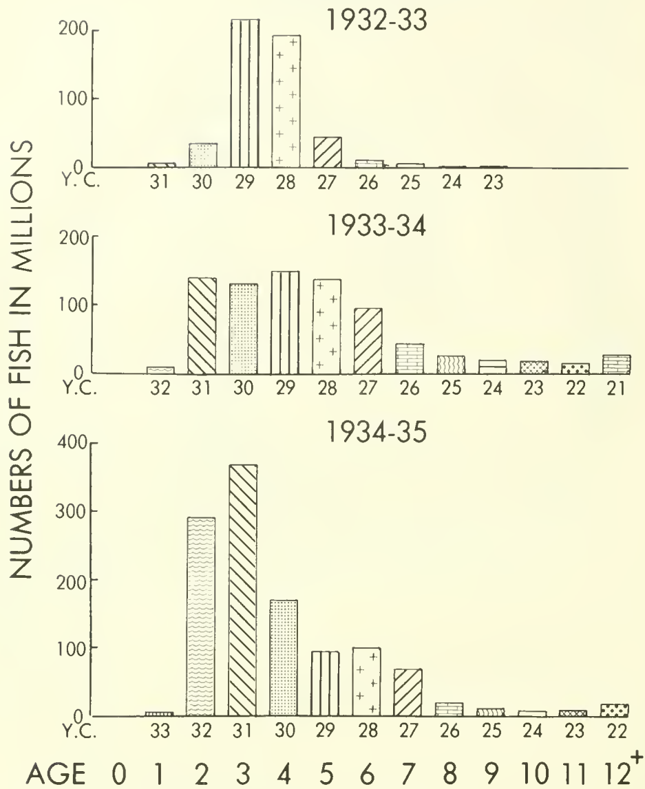
Figure 16.--Catch in millions of fish, by age and year class, for San Pedro for the seasons 1932-33 through 1934-35.
