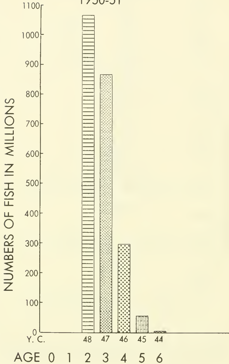
Figure 27.- Catch in millions of fish, by age and year class, for San Pedro for the season 1950-51.
