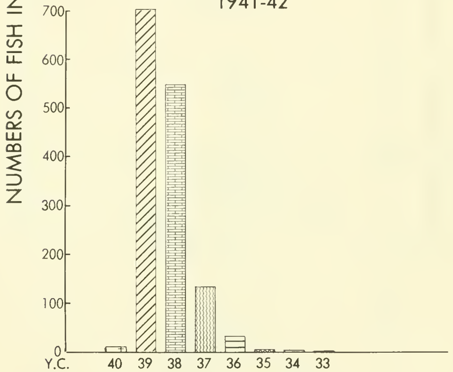
Figure 3.--Catch in millions of fish, by age and year class, for San Francisco for the seasons 1940-41 and 1941-42.
