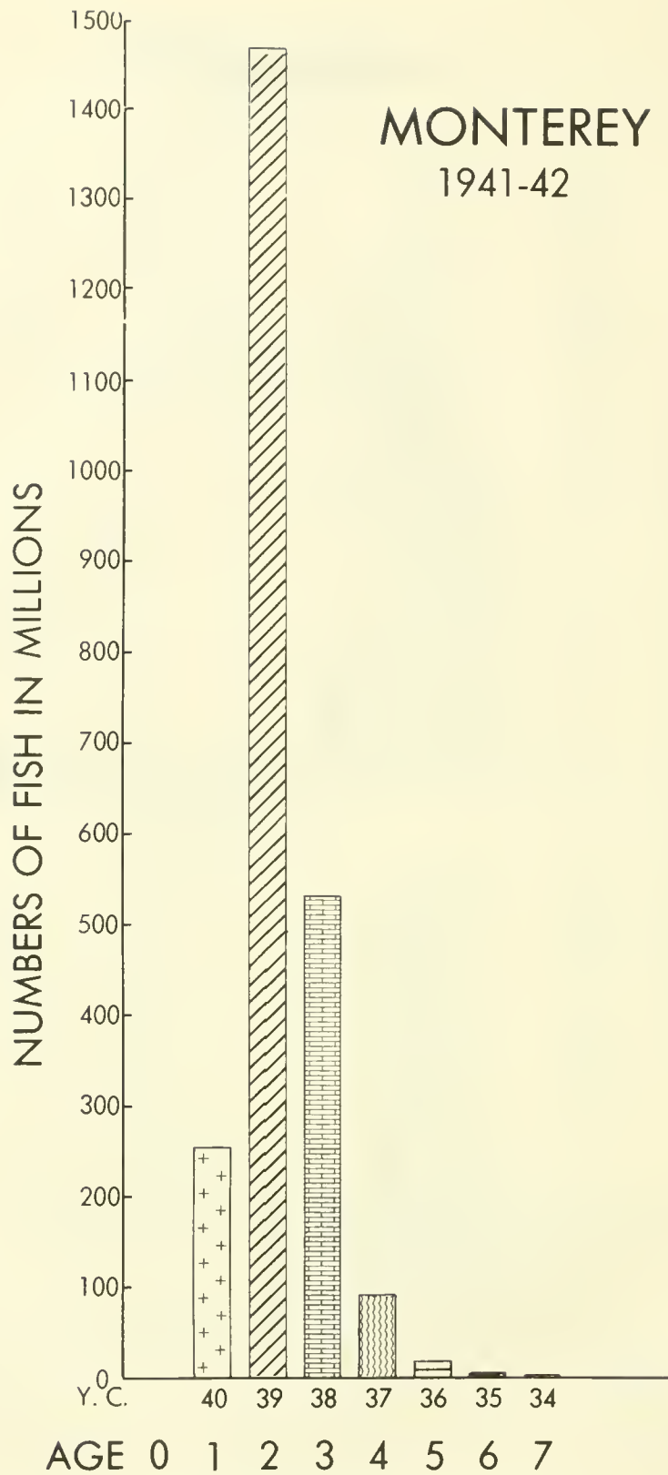
Figure 10.--Catch in millions of fish, by age and year class, for Monterey for the season 1941-42.
