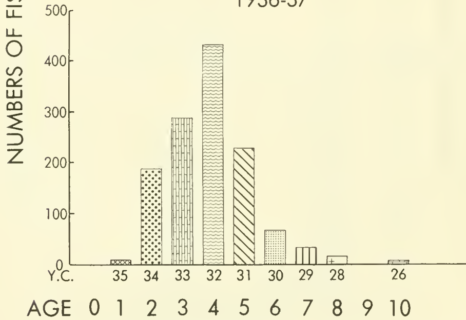
Figure 7.--Catch in millions of fish, by age and year class, for Monterey for the seasons 1935-36 and 1936-37.
