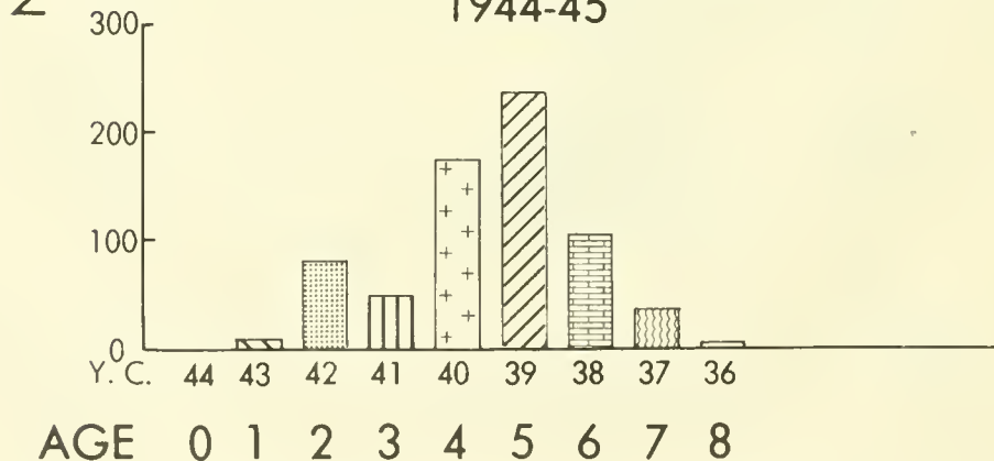
Figure 4.--Catch in millions of fish, by age and year class, for San Francisco for the seasons 1942-43 through 1944-45.
