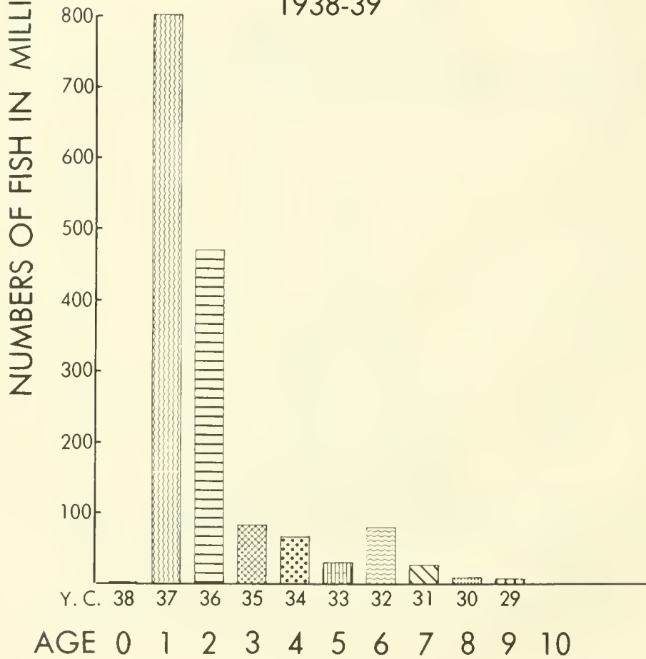
Figure 8.--Catch in millions of fish, by age and year class, for Monterey for the seasons 1937-38 and 1938-39.
