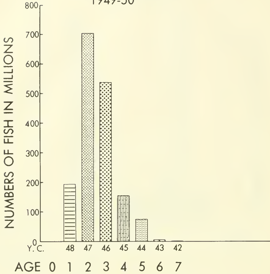
Figure 26.--Catch in millions of fish, by age and year class, for San Pedro for the season 1949-50.
