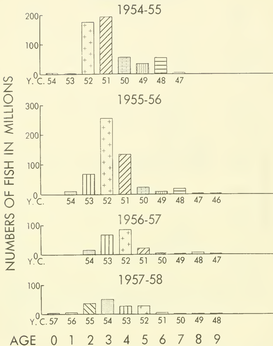
Figure 29.--Catch in millions of fish, by age and year class, for San Pedro for the seasons 1954-55 and 1955-56 and for southern California for the seasons 1956-57 and 1957-58.
