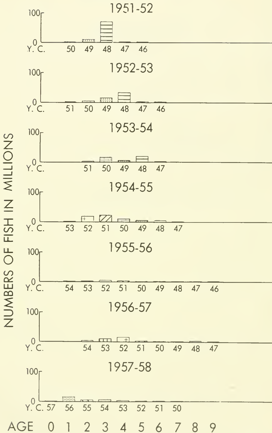
Figure 31.--Catch in millions of fish, by age and year class, for Ensenada for the seasons 1951-52 through 1955-56, and for Baja California for the seasons 1956-57 and 1957-58.
