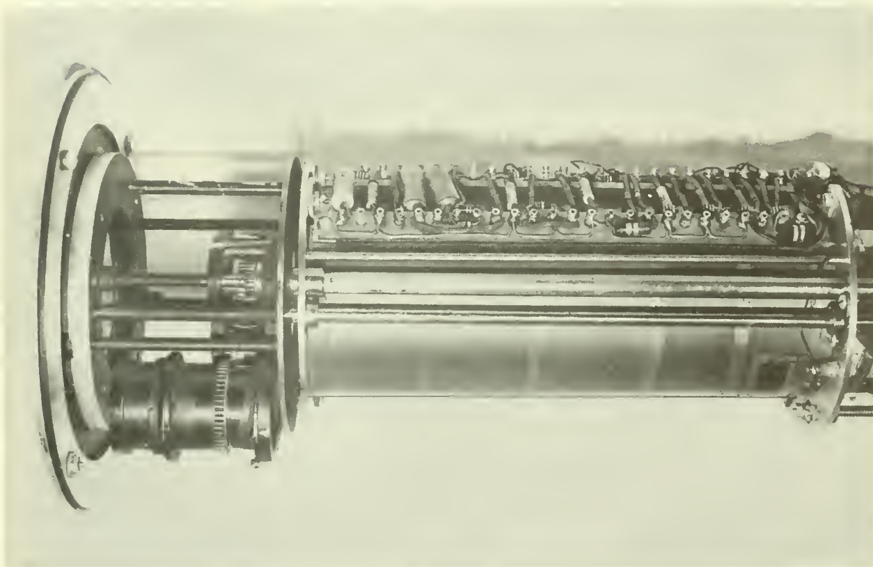
FIGURE A-3.--TELEVISION CAMERA DETAIL, SECTION A.
