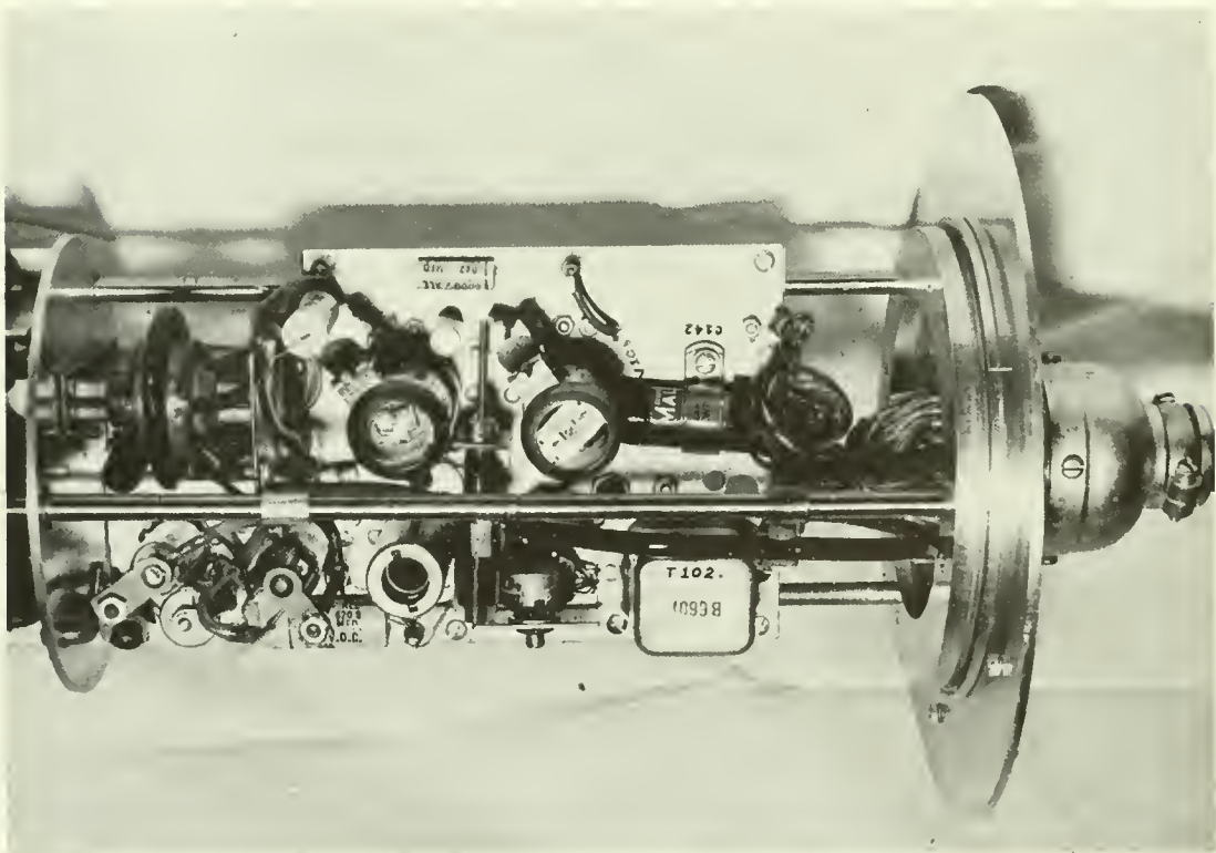
FIGURE A-7.--TELEVISION CAMERA DETAIL, SECTION E.
