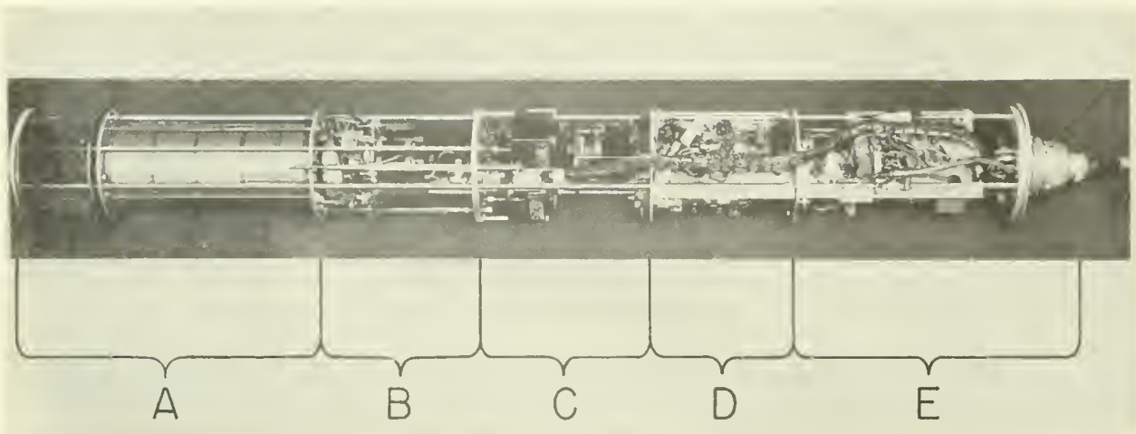
FIGURE A-2.--TELEVISION CAMERA, SECTIONS A-E.
