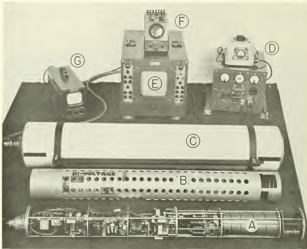
FIGURE 1.--COMPLETE IMAGE-ORTHICON TELEVISION CHAIN. INDIVIDUAL UNITS INCLUDE: (A) CAMERA, (B) PROTECTIVE SLEEVE, (C) WATERTIGHT HOUSING, (D) POWER SUPPLY AND VOLTAGE REGULATOR, (E) CAMERA CONTROL UNIT AND VIEWING MONITOR. THE OSCILLOSCOPE (F) AND SMALL MONITOR (G) ARE ACCESSORY EQUIPMENT.
