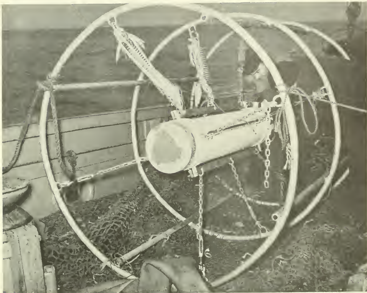
FIGURE 4.--CAMERA UNIT MOUNTED IN SUPPORTING FRAME USED IN COD END OBSERVATION WORK. (CAMERA LENS IS COVERED TO PROTECT THE PICKUP TUBE FROM EXPOSURE TO DIRECT SUNLIGHT).
