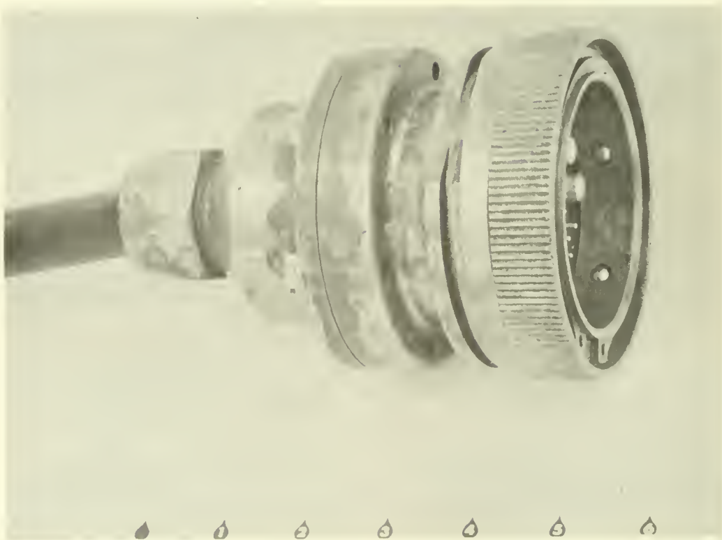
FIGURE A-1.--SPECIAL WATERTIGHT CONNECTOR DEVELOPED FOR USE WITH UNDERWATER TELEVISION.
