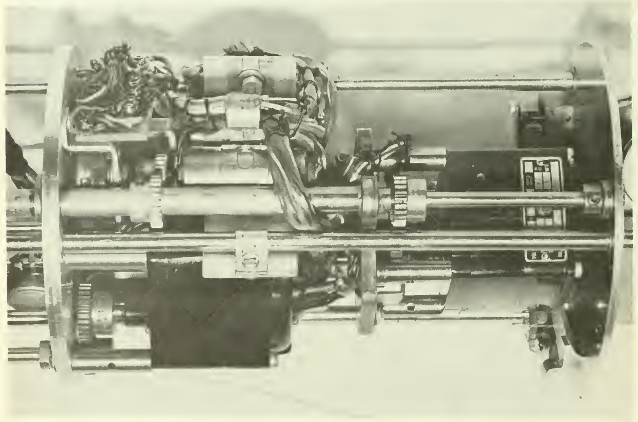
FIGURE A-5.--TELEVISION CAMERA DETAIL, SECTION C.
