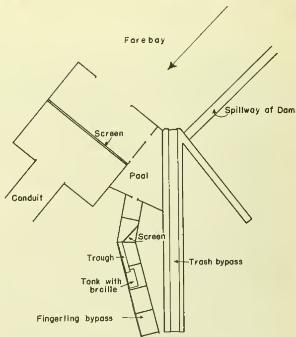
Figure 9.--Fingerling bypass at Tumwater Dam and trapping device.
