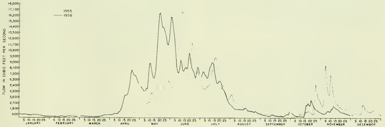
Figure 17.--Wenatchee River discharge at Plain, Washington.
