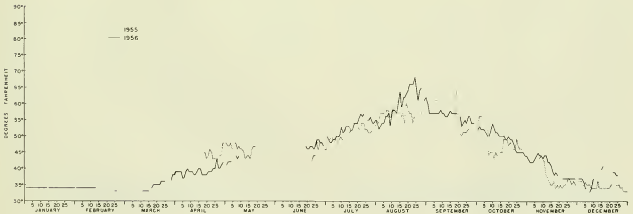
Figure 18.--Wenatchee River Water temperature at Tumwater Dam. (Hand thermometer)
