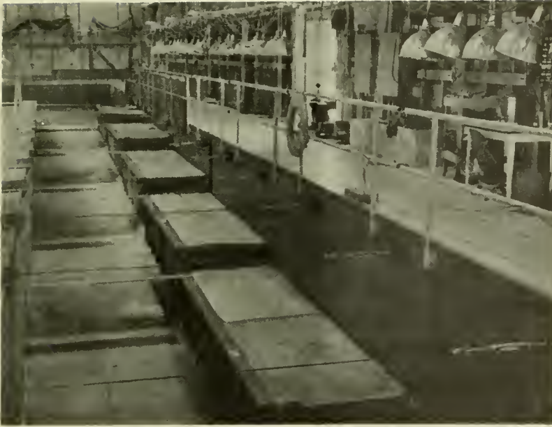
Figure 3.--The dark fishway (on right) showing plywood and canvas covering. Building interior was darkened during trials.
