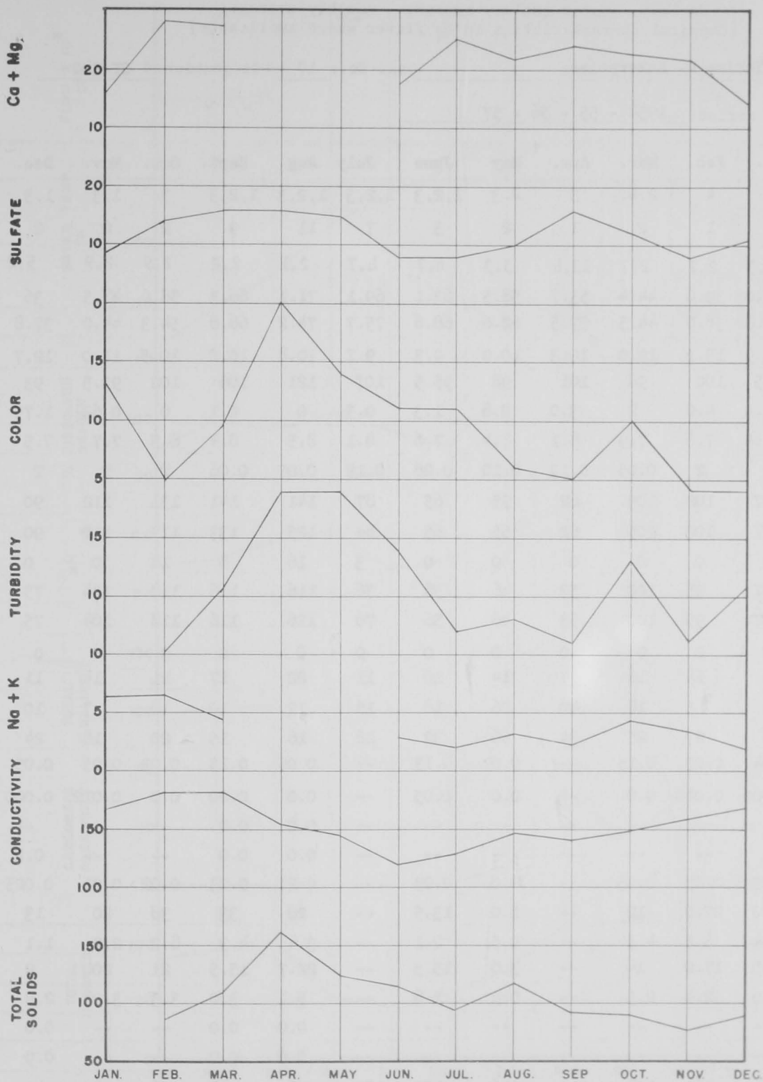
COLUMBIA RIVER AT PASCO Average Monthly Water Quality 1954 - 1957
