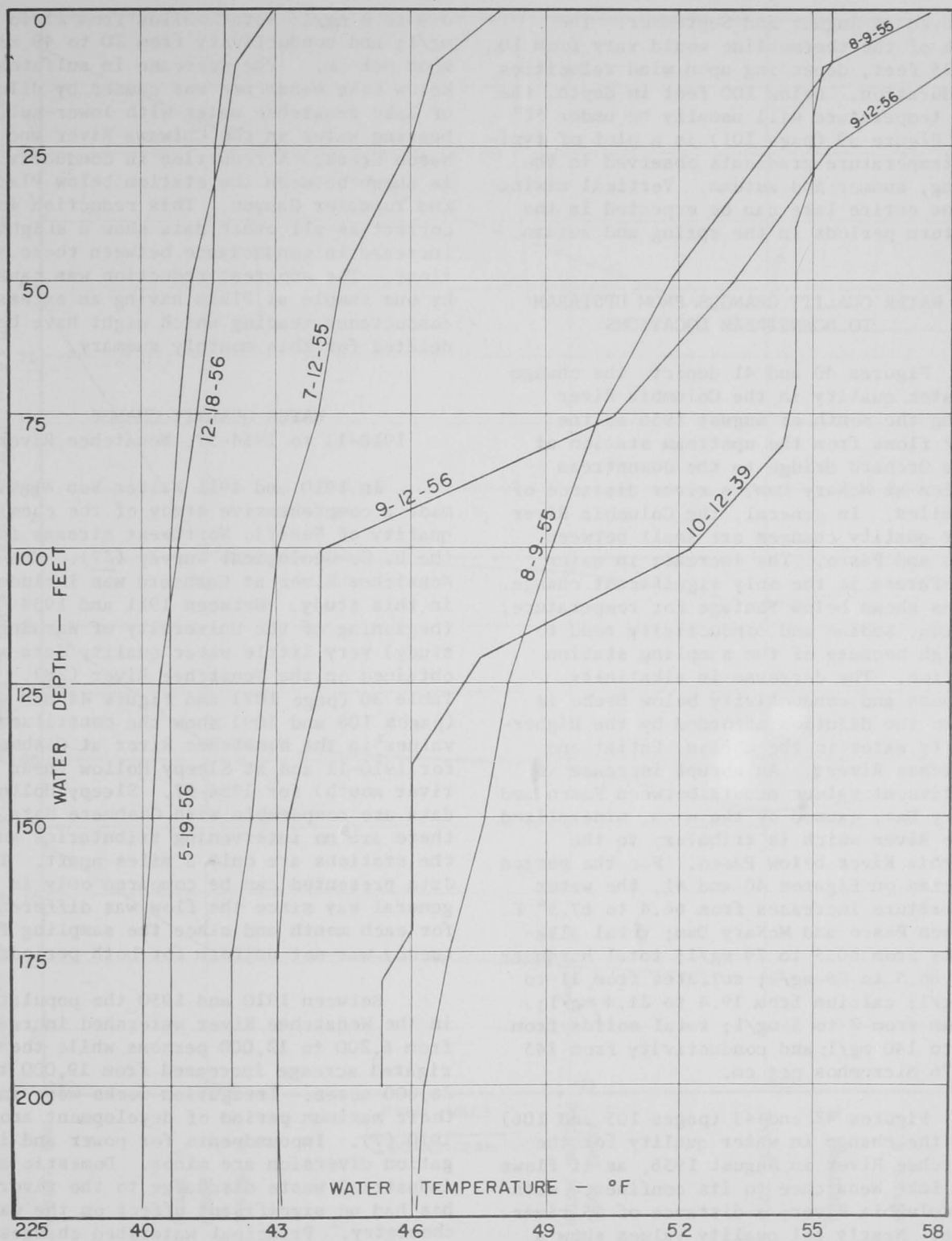
TYPICAL WATER TEMPERATURE GRADIENTS LAKE WENATCHEE, Station 42; 1939, 1955, 1956
