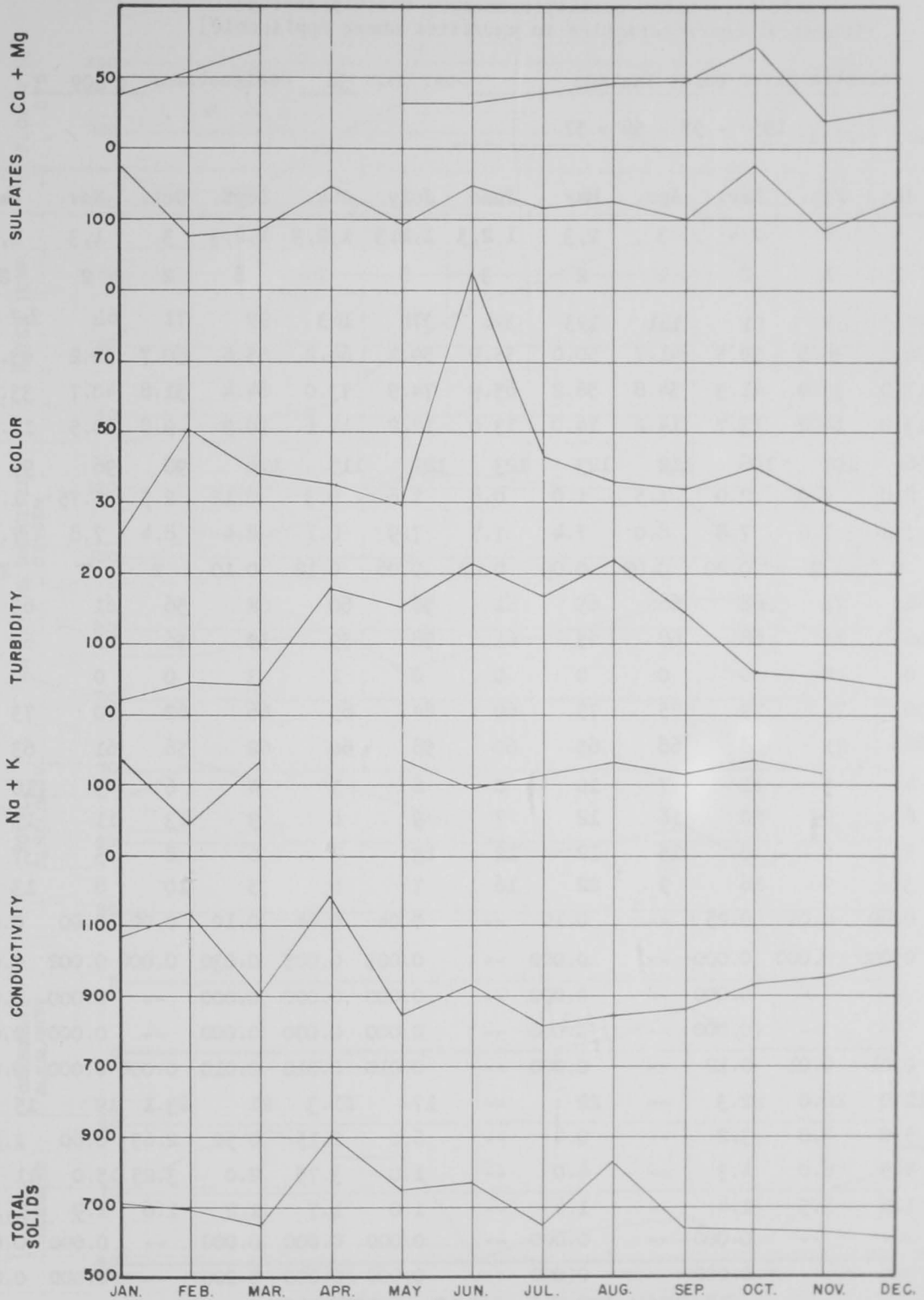
CRAB CREEK AT BEVERLY Average Monthly Water Quality 1954 - 1957
