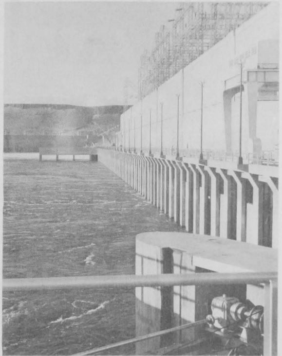
STA. 13 - COLUMBIA RIVER AT McNARY DAM
