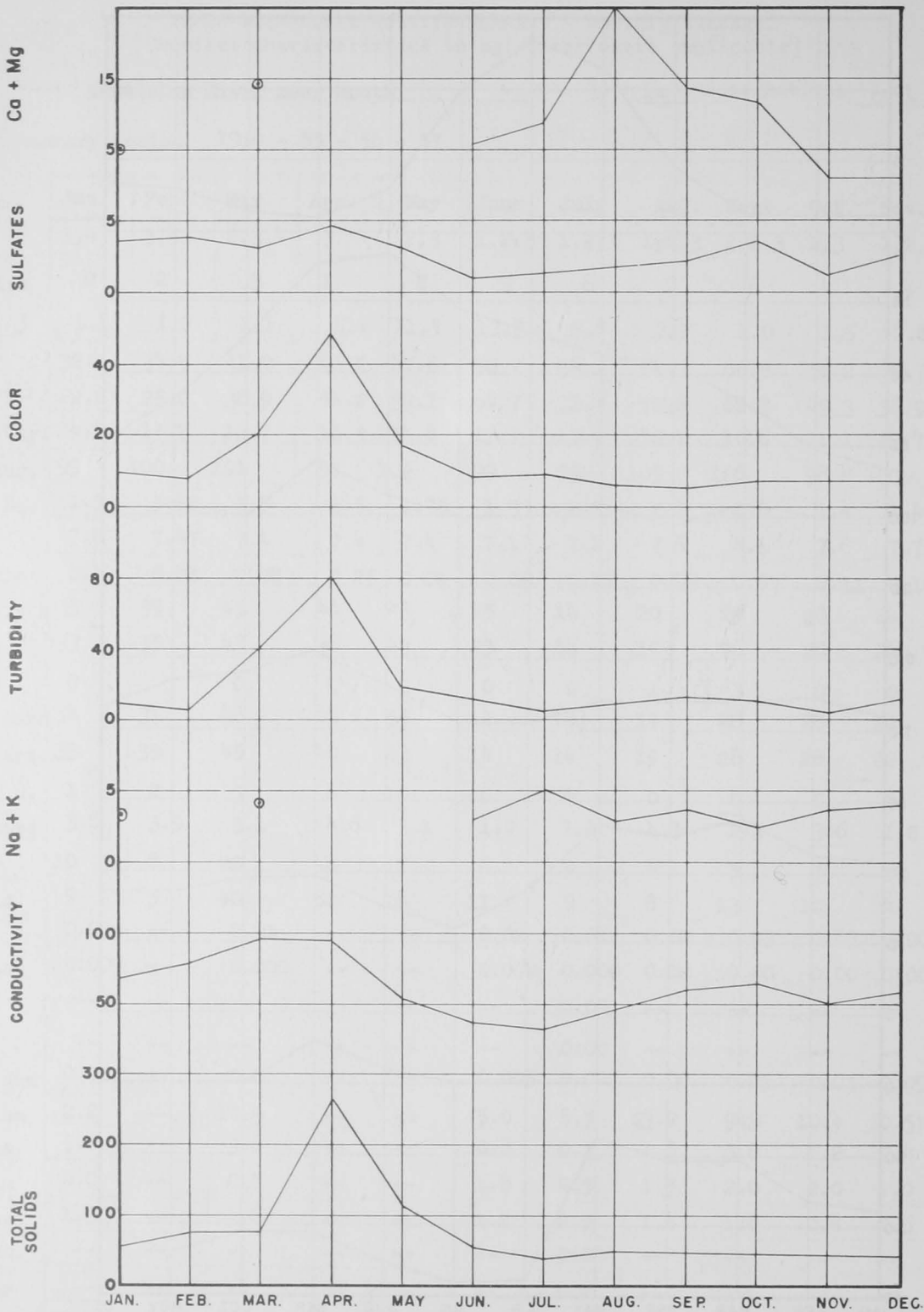
WENATCHEE RIVER NEAR MOUTH Average Monthly Water Quality 1954-1957
