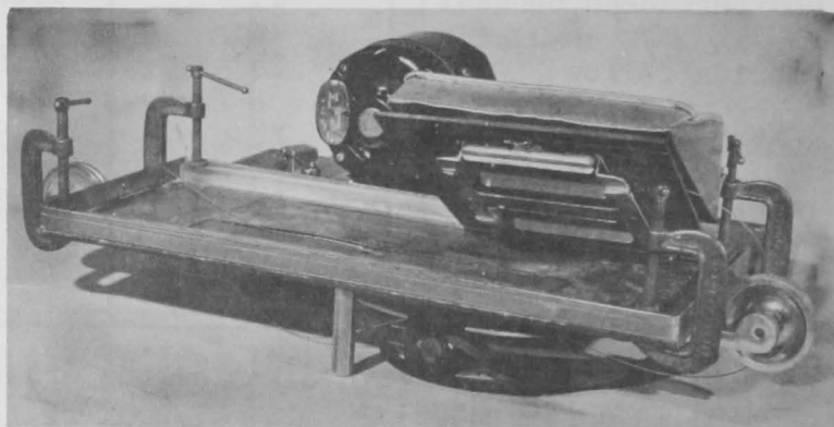
Figure 11.—Abrasion test equipment
