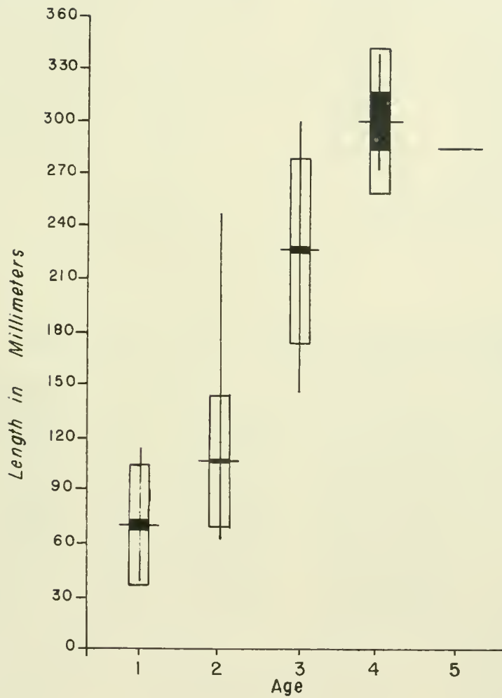
Figure 18. - Maximum, minimum, and average lengths of each age group of downstream-migrant bluebacks, 1949-53 average. White boxes represent two standard deviations on each side of the mean; black boxes represent 95-percent confidence limits of the mean.
