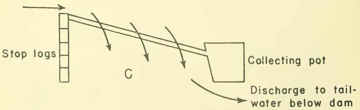
Figure 3 - Diagrammatic drawing of an auxiliary-water screen pit showing positions of fingerling bypasses and fingerling traps.
