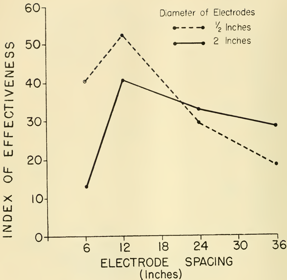
Figure 13.--Effect of electrode spacing in relation to electrode diameter using a width of electrical field of 2 feet at a 40° angle of electrical field with a voltage gradient of 1 volt/cm., a pulse frequency of 8 pulses/sec., a pulse duration of 40 milliseconds, and a square wave form.
