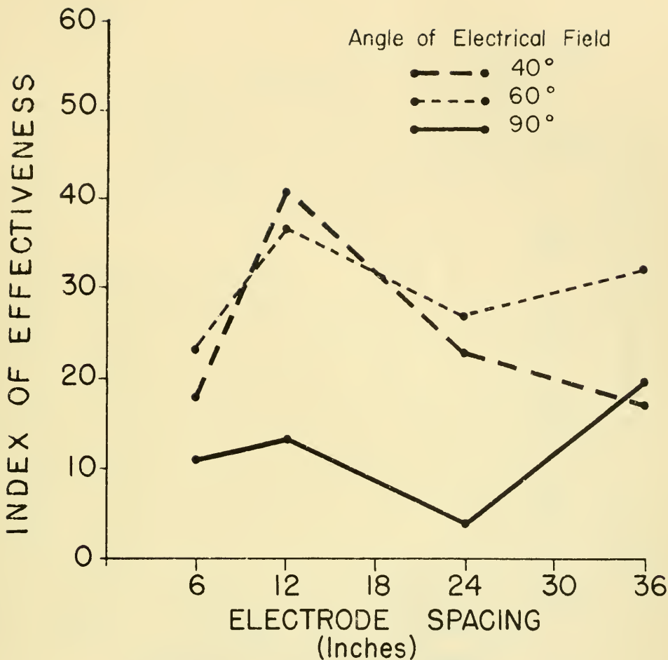
Figure 11.--The effect of electrode spacing in relation to the angle of electrical field using 2-inch electrodes at a width of electrical field of 3 feet with a voltage gradient of 1 volt/cm., a pulse frequency of 8 pulses/sec., a pulse duration of 40 milliseconds, and a square wave form.
