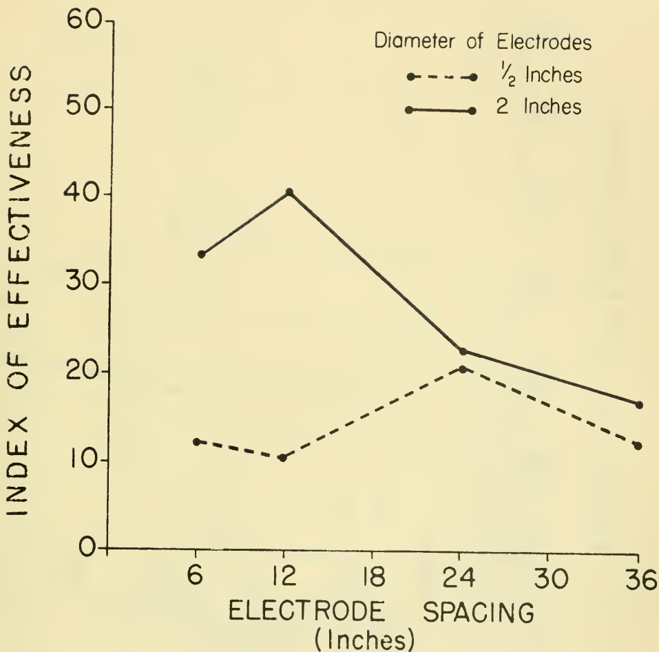
Figure 14.--Effect of electrode spacing in relation to electrode diameter using a width of electrical field of 3 feet at a 40^\circ angle of electrical field with a voltage gradient of 1 volt/cm., a pulse frequency of 8 pulses/sec., a pulse duration of 40 milliseconds, and a square wave form.
