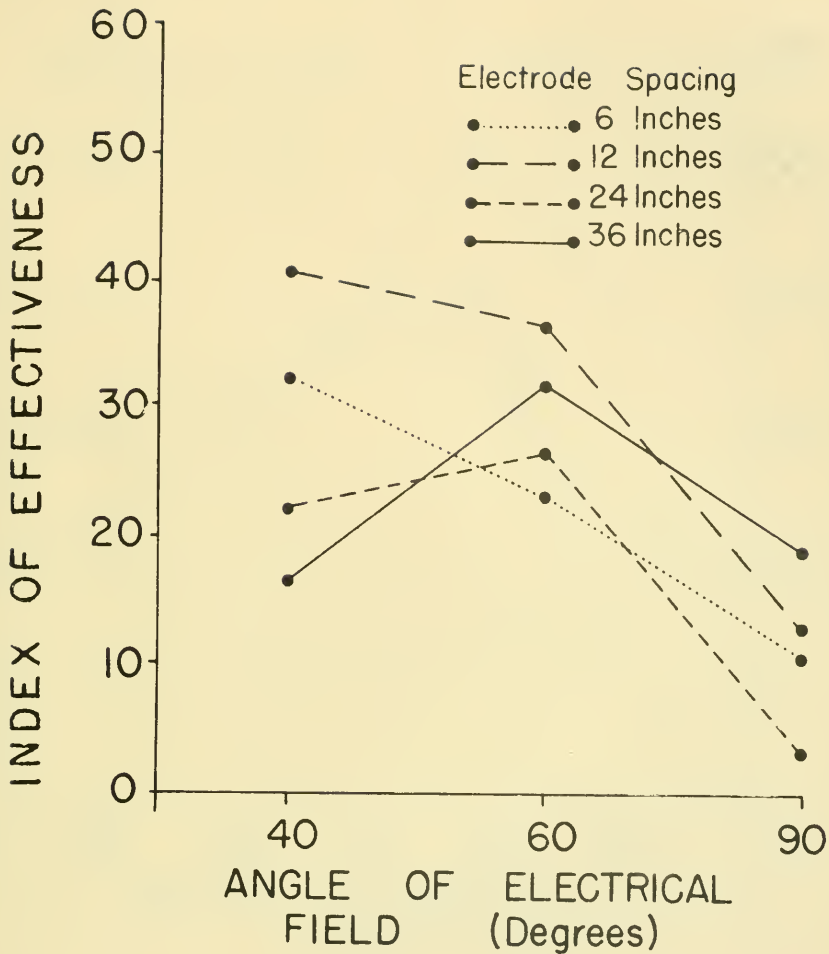
Figure 12.--The effect of the angle of electrical field in relation to electrode spacing using 2-inch electrodes at a width of electrical field of 3 feet with a voltage gradient of 1 volt/cm., a pulse frequency of 8 pulses/sec., a pulse duration of 40 milliseconds, and a square wave form.
