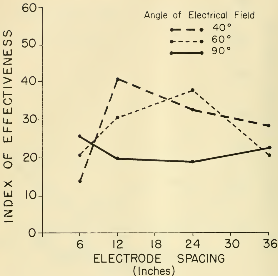
Figure 9.--The effect of electrode spacing in relation to the angle of electrical field using 2-inch electrodes at a width of electrical field of 2 feet with a voltage gradient of 1 volt/cm., a pulse frequency of 8 pulses/sec., a pulse duration of 40 milliseconds, and a square wave form.
