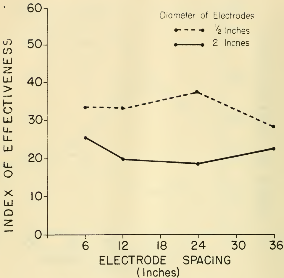
Figure 15.--Effect of electrode spacing in relation to electrode diameter using a width of electrical field of 2 feet at a 90° angle of electrical field with a voltage gradient of 1 volt/cm., a pulse frequency of 8 pulses/sec., a pulse duration of 40 milliseconds, and a square wave form.
