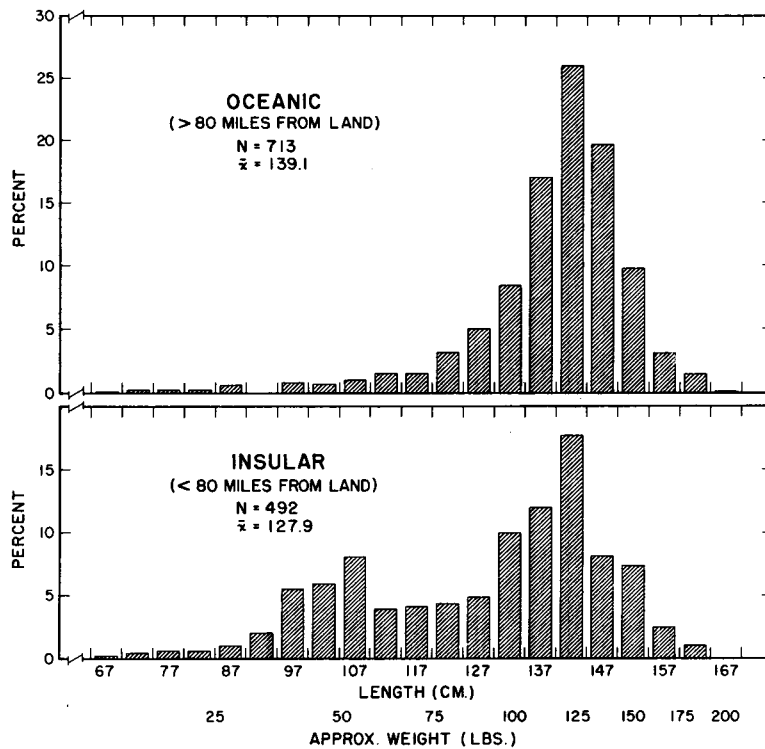
Figure 7. --Yellowfin size distribution with distance from land (data in appendix table 14).
