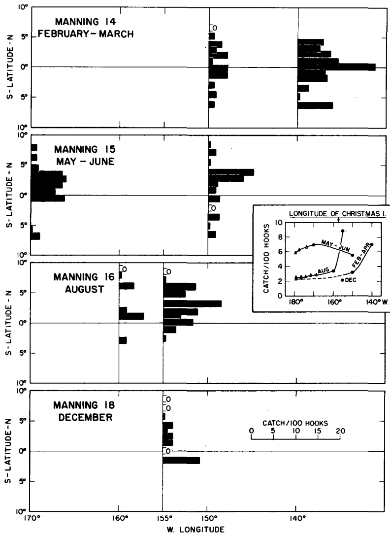
Figure 2. --Temporal and spatial distribution of long-line catches of yellowfin made during 1953 at stations more than 80 miles from land (data from appendix tables 6-11). Insert--diagrammatic representation of longitudinal variation in abundance (data from figs. 2 and 3). The round dots represent POFI data and the triangles represent Japanese data.
