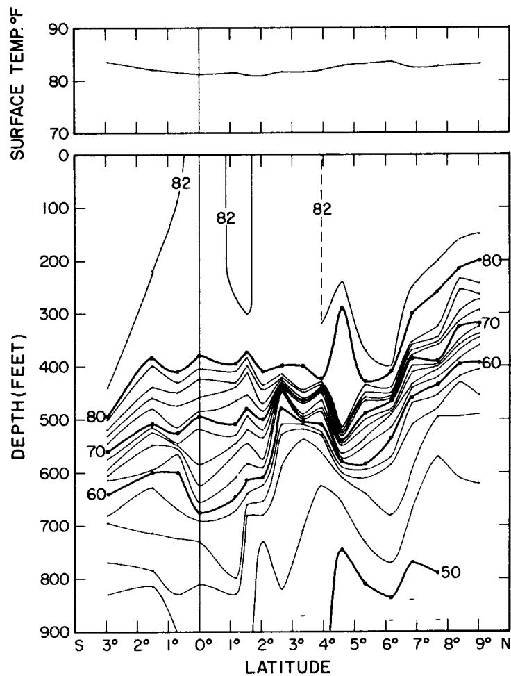
Figure 18.--Surface temperatures and vertical temperature section along 160^{\circ} W. longitude, August 1953 ( Manning cruise 16). Upper panel--surface temperatures as read at each bathythermograph lowering. Lower panel--temperature section based on bathythermograph lowerings; isotherms at 2^{\circ} F. intervals, depth of lowering shown by small horizontal dashes.
