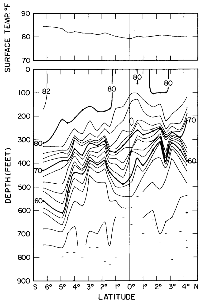
Figure 13. --Surface temperatures and vertical temperature section along 140^{\circ}\text{W} . longitude, March 1953 ( Manning cruise 14). Upper panel--surface temperatures as read at each bathythermograph lowering. Lower panel--temperature section based on bathythermograph lowerings; isotherms at 2^{\circ}\text{F} . intervals, depth of lowering shown by small horizontal dashes.
