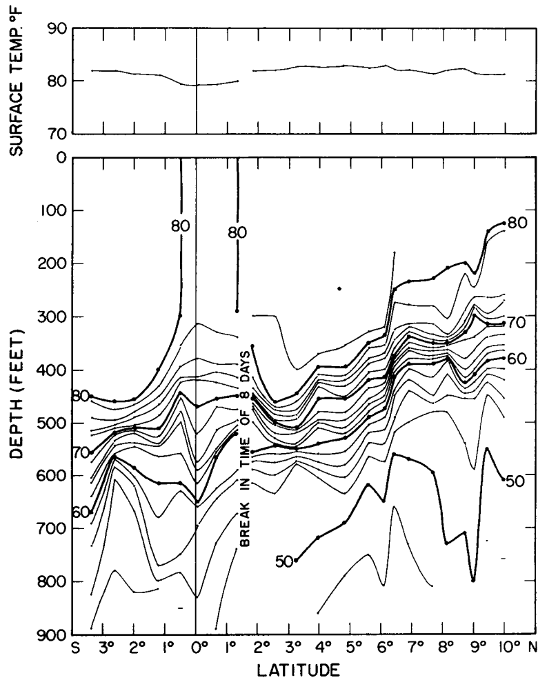
Figure 17.--Surface temperatures and vertical temperature section along 155^{\circ} W. longitude, August 1953 (Manning cruise 16). Upper panel--surface temperatures as read at each bathythermograph lowering. Lower panel--temperature section based on bathythermograph lowerings; isotherms at 2^{\circ} F. intervals, depth of lowering shown by small horizontal dashes.
