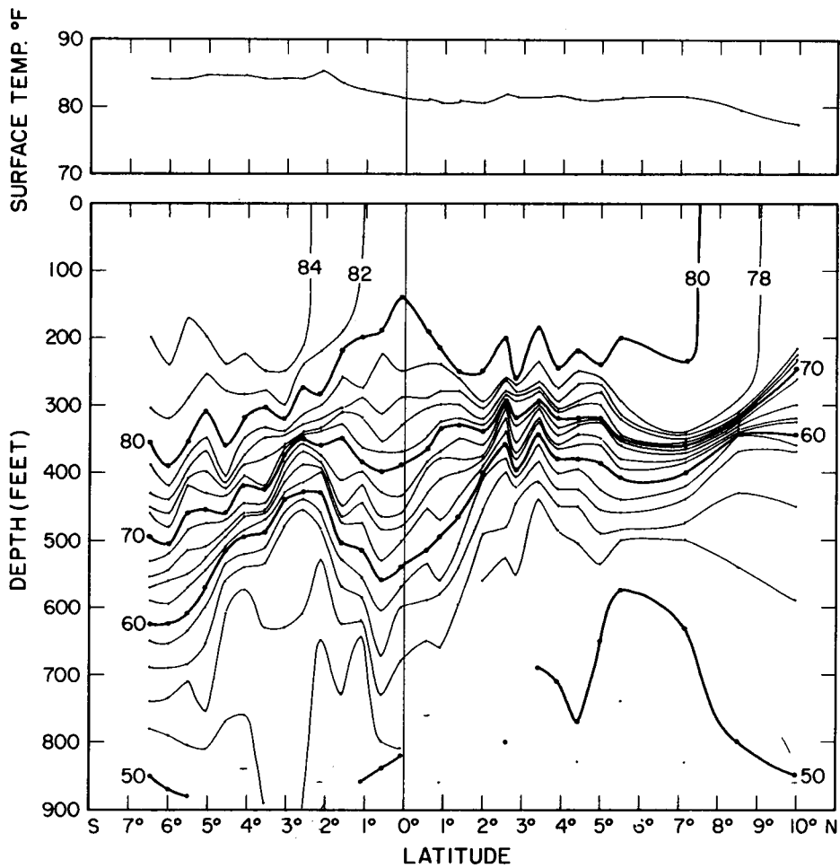
Figure 15. --Surface temperatures and vertical temperature section along 150^{\circ}\text{W} . longitude, May 1953 ( Manning cruise 15). Upper panel--surface temperatures as read at each bathythermograph lowering. Lower panel--temperature section based on bathythermograph lowerings; isotherms at 2^{\circ}\text{F} . intervals, depth of lowering shown by small horizontal dashes.
