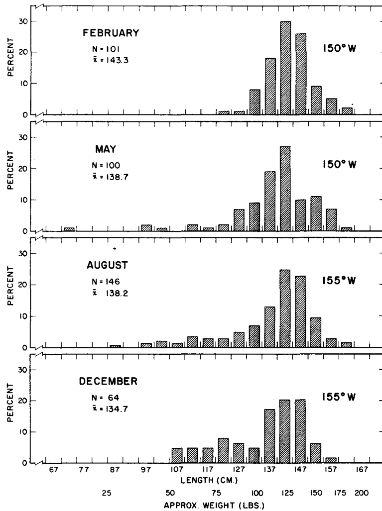
Figure 9.--Yellowfin size distribution by time of year at 150°-155°W. longitude (data in appendix table 14).
