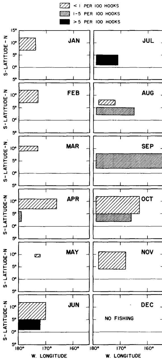
Figure 3.--Japanese commercial yellowfin catches in the central Pacific in 1953 (data from appendix table 12). The rectangles indicate the areas fished and the code indicates the catch rates.
