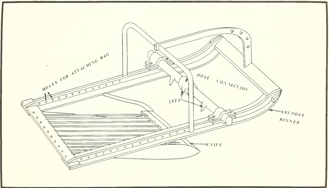
Figure 3.—“Long Island” hydraulic bar clam dredge of the type which became popular with the Long Island clambers. (Drawn by Carl Rich after C. E. Petite and P. W. G. McMullon, Fish. Res. Board Can., Bull. 102, Ottawa, 1955.)
