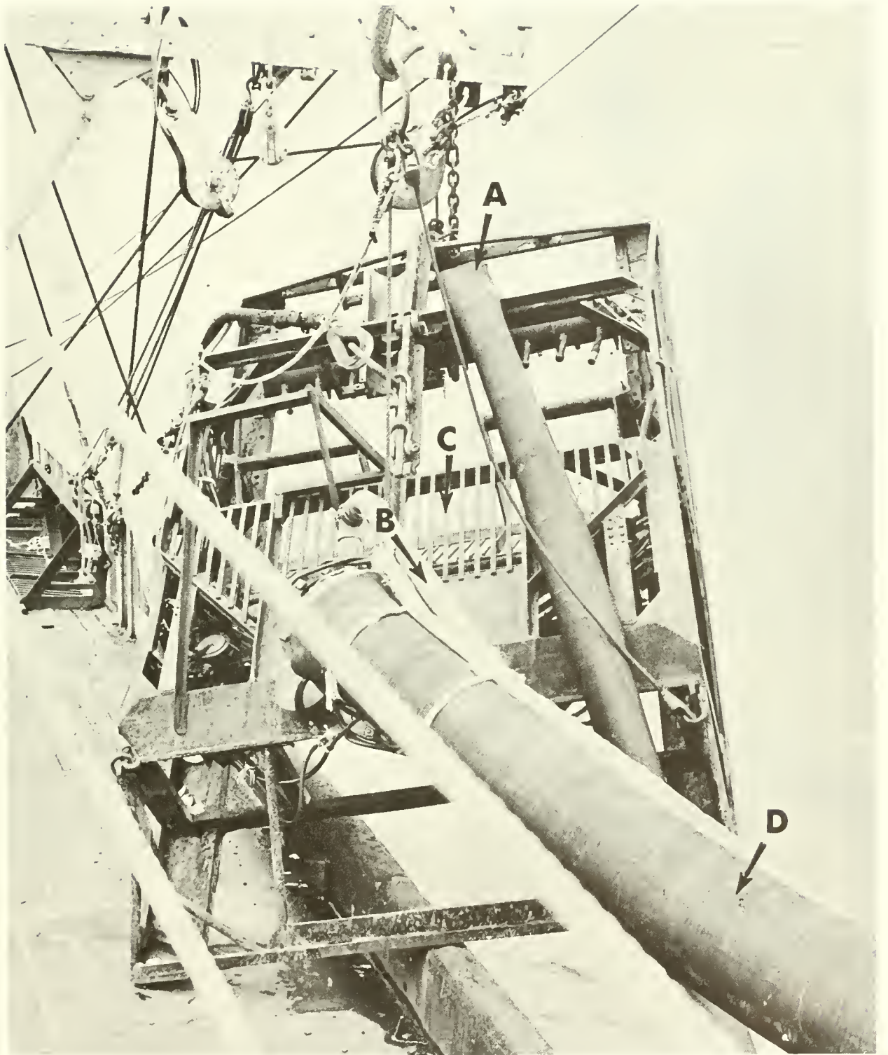
Figure 10.—Constant delivery pump system dredge aboard the Gail Borden . A — Clam jetting water supply hose. B — Compressed air hose. Air is supplied through this hose to the uptake unit where it mixes with the water in the hose, generating the upward movement of water within the hose. C — Receiver. Material jetted out of bottom and picked up by the dredge knife passes into this area and then into the uptake of the discharge hose. D — Transporting hose for carrying dredge material from receiver to separator.
