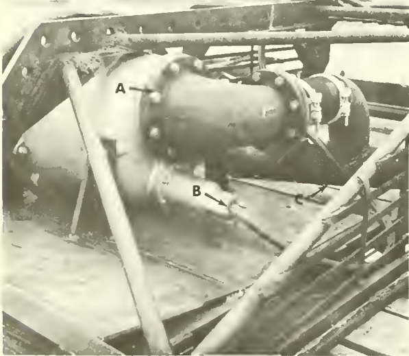
Figure 12.—Electrical submersible pump shown as mounted to 48-inch clam dredge. A — 8-inch discharge, connected to header. B — Watertight electrical junction. C — Header.
