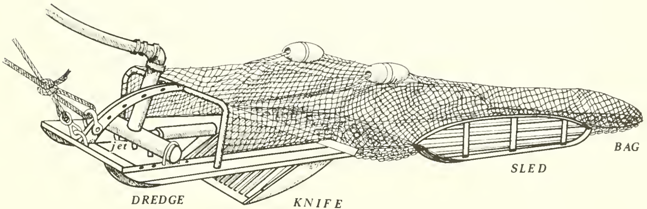
Figure 4.—Early model hydraulic dredge showing sled under bag, one of the early modifications which led to the development of the standard dredge with its after-cage built of steel bars.
