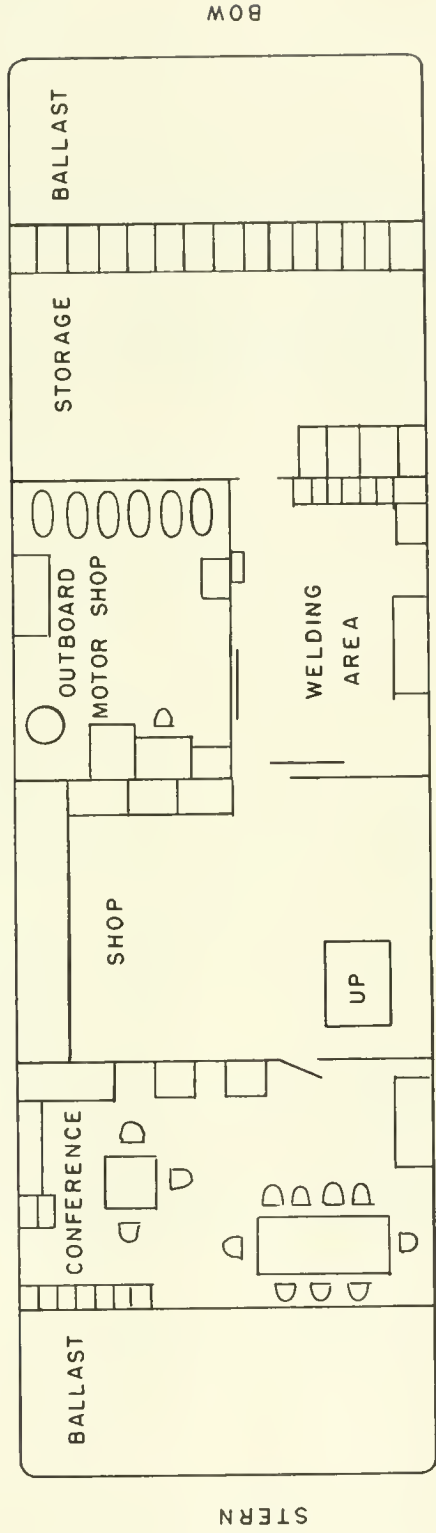
LOWER DECK
