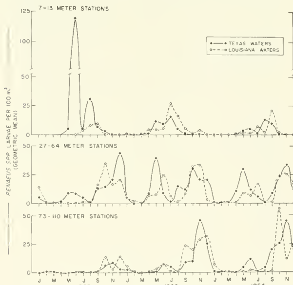
Figure 1.--Abundance of Penaeus larvae by depth zones in Louisiana and Texas waters, 1962-64.
