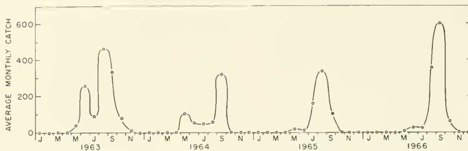
Figure 14.--Abundance of postlarval white shrimp, Sabine Pass, Tex., 1963-66. Open circles represent averages of four tows per month.
