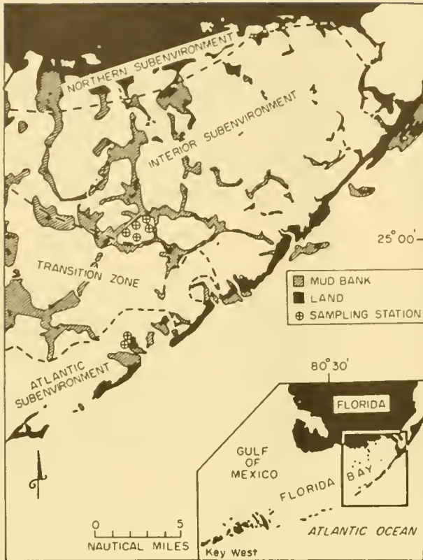
Figure 10.--Subenvironments in Florida Bay.
