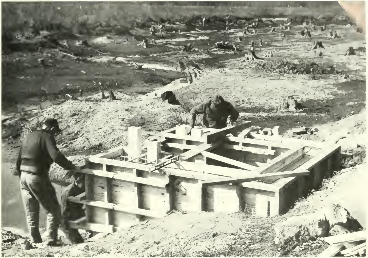
The conversion of wooded land, marginal for agricultural or industrial use, to highly productive wildlife habitat has been demonstrated by biologists at the Patuxent Center. Such areas may be cleared, partly cleared, or left with trees standing. Water levels in the impoundment are regulated by a control structure (above) to permit drawdown for maximum food-plant development, removal of rough fish, or for other purposes (below, left). Such a development showing impounded water, woody cover, and installed, predator-proofed, wood duck nesting boxes (below, right). (Photos by Frederick C. Schmid, top and lower left; Lee E. Yeager, bottom right)
