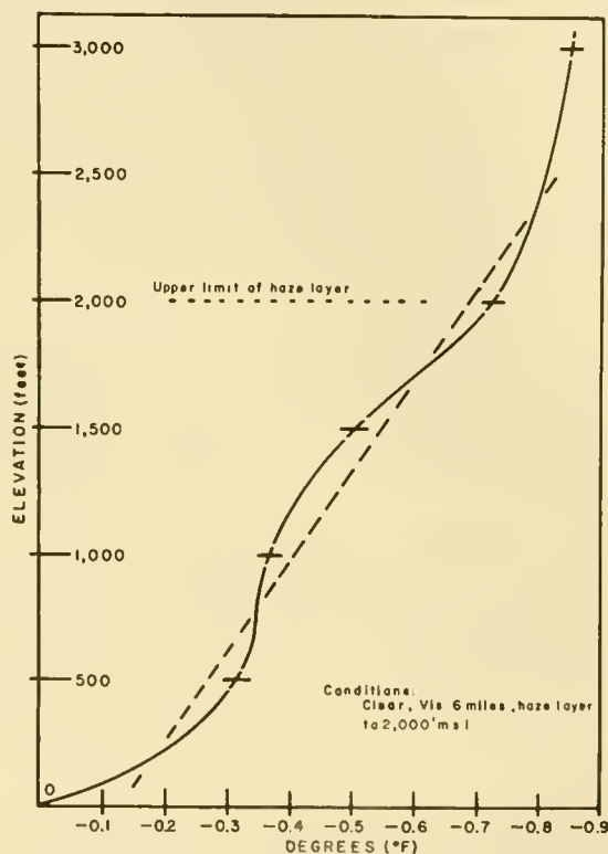
Figure 1. Haze effect observations; November 21, 1962; 1348-1447 P.S.T.; North San Francisco Bay
