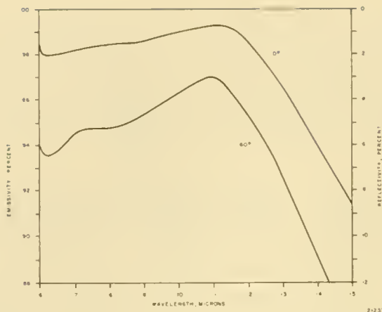
Figure 3. Spectral Emissivity of Ocean Surface at Normal Incidence and 60° from Normal
