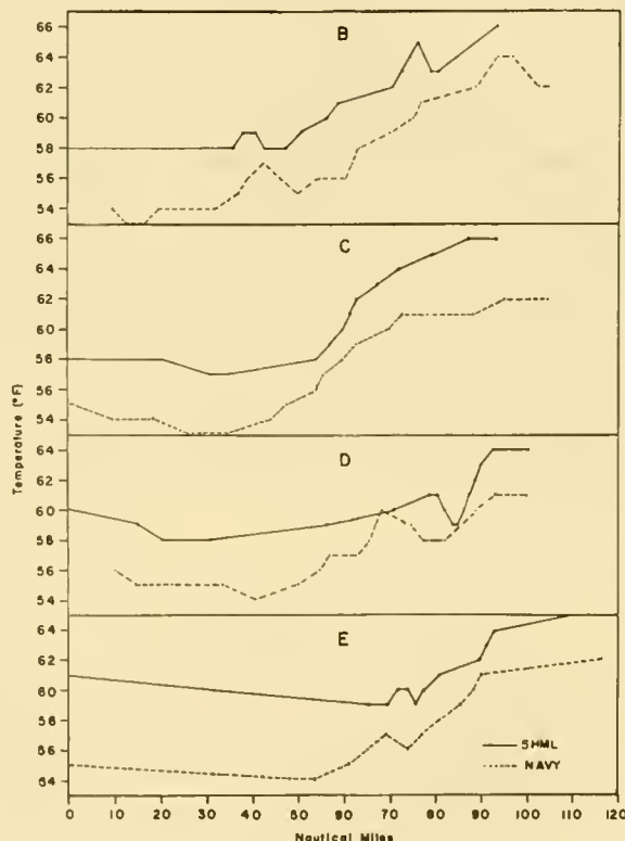
Figure 2. Temperatures from Sandy Hook - Navy comparative flight for transects B-E, September 30, 1963
