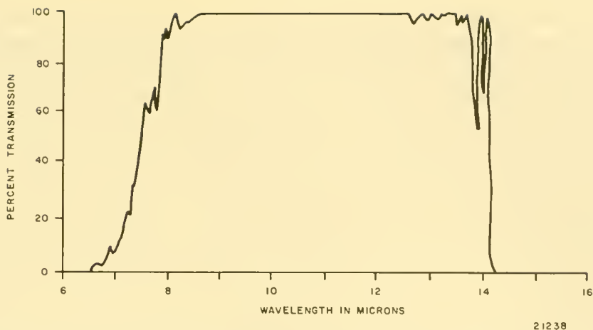
Figure 4. Transmission of Atmosphere (Sea Level, 1000 Feet Path, 0.1 cm Precipitable Water)
