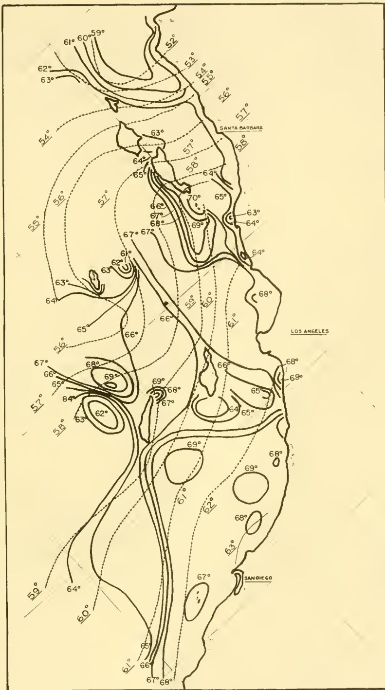
Figure 3. Surface water temperature survey with IRT; date: 8/1/63; time: 1952 -1648 P.D.S.T. Air temperature °F, dotted line. Water temperature °F, solid line .
