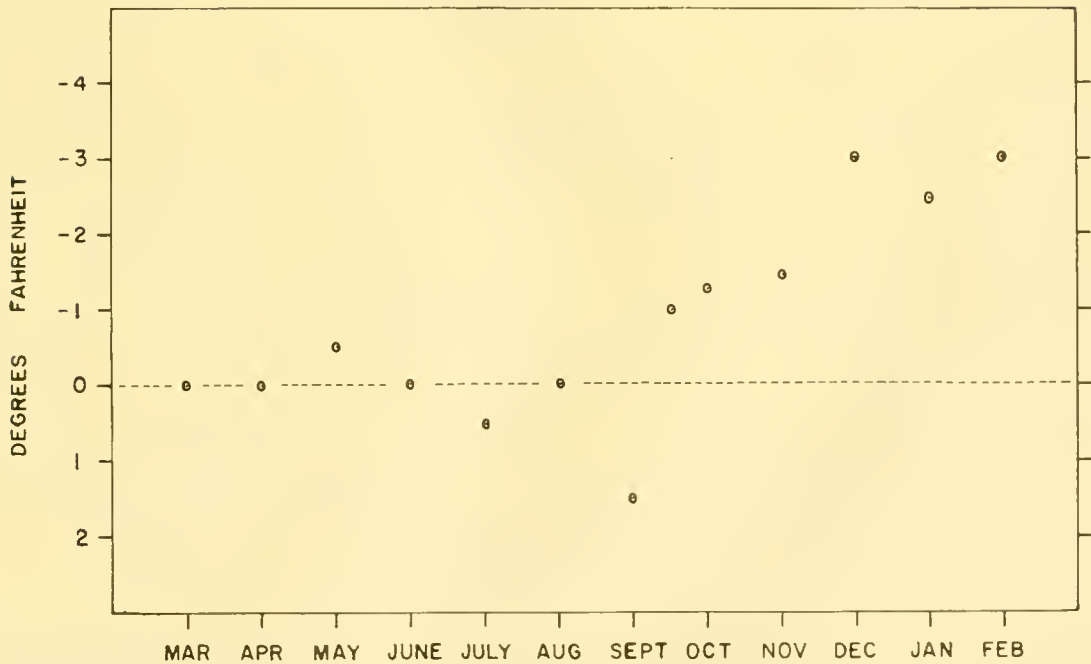
Figure 4. Differences between bucket-depth temperatures and lightship temperatures (data from Table 2)
