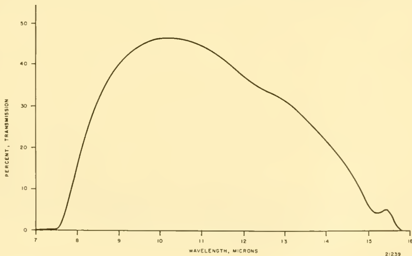
Figure 5. Spectral Passband of Barnes Infrared Thermometer, Model IT-2
