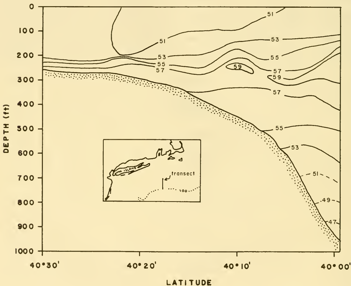
Figure 6. Temperature profile (°F.) along comparative air/sea transect (71° 07' meridian) from Albatross IV B. T. casts
