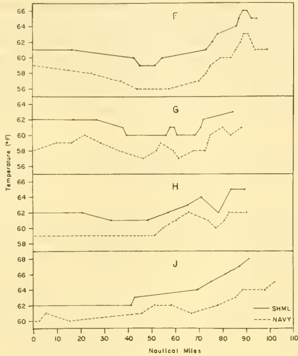
Figure 3. Temperatures from Sandy Hook - Navy comparative flight for transects F-J, October 1, 1963
