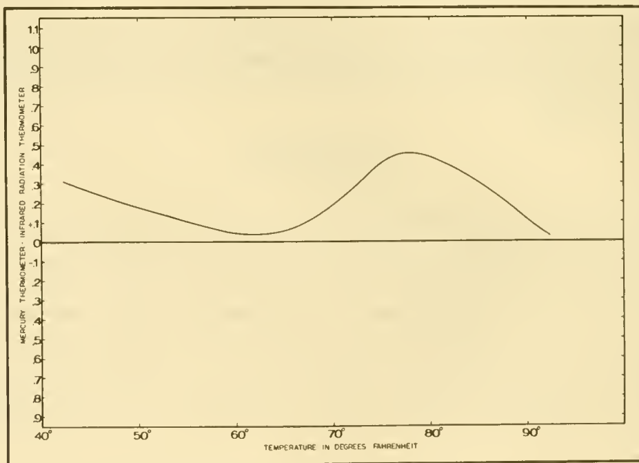
Figure 1. Results of calibration test using temperature controlled bath to determine accuracy of infrared thermometer
