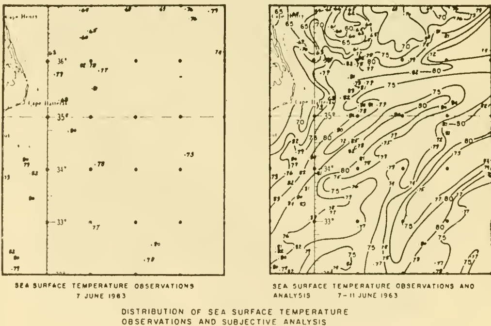
Figure 13. Example showing the ratio between daily and five-day collecting of surface reports
