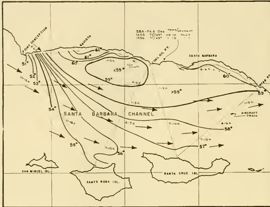
Figure 5. Wind direction and surface isotherm pattern, southern California, April 29, 1963
