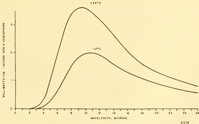
Figure 2. Blackbody Radiation (Planck's Equation)
