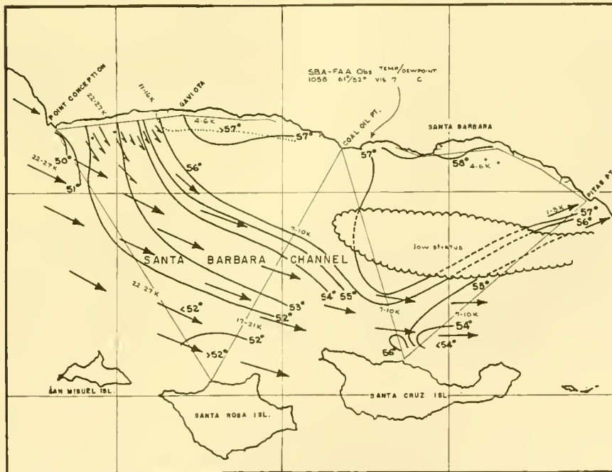
Figure 8. Wind direction and surface isotherm pattern, southern California, May 1, 1963
