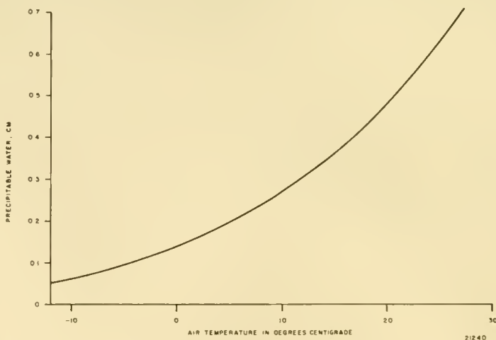
Figure 6. Precipitable Water versus Air Temperature at 1000 Feet Altitude, 100% Relative Humidity
