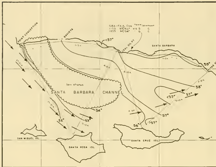
Figure 9. Wind direction and surface isotherm pattern, southern California, May 2, 1963
