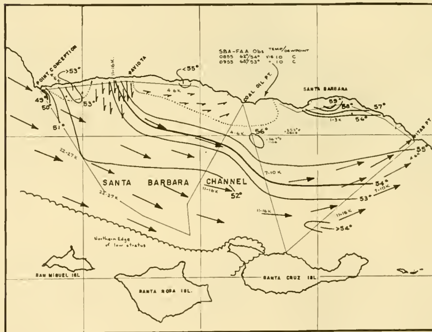
Figure 6. Wind direction and surface isotherm pattern, southern California, April 30, 1963, morning
