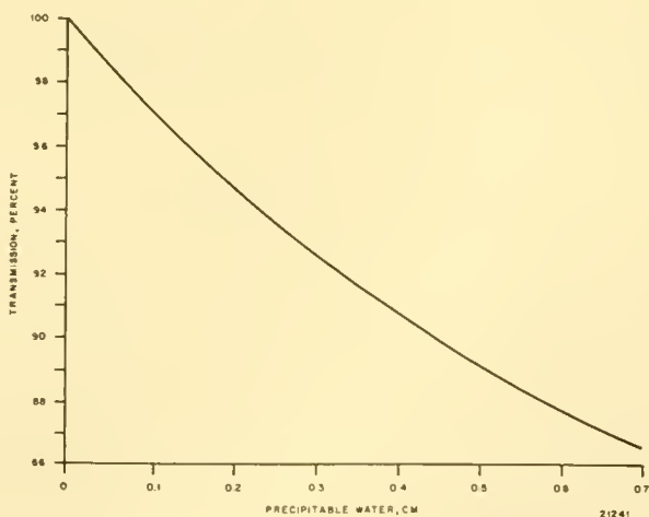
Figure 7. Average Transmission of the Atmosphere vs. Precipitable Water, 1000 Feet Path, 8-14 Microns
