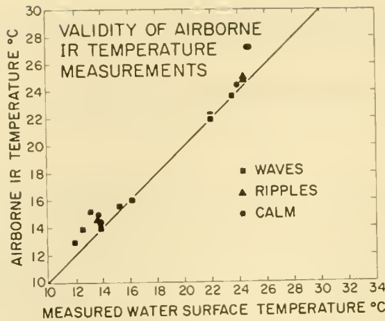
Figure 1. Validity of Airborne Infrared Temperature Measurements
