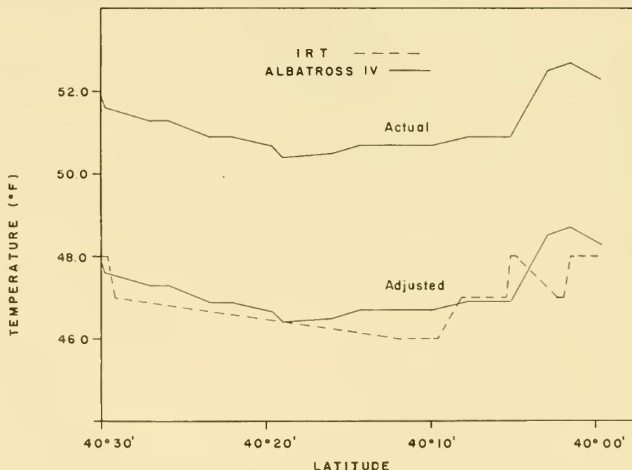
Figure 5. Surface temperature comparisons from near simultaneous records of Albatross IV and airborne IRT. Continuous recording B. T. temperatures from Albatross IV are shown as both absolute plot and superimposed on plot of IRT micro-surface readings for better comparison
