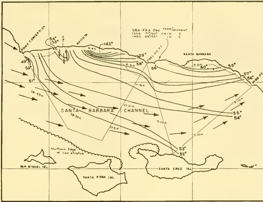
Figure 7. Wind direction and surface isotherm pattern, southern California, April 30, 1963. afternoon
