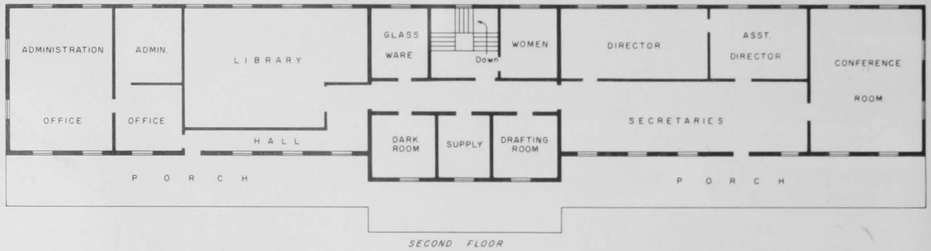
Plan of building A. This heavy masonry building is 177 feet long and 28 feet wide.
