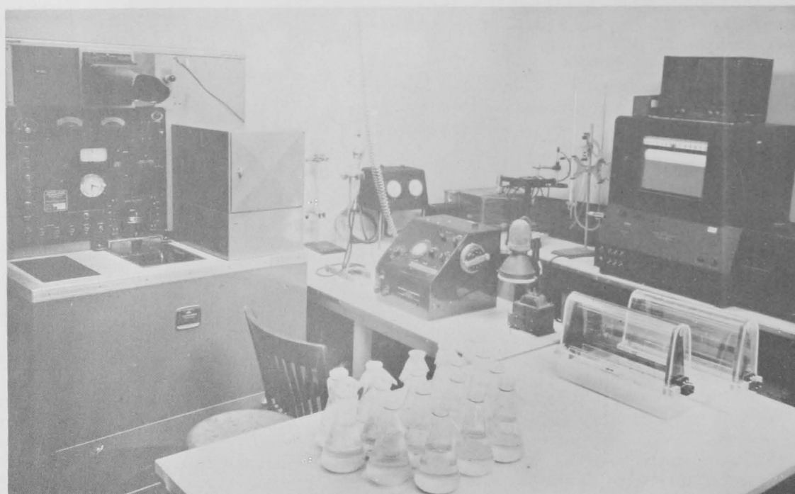
Temperature-controlled instrument room in the chemistry laboratory showing recording spectrophotometers and electrophoresis apparatus.
