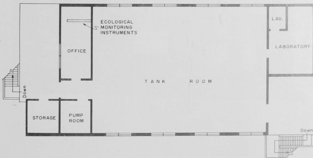
Plan of the East Lagoon field station (picture on back cover). The tank room is 40 feet wide and 56 feet long. From large concrete roof tanks, sea water flows through five plastic ceiling pipes each extending 30 feet across the width of the tank room.
