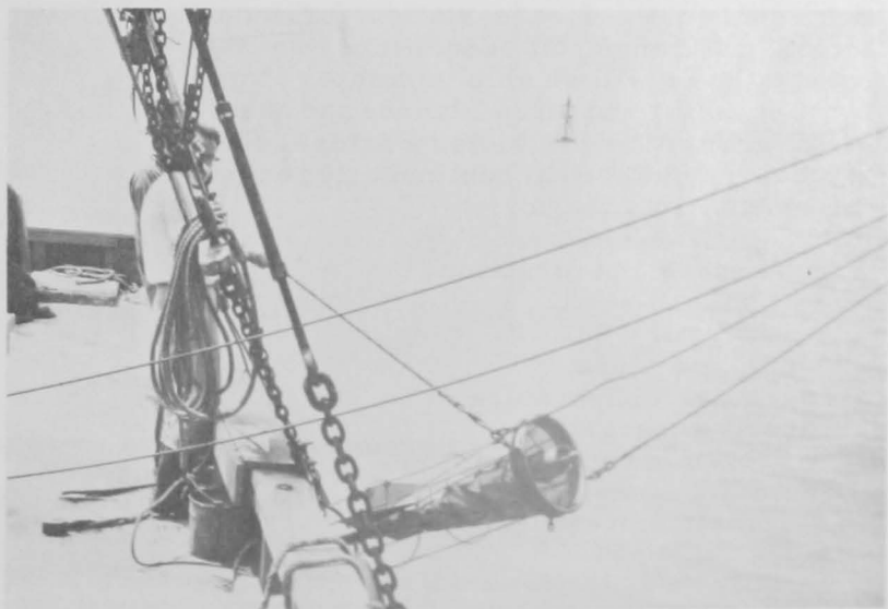
Gulf V high-speed plankton sampler. The net is fine monel metal screen.
