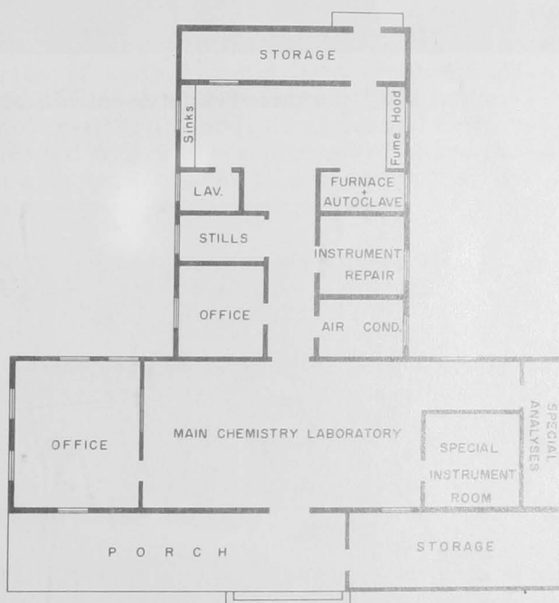
Plan of building C, the chemistry laboratory.
