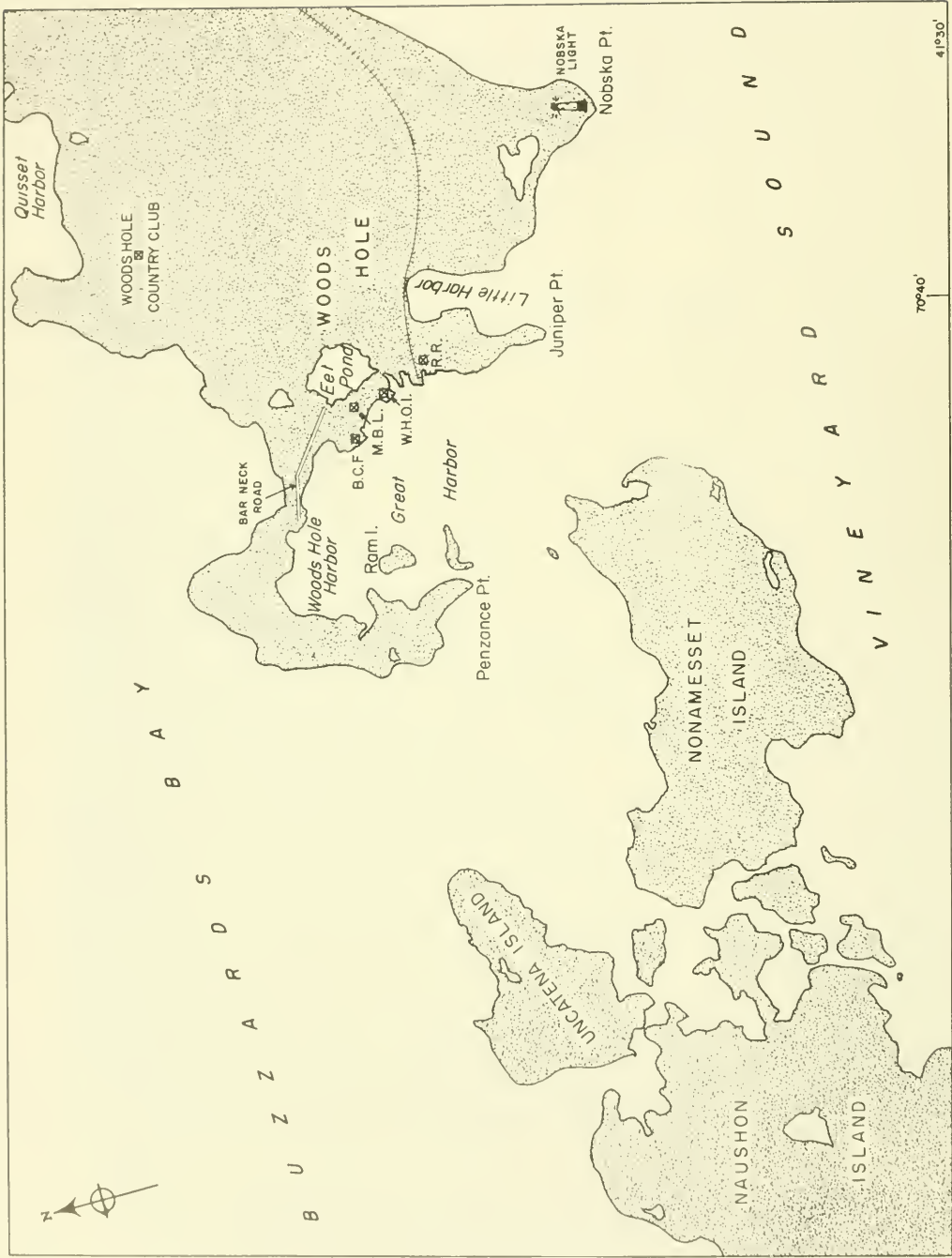
Figure 2.--Map of the present day Woods Hole area and adjacent islands.
