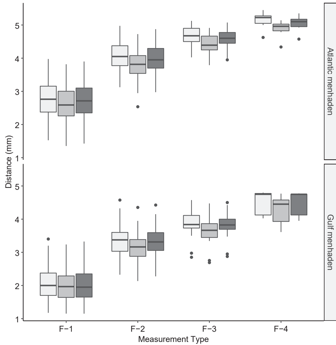
Supplementary Figure 18. Boxplot of scale distance (mm) by measurement type for the Atlantic menhaden and Gulf menhaden subsamples measured on the Eberbach projector with blue cards and then the sonic digitizer pen, and through microscope using image analysis software.
