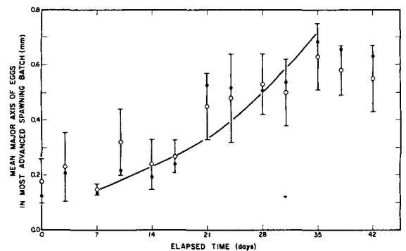
FIGURE 5.—Maturation of eggs in the most advanced spawning batch of laboratory-held northern anchovy as a function of elapsed time. Maturity is achieved when average egg size in batch attains 0.6-0.7 mm. Circles are averages of the mean size of eggs in the most advanced spawning batch of females sampled on a particular day, dots the median, and bars are \pm 2 SE. Number of eggs used to calculate the mean for each female was determined using Equation (4). The solid line is hypothetical maturation rate of egg batches from 0.15 mm (major egg axis), assuming females spawn at weekly intervals; the line is derived from data in Figure 4.
