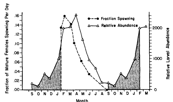
FIGURE 2.—Fraction of mature northern anchovy females from the Southern California Bight spawning per day during various months (dots). Fraction calculated from incidence of females with 24-h-old postovulatory follicles (Hunter and Goldberg 1980; Hunter and Macewicz 1980). Triangles indicate relative larval abundance per month from 1953 to 1960 (Lasker and Smith 1977). Shaded areas indicate months where spawning fraction was not estimated; total spawns per year by northern anchovy females was estimated from areas under the two curves (see text).
