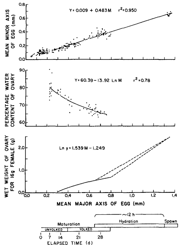
FIGURE 7.—The mean length of the minor egg axis (upper), water content of the ovary (middle), and ovary wet weight of a 16 g northern anchovy female calculated from Equation (6) (bottom), as functions of the mean major egg axis of eggs in the most advanced spawning batch (natural logarithms were used). Original data for Equation (6) (solid line, bottom) given in Hunter and Goldberg (1980); dashed lines indicate the range of egg sizes that may hydrate; and they converge at the average weight of a hydrated ovary in a 16 g female. Time scale on abscissa is based on hypothetical rate of egg maturation required for weekly spawning (see Figure 4).
